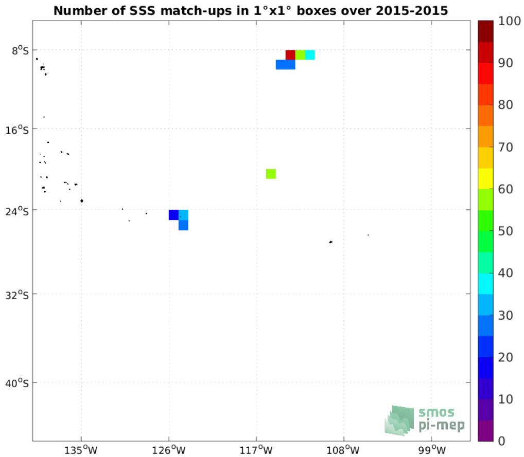
Figure 3: Number of SSS match-ups between Surface drifters SSS and the Aquarius SSS L4 OI v5 - Weekly (IPRC) SSS product for the OTT zone Pi-MEP region over 1^\circ \times 1^\circ boxes and for the full satellite product period.
