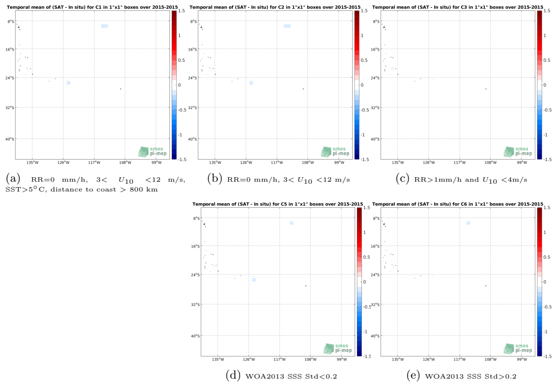
Figure 11: Temporal mean gridded over spatial boxes of size 1^\circ \times 1^\circ of \Delta SSS (Aquarius SSS L4 OI v5 - Weekly (IPRC) - Surface drifters) for 5 different subdatasets corresponding to:RR=0 mm/h, 3 < U_{10} < 12 m/s, SST >5^\circ C, distance to coast > 800 km (a), RR=0 mm/h, 3 < U_{10} < 12 m/s (b), RR >1 mm/h and U_{10} < 4 m/s (c), WOA2013 SSS Std <0.2 (d), WOA2013 SSS Std >0.2 (e).
