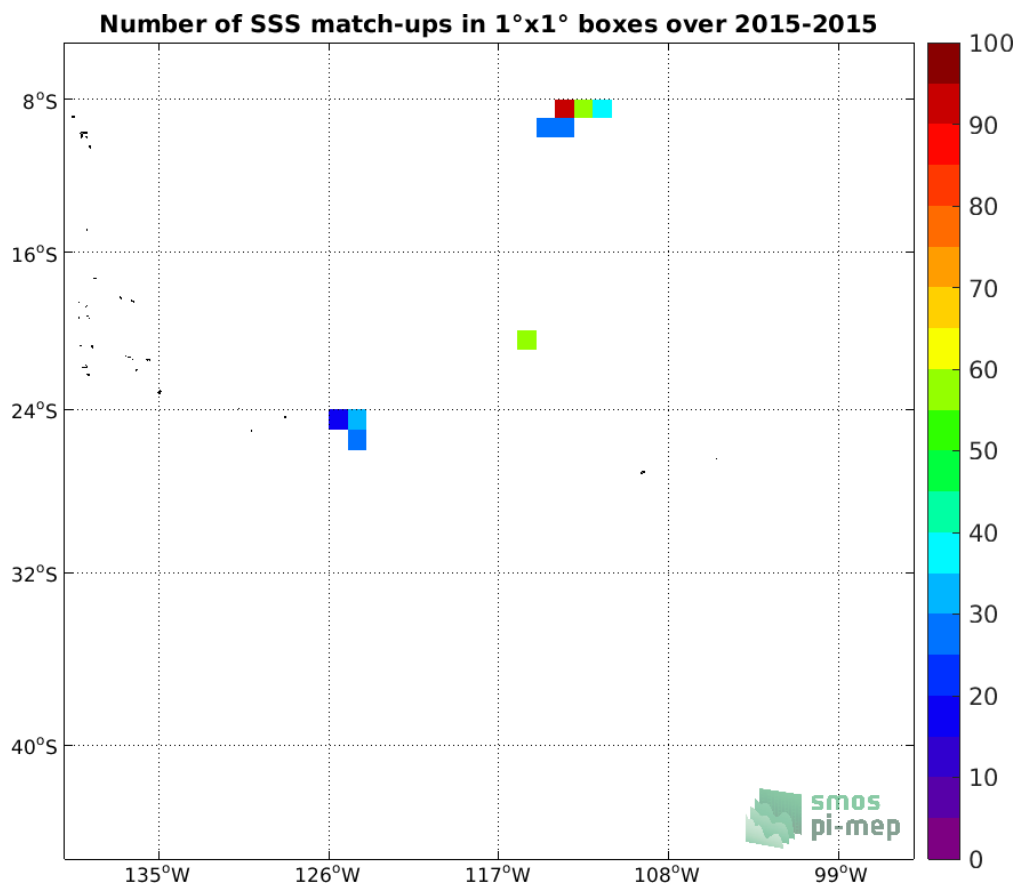
Figure 3: Number of SSS match-ups between Surface drifters SSS and the Aquarius SSS L4 OI v5 - Weekly (IPRC) SSS product for the OTT zone Pi-MEP region over 1°x1° boxes and for the full satellite product period.
