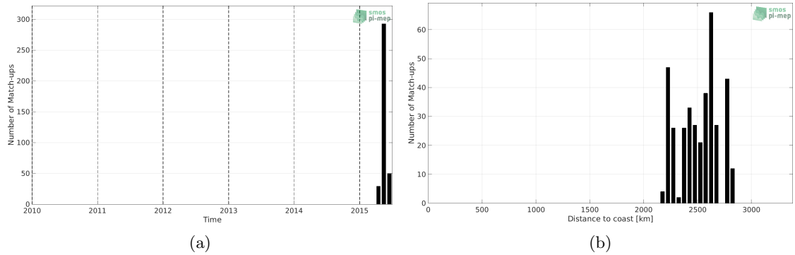
Figure 1: Number of match-ups between Surface drifters and Aquarius SSS L4 OI v5 - Weekly (IPRC) SSS as a function of time (a) and as function of the distance to coast (b) over the OTT zone Pi-MEP region and for the full satellite product period.
