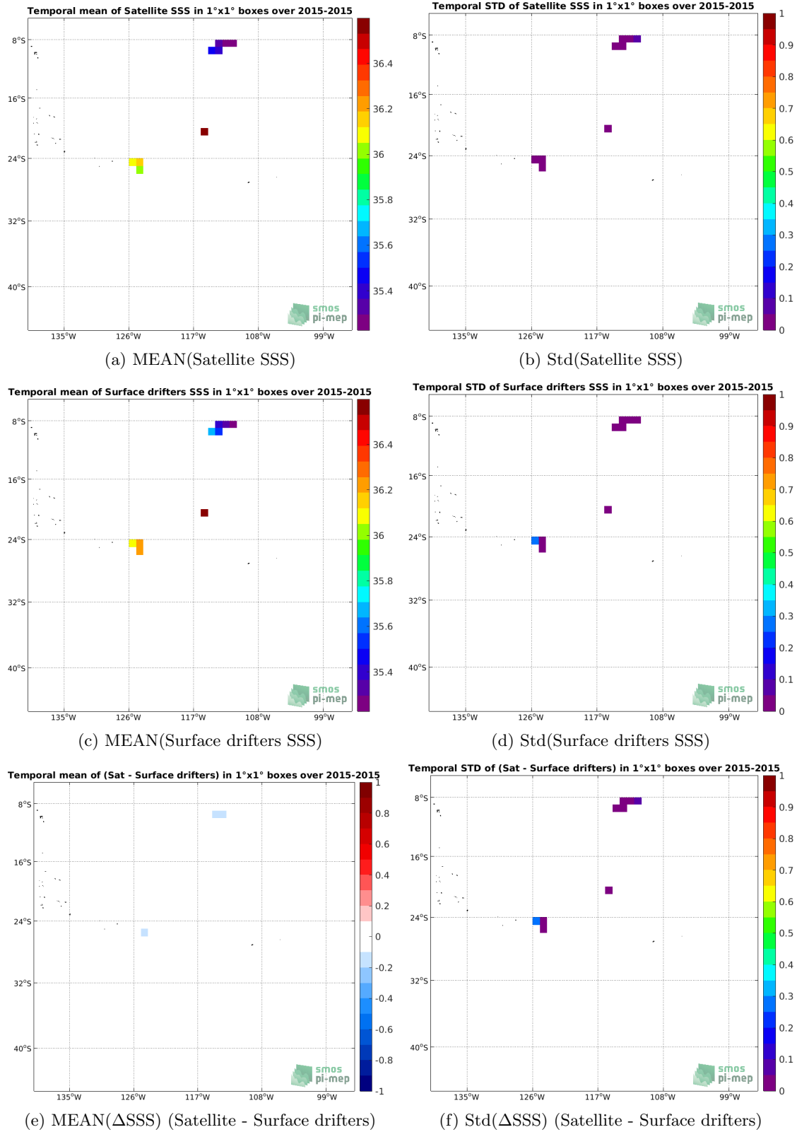
Figure 5: Temporal mean (left) and Std (right) of SSS from Aquarius SSS L4 OI v5 - Weekly (IPRC) (top), Surface drifters (middle), and of \Delta SSS (Satellite - Surface drifters). Only match-up pairs are used to generate these maps.
