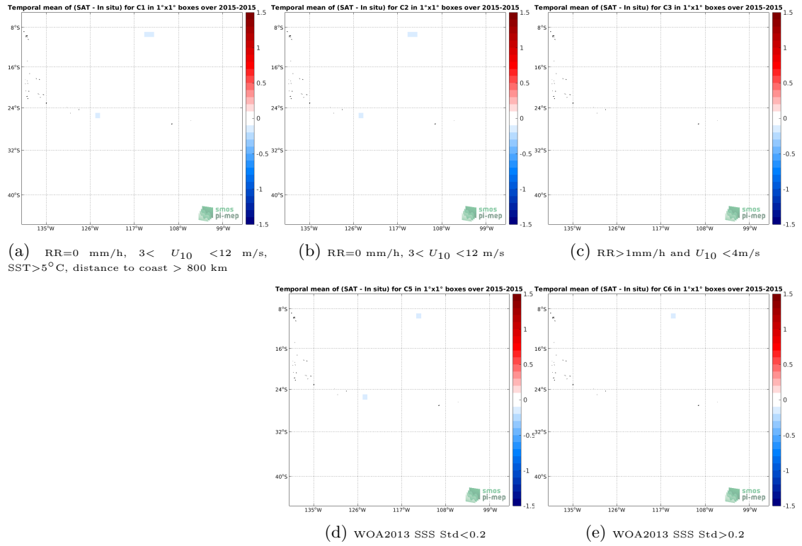
Figure 11: Temporal mean gridded over spatial boxes of size 1^\circ \times 1^\circ of \Delta SSS (Aquarius SSS L4 OI v5 - Weekly (IPRC) - Surface drifters) for 5 different subdatasets corresponding to: RR=0 mm/h, 3 < U_{10} < 12 m/s, SST > 5^\circ C , distance to coast > 800 km (a), RR=0 mm/h, 3 < U_{10} < 12 m/s (b), RR > 1 mm/h and U_{10} < 4 m/s (c), WOA2013 SSS Std < 0.2 (d), WOA2013 SSS Std > 0.2 (e).
