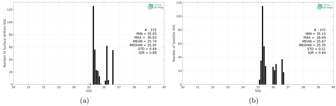
Figure 2: Histograms of SSS from Surface drifters (a) and Aquarius SSS L4 OI v5 - Weekly (IPRC) (b) considering all match-up pairs per bins of 0.1 over the OTT zone Pi-MEP region and for the full satellite product period.
