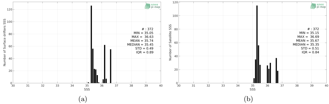
Figure 2: Histograms of SSS from Surface drifters (a) and Aquarius-L4-IPRC-V5-WEEKLY (b) considering all match-up pairs per bins of 0.1 over the OTT zone Pi-MEP region and for the full satellite product period.
