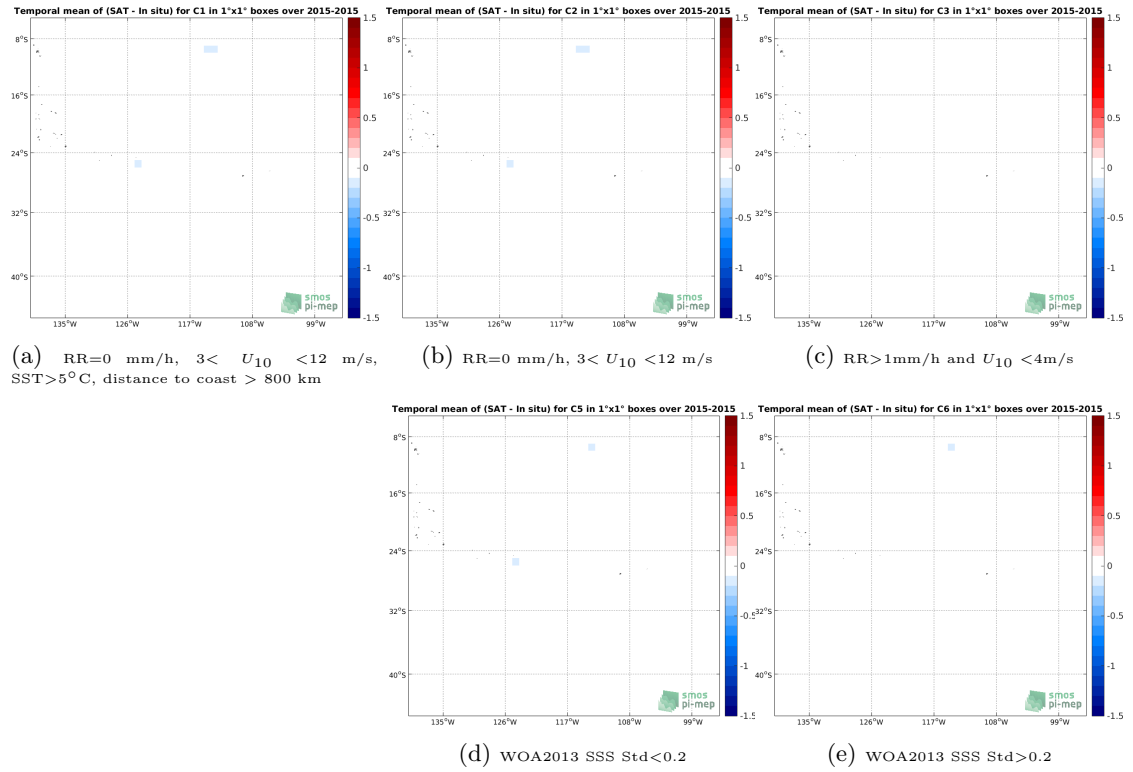
Figure 11: Temporal mean gridded over spatial boxes of size 1^\circ \times 1^\circ of \Delta SSS (Aquarius-L4-IPRC-V5-WEEKLY - Surface drifters) for 5 different subdatasets corresponding to: RR=0 mm/h, 3 < U_{10} < 12 m/s, SST >5^\circ C, distance to coast > 800 km (a), RR=0 mm/h, 3 < U_{10} < 12 m/s (b), RR >1 mm/h and U_{10} < 4 m/s (c), WOA2013 SSS Std <0.2 (d), WOA2013 SSS Std >0.2 (e).
