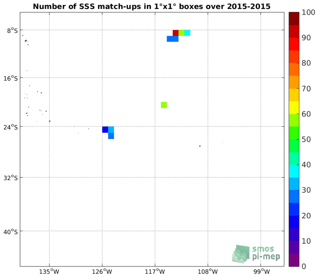
Figure 3: Number of SSS match-ups between Surface drifters SSS and the Aquarius-L4-IPRC-V5-WEEKLY SSS product for the OTT zone Pi-MEP region over 1°x1° boxes and for the full satellite product period.
