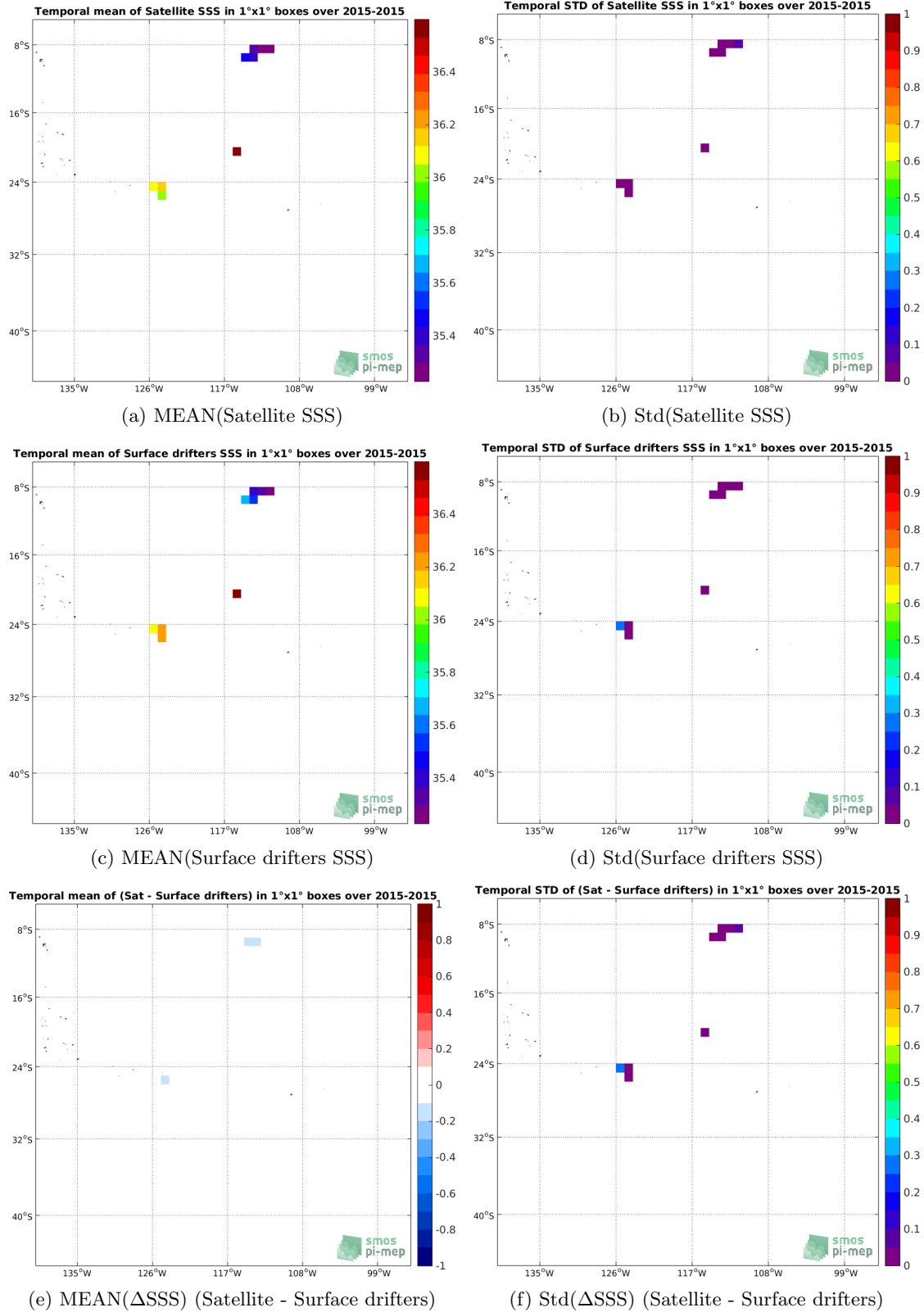
Figure 5: Temporal mean (left) and Std (right) of SSS from Aquarius-L4-IPRC-V5-WEEKLY (top), Surface drifters (middle), and of \Delta SSS (Satellite - Surface drifters). Only match-up pairs are used to generate these maps.
