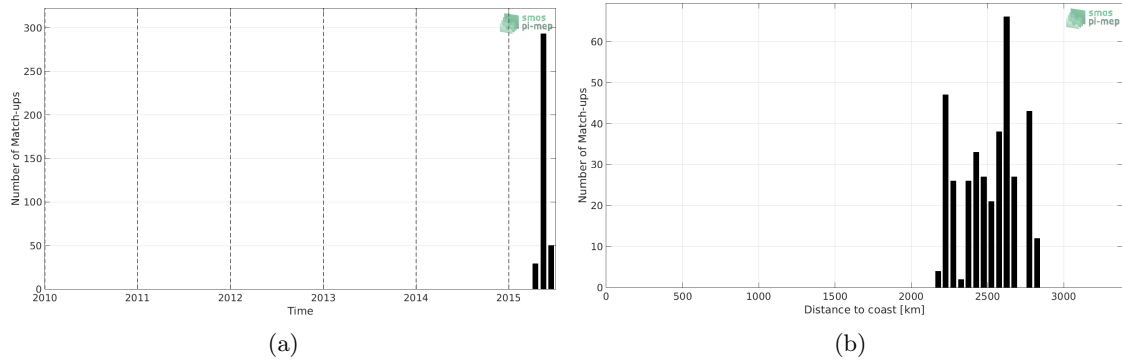
Figure 1: Number of match-ups between Surface drifters and Aquarius-L4-IPRC-V5-WEEKLY SSS as a function of time (a) and as function of the distance to coast (b) over the OTT zone Pi-MEP region and for the full satellite product period.
