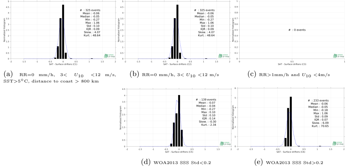
Figure 12: Normalized histogram of \Delta SSS (Aquarius-L4-IPRC-V5-WEEKLY - Surface drifters) for 5 different subdatasets corresponding to: RR=0 mm/h, 3 < U_{10} < 12 m/s, SST>5°C, distance to coast > 800 km (a), RR=0 mm/h, 3 < U_{10} < 12 m/s (b), RR>1mm/h and U_{10} < 4 m/s (c), WOA2013 SSS Std<0.2 (d), WOA2013 SSS Std>0.2 (e).
