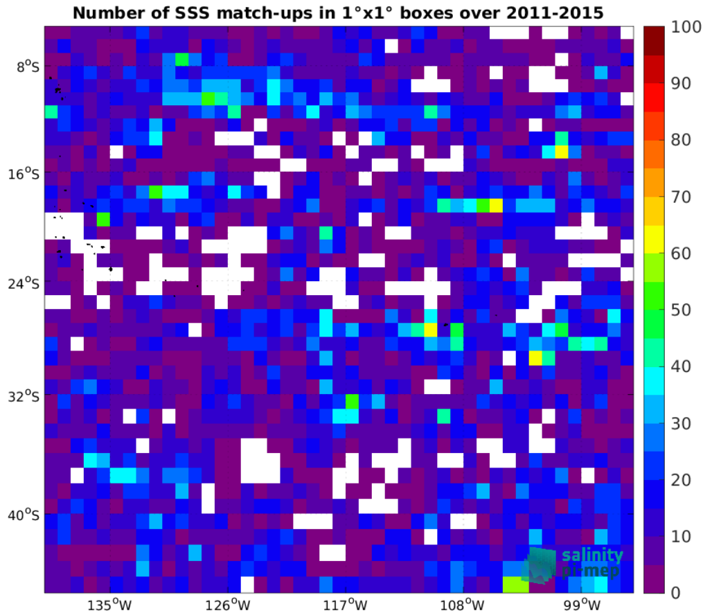
Figure 5: Number of SSS match-ups between Argo SSS and the Aquarius SSS L4 OI v5 - Weekly (IPRC) SSS product for the OTT zone Pi-MEP region over 1^\circ \times 1^\circ boxes and for the full satellite product period.
