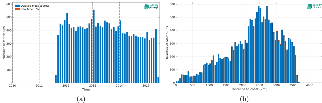
Figure 2: Number of match-ups between Argo and Aquarius SSS L4 OI v5 - Weekly (IPRC) SSS as a function of time (a) and as function of the distance to coast (b) over the OTT zone Pi-MEP region and for the full satellite product period.
