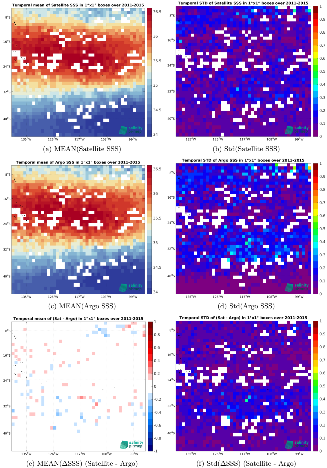
Figure 7: Temporal mean (left) and Std (right) of SSS from Aquarius SSS L4 OI v5 - Weekly (IPRC) (top), Argo (middle), and of \Delta SSS (Satellite - Argo). Only match-up pairs are used to generate these maps.
