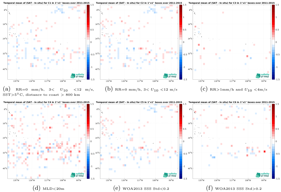
Figure 14: Temporal mean gridded over spatial boxes of size 1^\circ \times 1^\circ of \Delta SSS (Aquarius SSS L4 OI v5 - Weekly (IPRC) - Argo) for 6 different subdatasets corresponding to:RR=0 mm/h, 3 < U_{10} < 12 m/s, SST >5^\circ C, distance to coast > 800 km (a), RR=0 mm/h, 3 < U_{10} < 12 m/s (b), RR >1 mm/h and U_{10} < 4 m/s (c),MLD <20 m (d),WOA2013 SSS Std <0.2 (e),WOA2013 SSS Std >0.2 (f).
