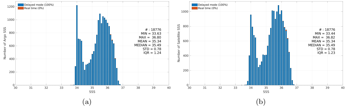
Figure 3: Histograms of SSS from Argo (a) and Aquarius SSS L4 OI v5 - Weekly (IPRC) (b) considering all match-up pairs per bins of 0.1 over the OTT zone Pi-MEP region and for the full satellite product period.
