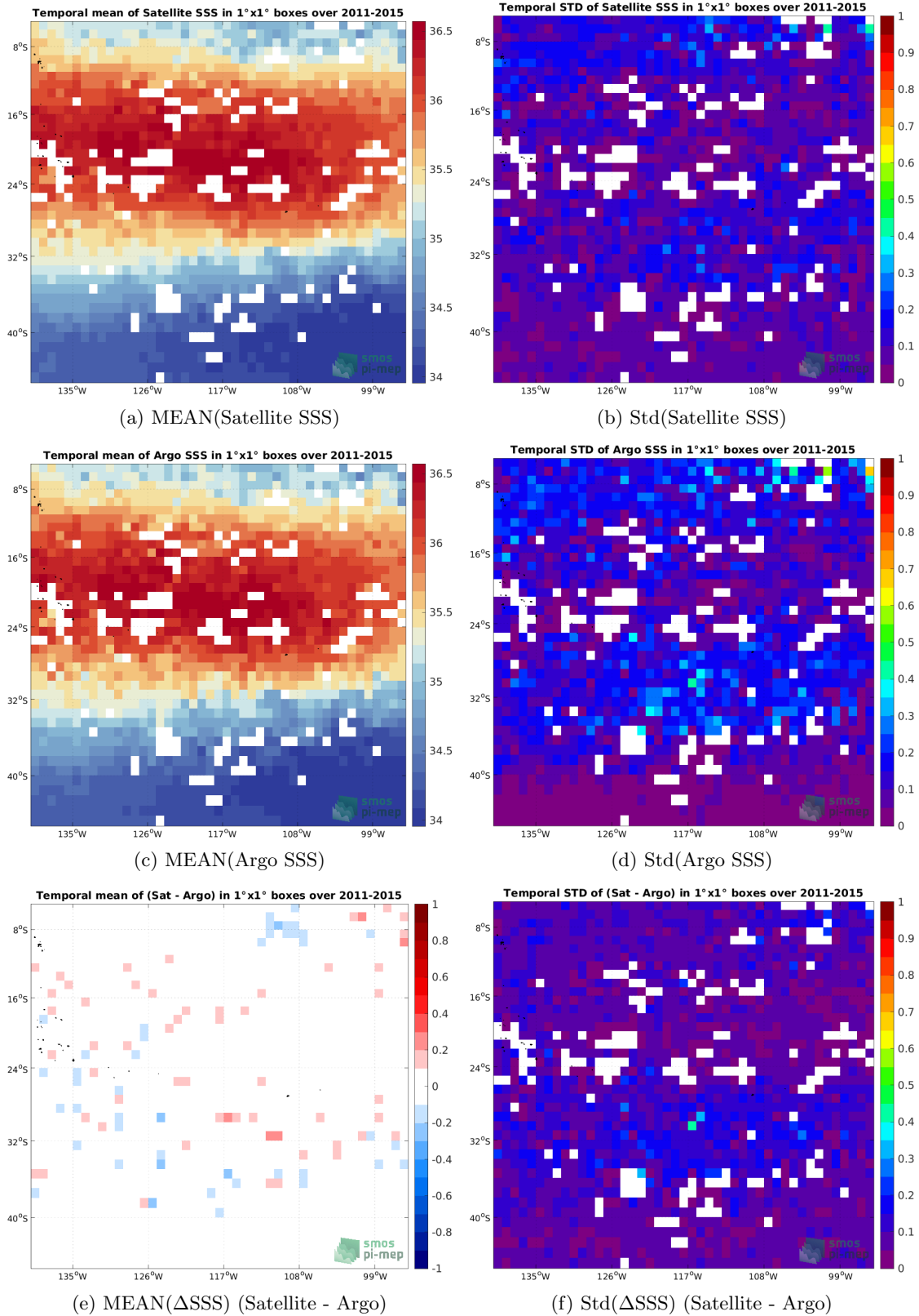
Figure 6: Temporal mean (left) and Std (right) of SSS from Aquarius SSS L4 OI v5 - Weekly (IPRC) (top), Argo (middle), and of \Delta SSS (Satellite - Argo). Only match-up pairs are used to generate these maps.
