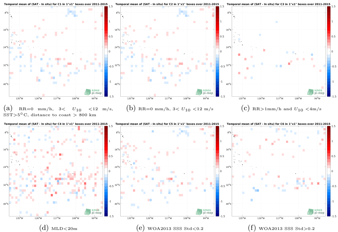
Figure 12: Temporal mean gridded over spatial boxes of size 1^\circ \times 1^\circ of \Delta SSS (Aquarius SSS L4 OI v5 - Weekly (IPRC) - Argo) for 6 different subdatasets corresponding to:RR=0 mm/h, 3 < U_{10} < 12 m/s, SST > 5^\circ\text{C} , distance to coast > 800 km (a), RR=0 mm/h, 3 < U_{10} < 12 m/s (b), RR > 1 mm/h and U_{10} < 4 m/s (c),MLD < 20 m (d),WOA2013 SSS Std < 0.2 (e),WOA2013 SSS Std > 0.2 (f).
