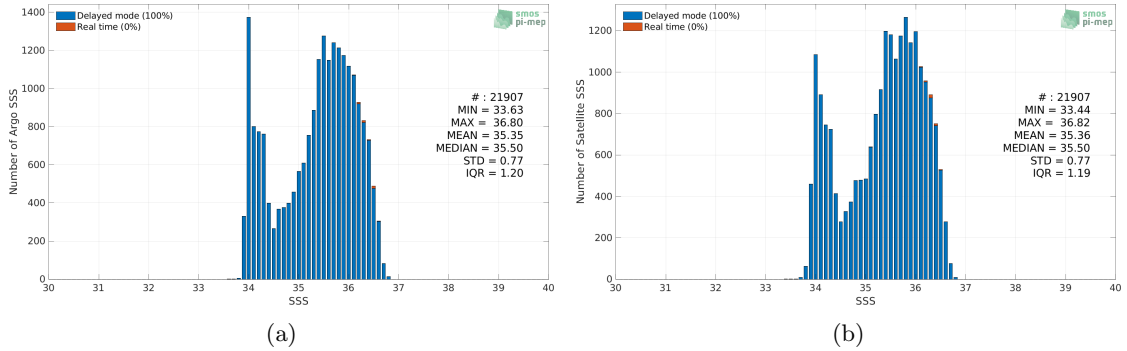
Figure 2: Histograms of SSS from Argo (a) and Aquarius SSS L4 OI v5 - Weekly (IPRC) (b) considering all match-up pairs per bins of 0.1 over the OTT zone Pi-MEP region and for the full satellite product period.
