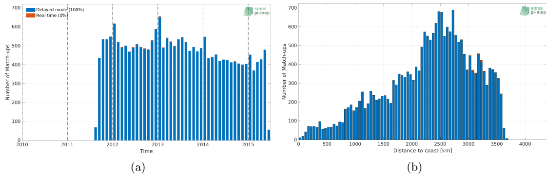
Figure 1: Number of match-ups between Argo and Aquarius SSS L4 OI v5 - Weekly (IPRC) SSS as a function of time (a) and as function of the distance to coast (b) over the OTT zone Pi-MEP region and for the full satellite product period.
