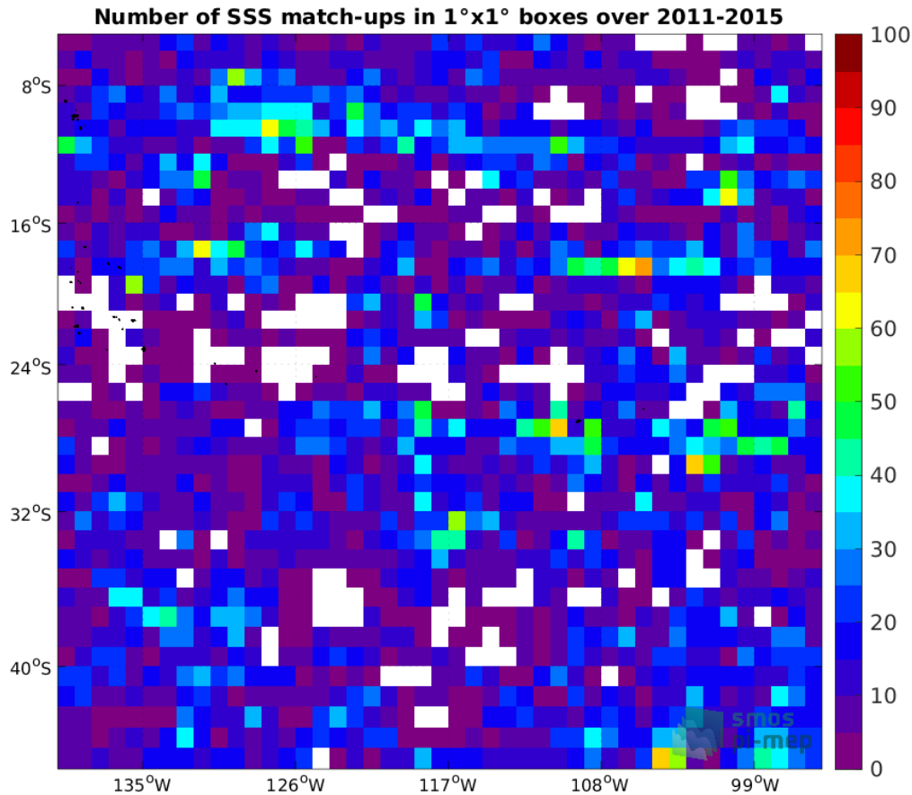
Figure 4: Number of SSS match-ups between Argo SSS and the Aquarius SSS L4 OI v5 - Weekly (IPRC) SSS product for the OTT zone Pi-MEP region over 1^\circ \times 1^\circ boxes and for the full satellite product period.
