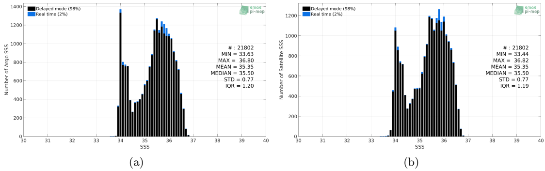
Figure 2: Histograms of SSS from Argo (a) and Aquarius-L4-IPRC-V5-WEEKLY (b) considering all match-up pairs per bins of 0.1 over the OTT zone Pi-MEP region and for the full satellite product period.
