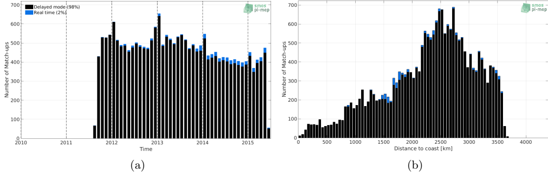
Figure 1: Number of match-ups between Argo and Aquarius-L4-IPRC-V5-WEEKLY SSS as a function of time (a) and as function of the distance to coast (b) over the OTT zone Pi-MEP region and for the full satellite product period.
