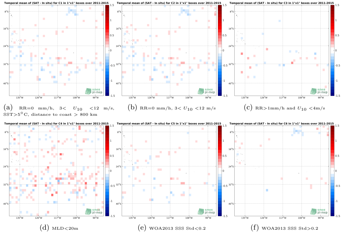
Figure 12: Temporal mean gridded over spatial boxes of size 1^\circ \times 1^\circ of \Delta SSS (Aquarius-L4-IPRC-V5-WEEKLY - Argo) for 6 different subdatasets corresponding to: RR=0 mm/h, 3 < U_{10} < 12 m/s, SST >5^\circ C, distance to coast > 800 km (a), RR=0 mm/h, 3 < U_{10} < 12 m/s (b), RR >1 mm/h and U_{10} < 4 m/s (c),MLD <20 m (d),WOA2013 SSS Std <0.2 (e),WOA2013 SSS Std >0.2 (f).
