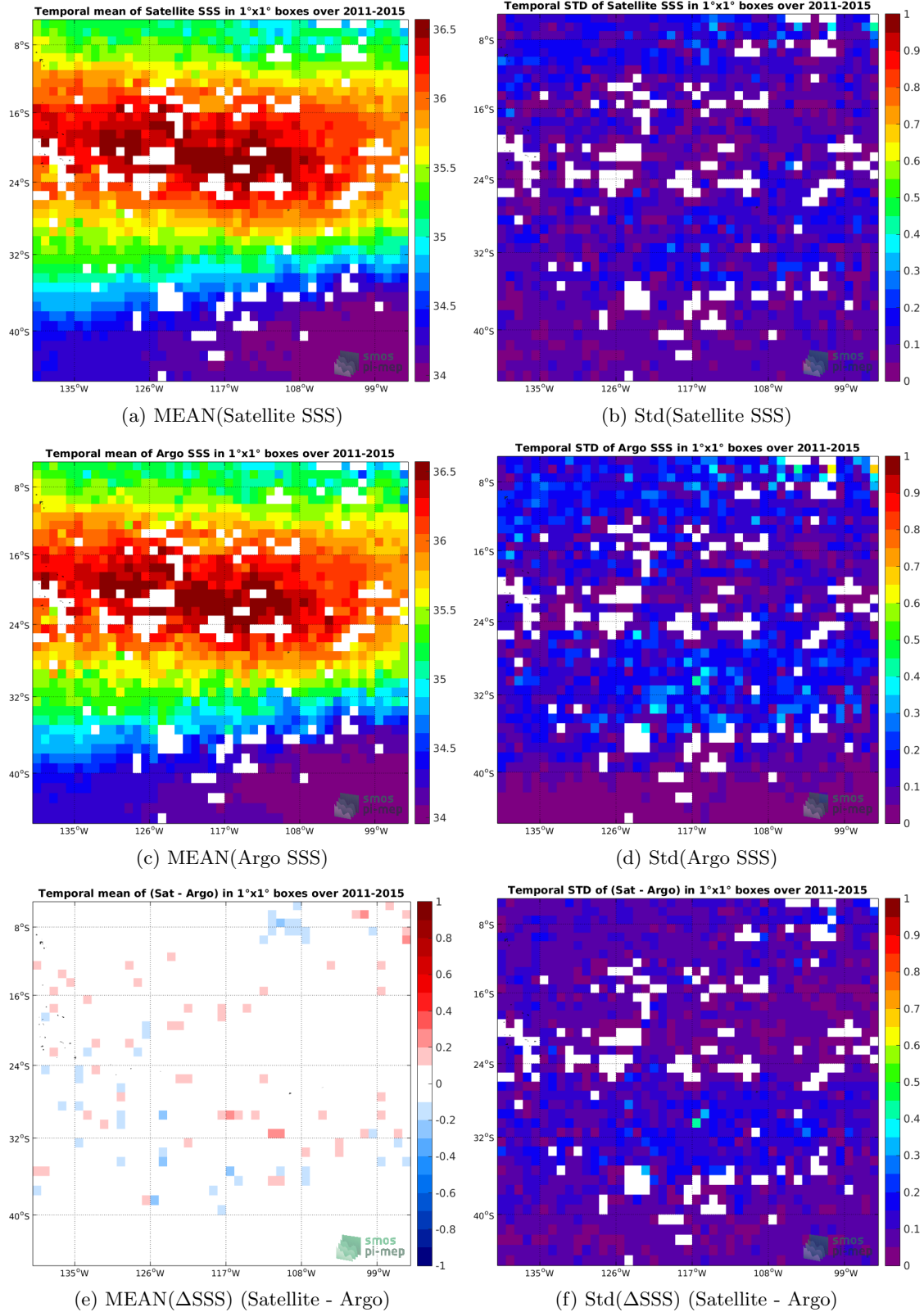
Figure 6: Temporal mean (left) and Std (right) of SSS from Aquarius-L4-IPRC-V5-WEEKLY (top), Argo (middle), and of \Delta SSS (Satellite - Argo). Only match-up pairs are used to generate these maps.
