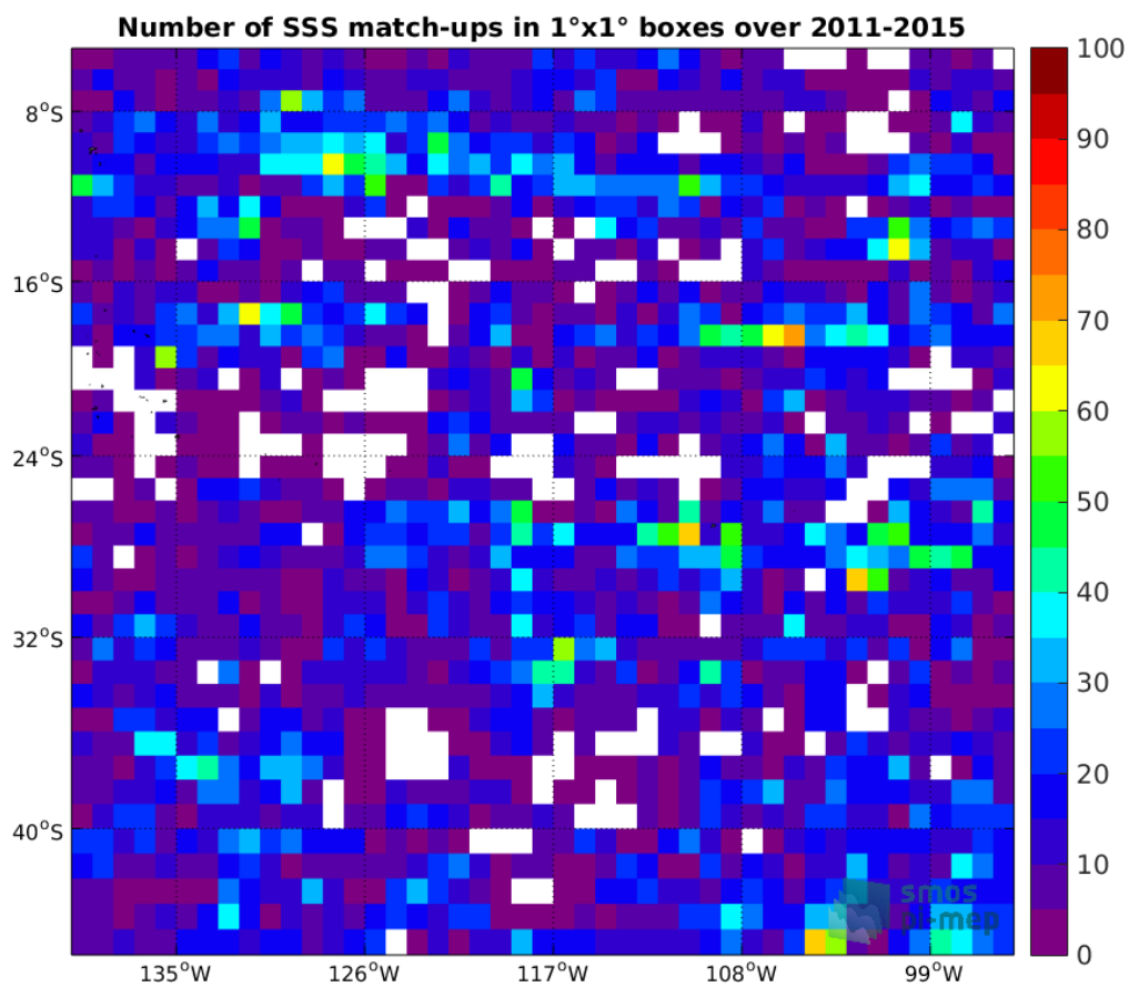
Figure 4: Number of SSS match-ups between Argo SSS and the Aquarius-L4-IPRC-V5-WEEKLY SSS product for the OTT zone Pi-MEP region over 1°x1° boxes and for the full satellite product period.
