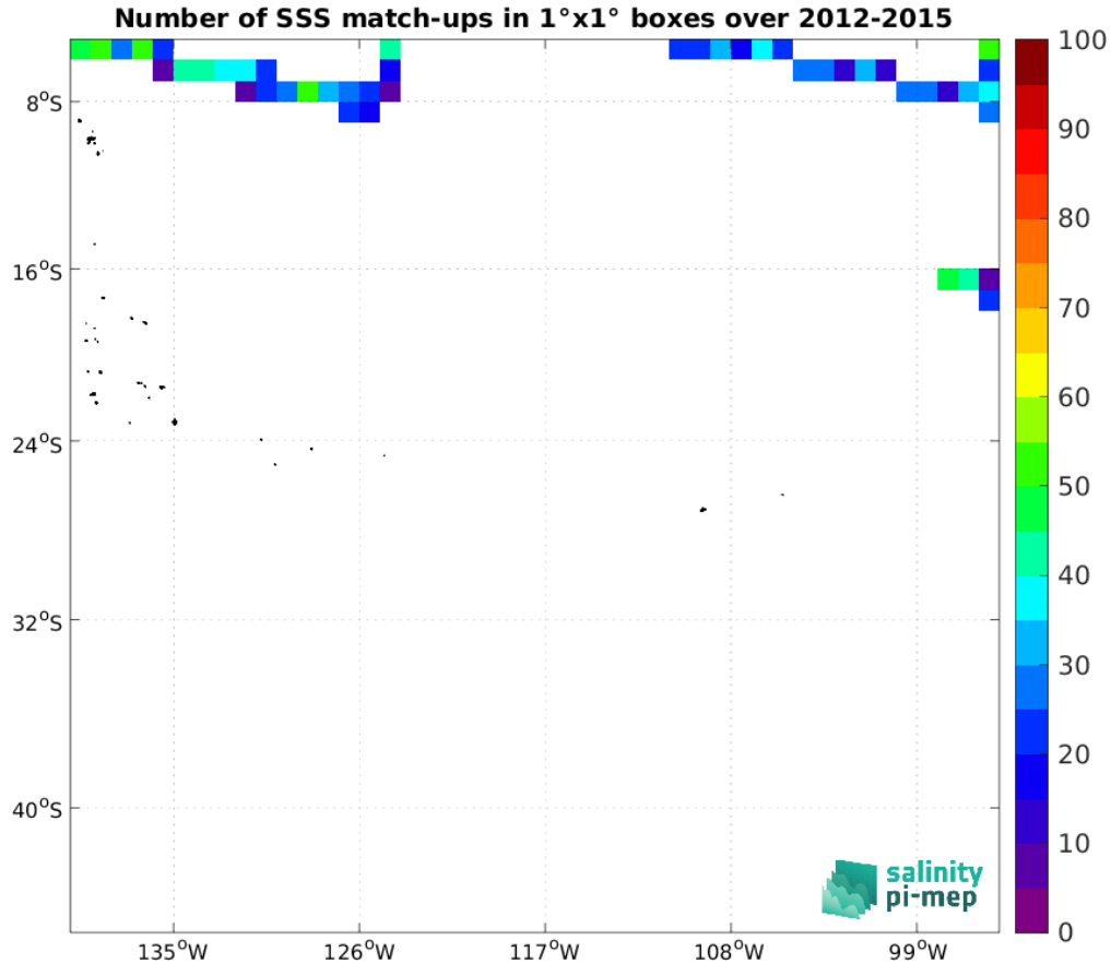
Figure 5: Number of SSS match-ups between TSG (SAMOS) SSS and the Aquarius SSS L4 OI v5 - Monthly (IPRC) SSS product for the OTT zone Pi-MEP region over 1^\circ \times 1^\circ boxes and for the full satellite product period.
