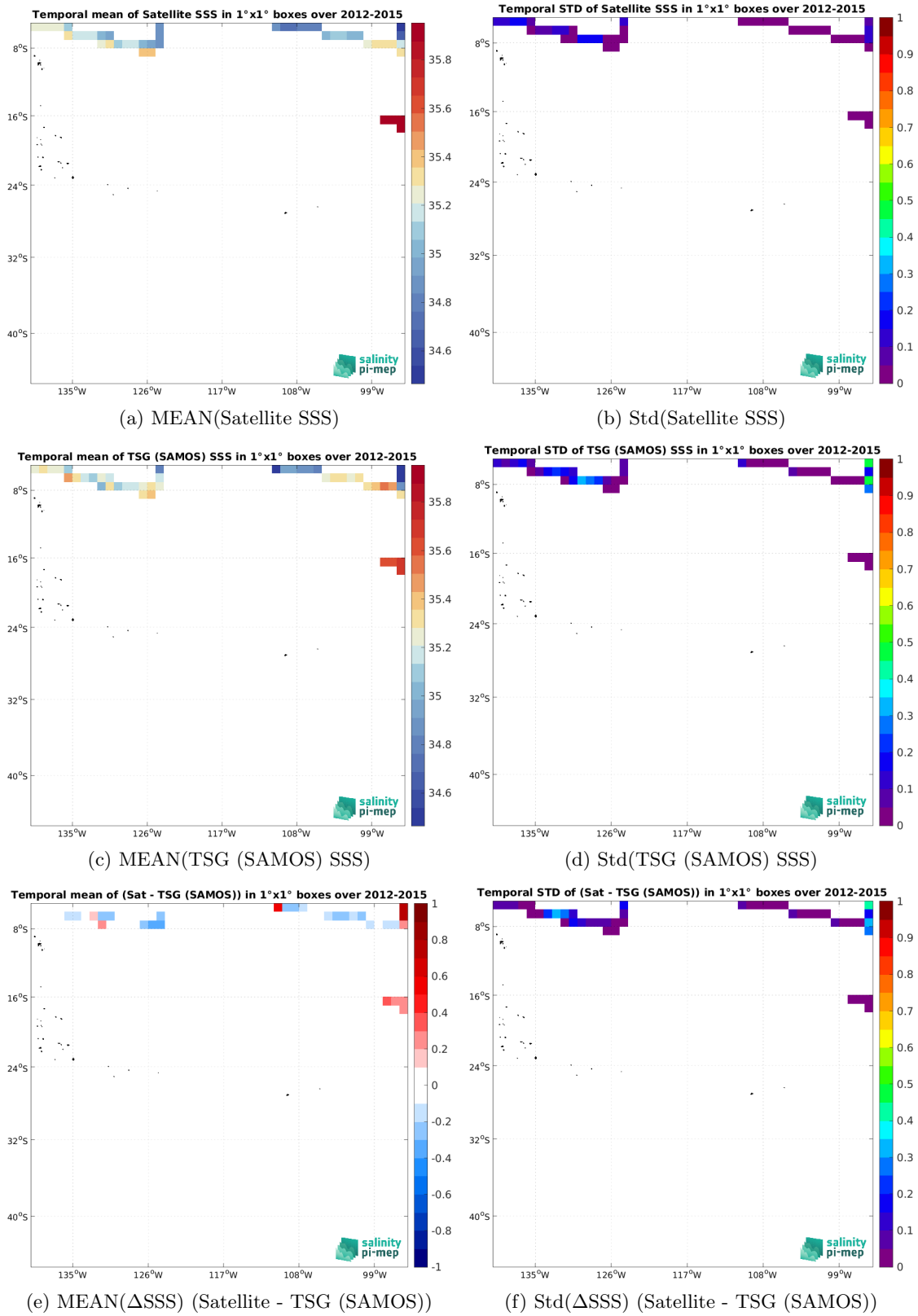
Figure 7: Temporal mean (left) and Std (right) of SSS from Aquarius SSS L4 OI v5 - Monthly (IPRC) (top), TSG (SAMOS) (middle), and of \Delta SSS (Satellite - TSG (SAMOS)). Only match-up pairs are used to generate these maps.
