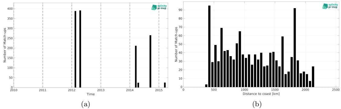
Figure 2: Number of match-ups between TSG (SAMOS) and Aquarius SSS L4 OI v5 - Monthly (IPRC) SSS as a function of time (a) and as function of the distance to coast (b) over the OTT zone Pi-MEP region and for the full satellite product period.
