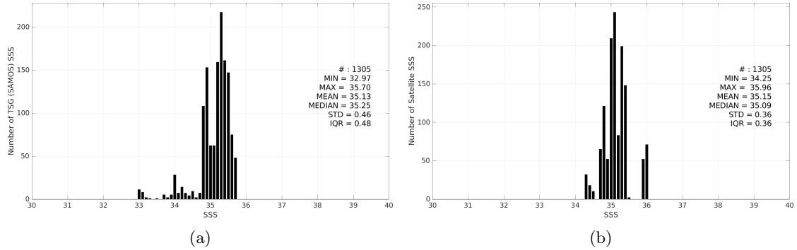
Figure 3: Histograms of SSS from TSG (SAMOS) (a) and Aquarius SSS L4 OI v5 - Monthly (IPRC) (b) considering all match-up pairs per bins of 0.1 over the OTT zone Pi-MEP region and for the full satellite product period.
