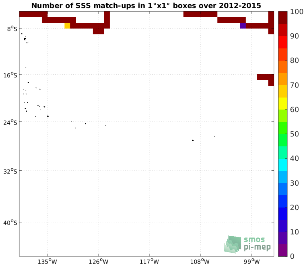
Figure 4: Number of SSS match-ups between TSG (SAMOS) SSS and the Aquarius SSS L4 OI v5 - Monthly (IPRC) SSS product for the OTT zone Pi-MEP region over 1^\circ \times 1^\circ boxes and for the full satellite product period.
