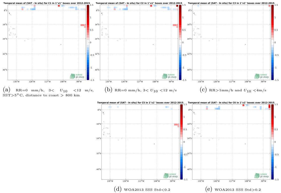
Figure 12: Temporal mean gridded over spatial boxes of size 1^\circ \times 1^\circ of \Delta\text{SSS} (Aquarius SSS L4 OI v5 - Monthly (IPRC) - TSG (SAMOS)) for 5 different subdatasets corresponding to:RR=0 mm/h, 3 < U_{10} < 12 m/s, SST >5^\circ\text{C} , distance to coast > 800 km (a), RR=0 mm/h, 3 < U_{10} < 12 m/s (b), RR >1 mm/h and U_{10} < 4 m/s (c), WOA2013 SSS Std <0.2 (d), WOA2013 SSS Std >0.2 (e).
