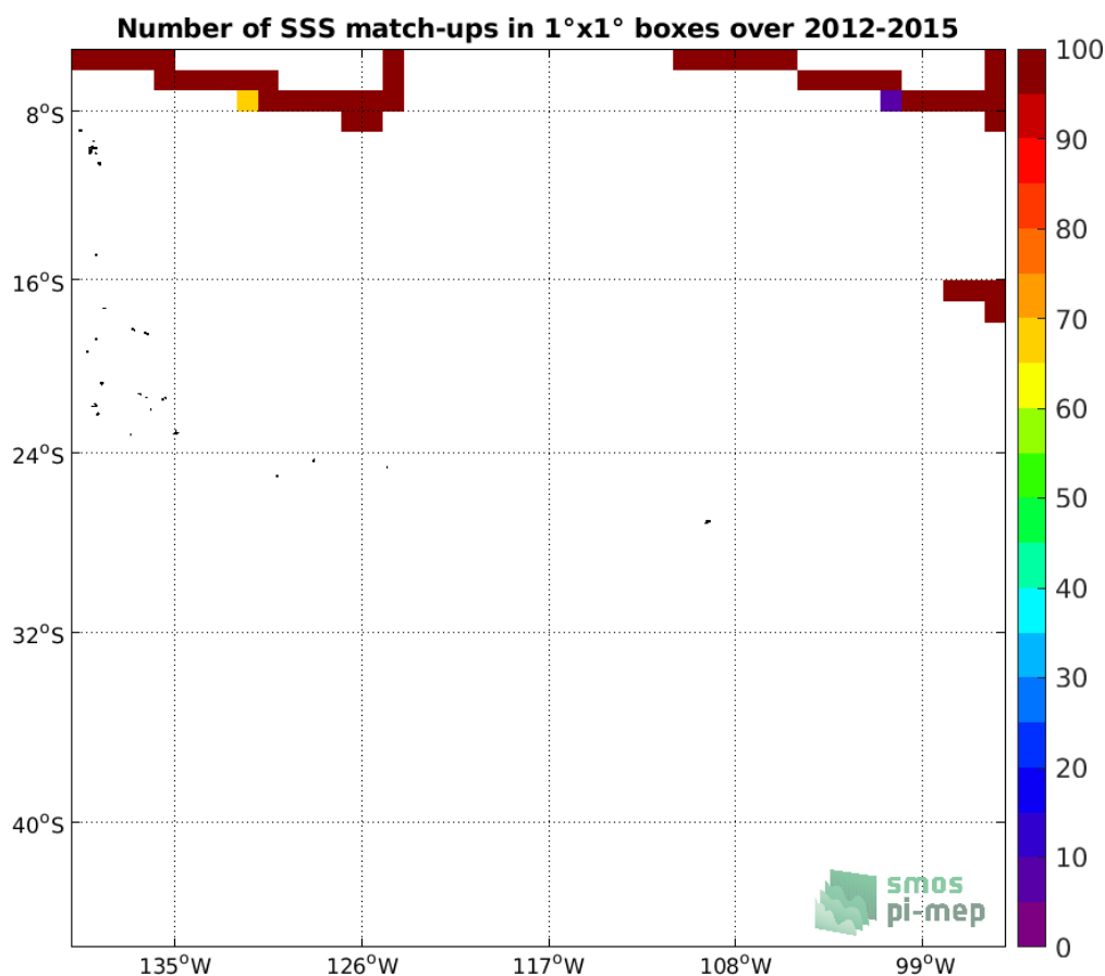
Figure 4: Number of SSS match-ups between TSG (SAMOS) SSS and the Aquarius SSS L4 OI v5 - Monthly (IPRC) SSS product for the OTT zone Pi-MEP region over 1°×1° boxes and for the full satellite product period.
