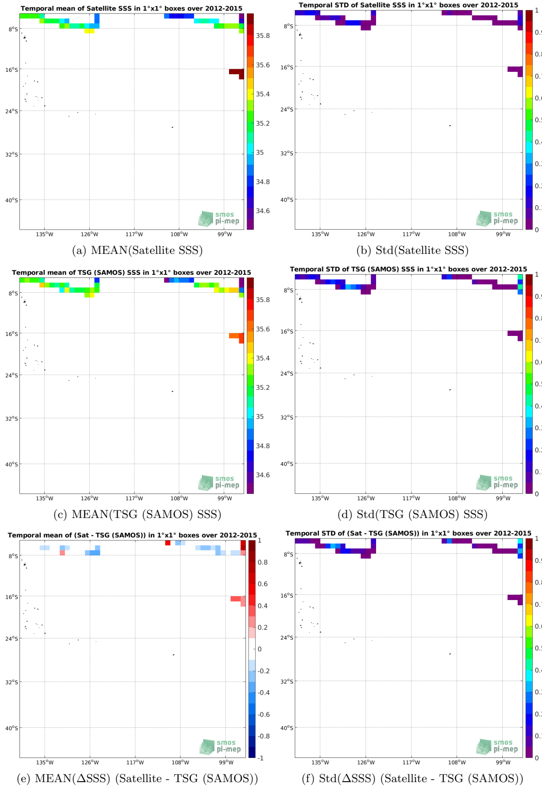
(a) MEAN(Satellite SSS) (b) Std(Satellite SSS) (c) MEAN(TSG (SAMOS) SSS) (d) Std(TSG (SAMOS) SSS) (e) MEAN( \Delta SSS) (Satellite - TSG (SAMOS)) (f) Std( \Delta SSS) (Satellite - TSG (SAMOS)) Figure 6: Temporal mean (left) and Std (right) of SSS from Aquarius SSS L4 OI v5 - Monthly (IPRC) (top), TSG (SAMOS) (middle), and of \Delta SSS (Satellite - TSG (SAMOS)). Only match-up pairs are used to generate these maps.
