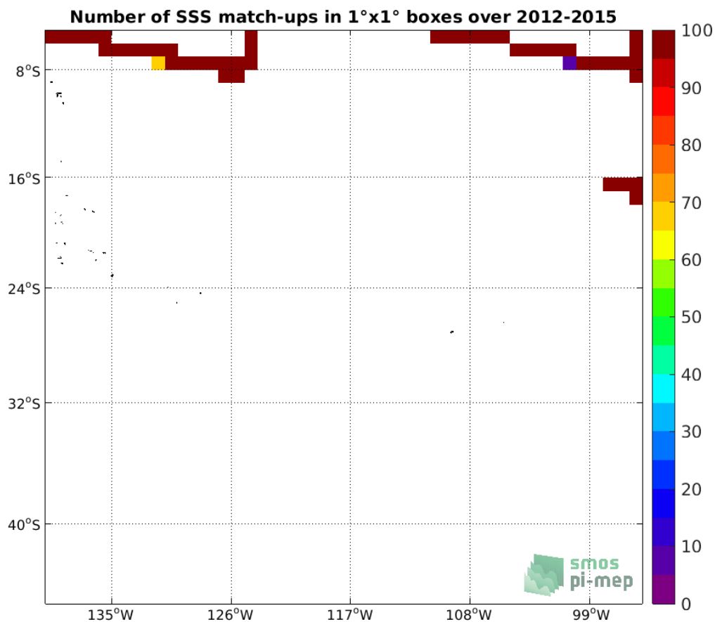
Figure 4: Number of SSS match-ups between TSG (SAMOS) SSS and the Aquarius SSS L4 OI v5 - Monthly (IPRC) SSS product for the OTT zone Pi-MEP region over 1°x1° boxes and for the full satellite product period.
