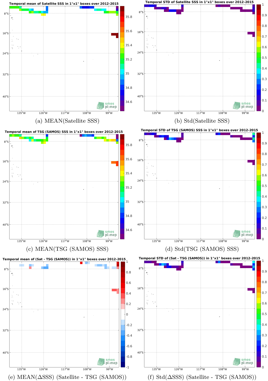
Figure 6: Temporal mean (left) and Std (right) of SSS from Aquarius SSS L4 OI v5 - Monthly (IPRC) (top), TSG (SAMOS) (middle), and of \Delta SSS (Satellite - TSG (SAMOS)). Only match-up pairs are used to generate these maps.
