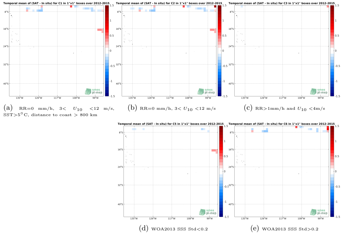
Figure 12: Temporal mean gridded over spatial boxes of size 1^\circ \times 1^\circ of \Delta SSS (Aquarius SSS L4 OI v5 - Monthly (IPRC) - TSG (SAMOS)) for 5 different subdatasets corresponding to:RR=0 mm/h, 3 < U_{10} < 12 m/s, SST >5^\circ C, distance to coast > 800 km (a), RR=0 mm/h, 3 < U_{10} < 12 m/s (b), RR >1 mm/h and U_{10} < 4 m/s (c), WOA2013 SSS Std <0.2 (d), WOA2013 SSS Std >0.2 (e).
