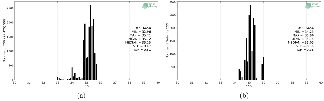
Figure 2: Histograms of SSS from TSG (SAMOS) (a) and Aquarius SSS L4 OI v5 - Monthly (IPRC) (b) considering all match-up pairs per bins of 0.1 over the OTT zone Pi-MEP region and for the full satellite product period.
