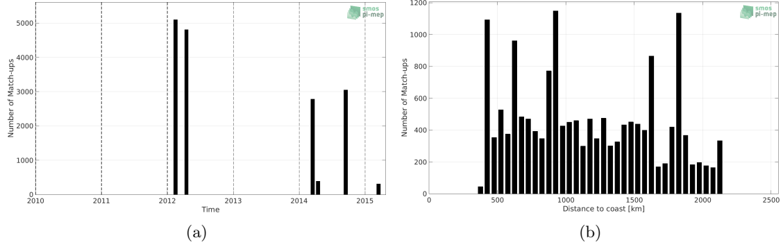
Figure 1: Number of match-ups between TSG (SAMOS) and Aquarius SSS L4 OI v5 - Monthly (IPRC) SSS as a function of time (a) and as function of the distance to coast (b) over the OTT zone Pi-MEP region and for the full satellite product period.
