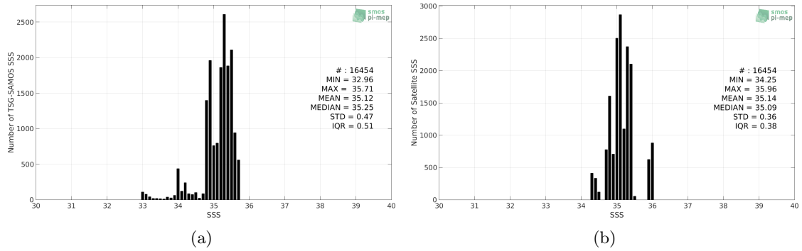
Figure 2: Histograms of SSS from TSG-SAMOS (a) and Aquarius-L4-IPRC-V5-MONTHLY (b) considering all match-up pairs per bins of 0.1 over the OTT zone Pi-MEP region and for the full satellite product period.
