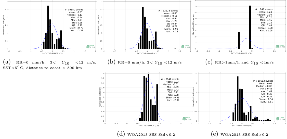
Figure 13: Normalized histogram of \Delta\text{SSS} (Aquarius-L4-IPRC-V5-MONTHLY - TSG-SAMOS) for 5 different subdatasets corresponding to: RR=0 mm/h, 3 < U_{10} < 12 m/s, SST > 5^\circ\text{C} , distance to coast > 800 km (a), RR=0 mm/h, 3 < U_{10} < 12 m/s (b), RR > 1 mm/h and U_{10} < 4 m/s (c), WOA2013 SSS Std < 0.2 (d), WOA2013 SSS Std > 0.2 (e).
