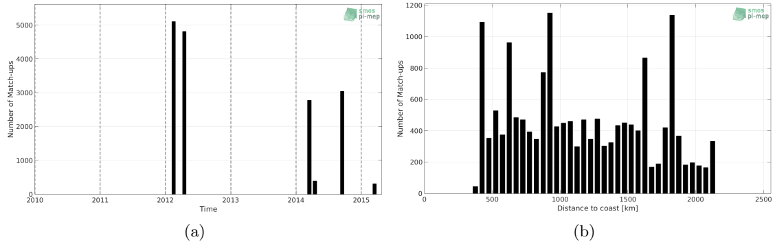
Figure 1: Number of match-ups between TSG-SAMOS and Aquarius-L4-IPRC-V5-MONTHLY SSS as a function of time (a) and as function of the distance to coast (b) over the OTT zone Pi-MEP region and for the full satellite product period.
