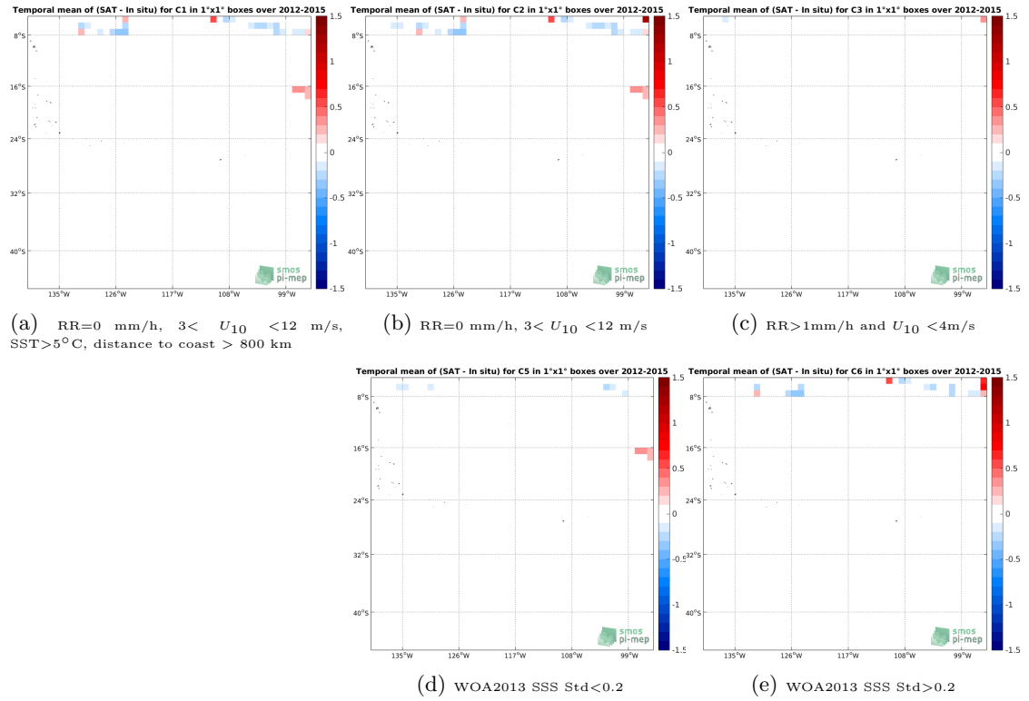
Figure 12: Temporal mean gridded over spatial boxes of size 1^\circ \times 1^\circ of \Delta SSS (Aquarius-L4-IPRC-V5-MONTHLY - TSG-SAMOS) for 5 different subdatasets corresponding to:RR=0 mm/h, 3 < U_{10} < 12 m/s, SST >5^\circ C, distance to coast > 800 km (a), RR=0 mm/h, 3 < U_{10} < 12 m/s (b), RR >1 mm/h and U_{10} < 4 m/s (c), WOA2013 SSS Std <0.2 (d), WOA2013 SSS Std >0.2 (e).
