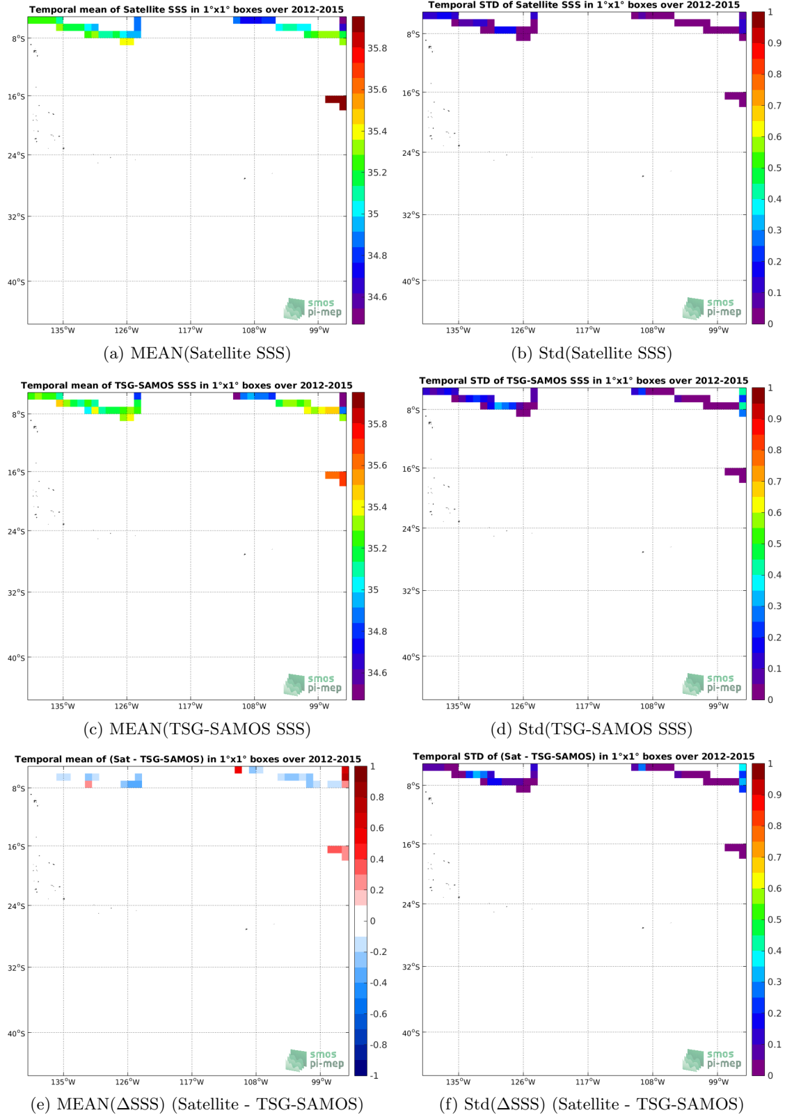
Figure 6: Temporal mean (left) and Std (right) of SSS from Aquarius-L4-IPRC-V5-MONTHLY (top), TSG-SAMOS (middle), and of \Delta SSS (Satellite - TSG-SAMOS). Only match-up pairs are used to generate these maps.
