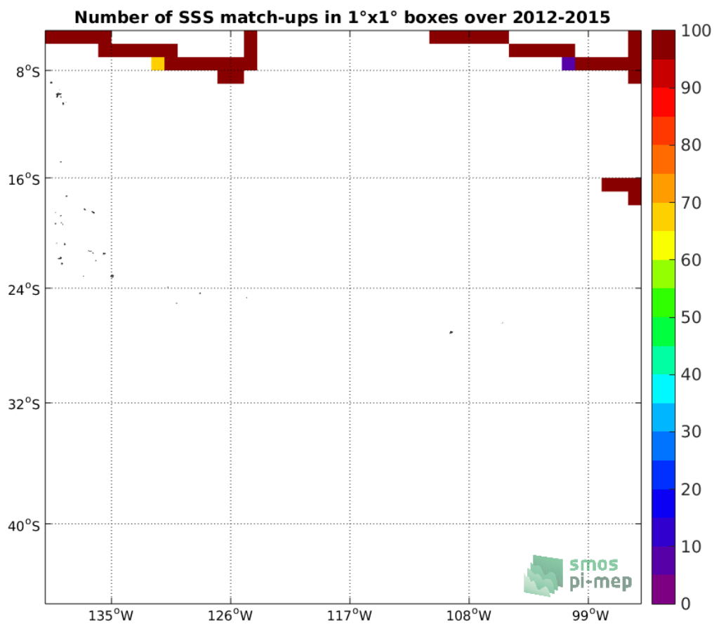
Figure 4: Number of SSS match-ups between TSG-SAMOS SSS and the Aquarius-L4-IPRC-V5-MONTHLY SSS product for the OTT zone Pi-MEP region over 1°x1° boxes and for the full satellite product period.
