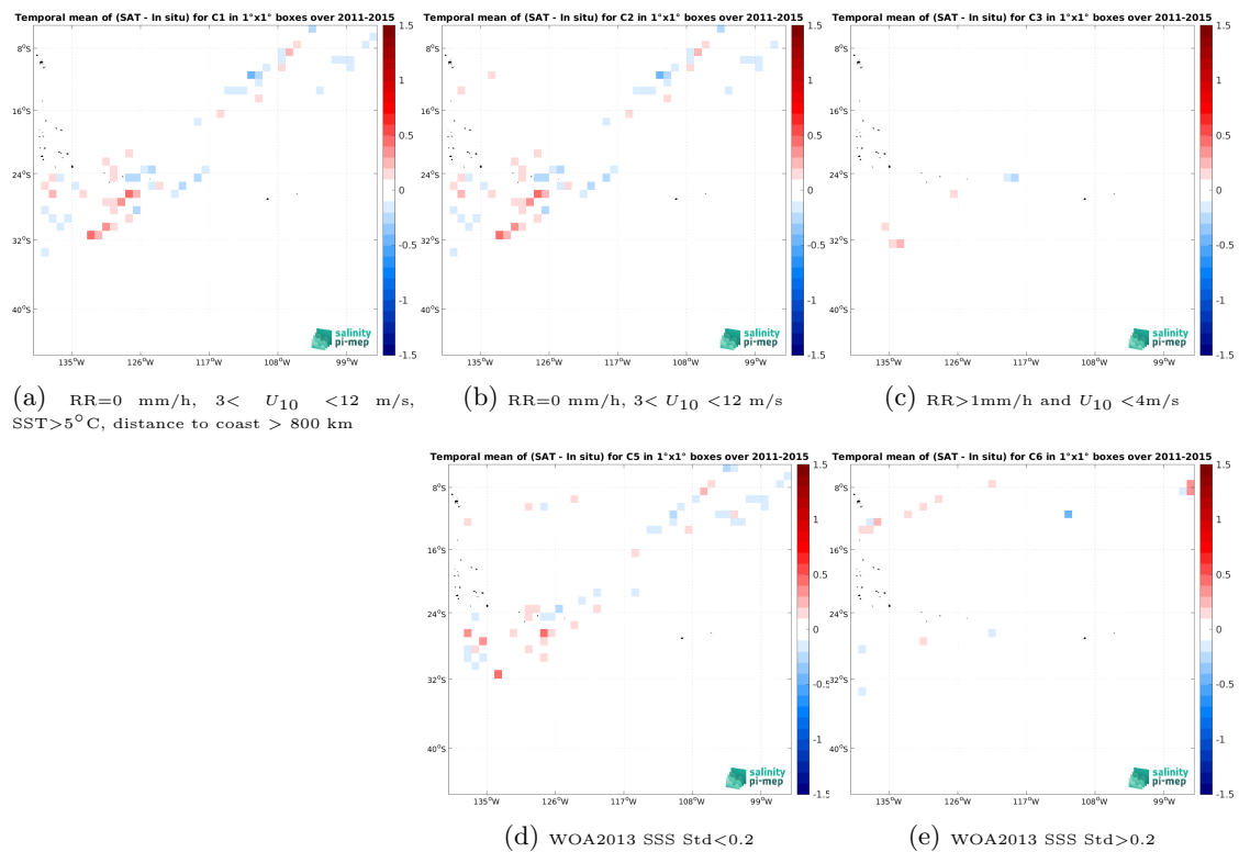
Figure 14: Temporal mean gridded over spatial boxes of size 1^\circ \times 1^\circ of \Delta\text{SSS} (Aquarius SSS L4 OI v5 - Monthly (IPRC) - TSG (LEGOS-DM)) for 5 different subdatasets corresponding to:RR=0 mm/h, 3 < U_{10} < 12 m/s, SST >5^\circ\text{C} , distance to coast > 800 km (a), RR=0 mm/h, 3 < U_{10} < 12 m/s (b), RR >1 mm/h and U_{10} < 4 m/s (c), WOA2013 SSS Std <0.2 (d), WOA2013 SSS Std >0.2 (e).
