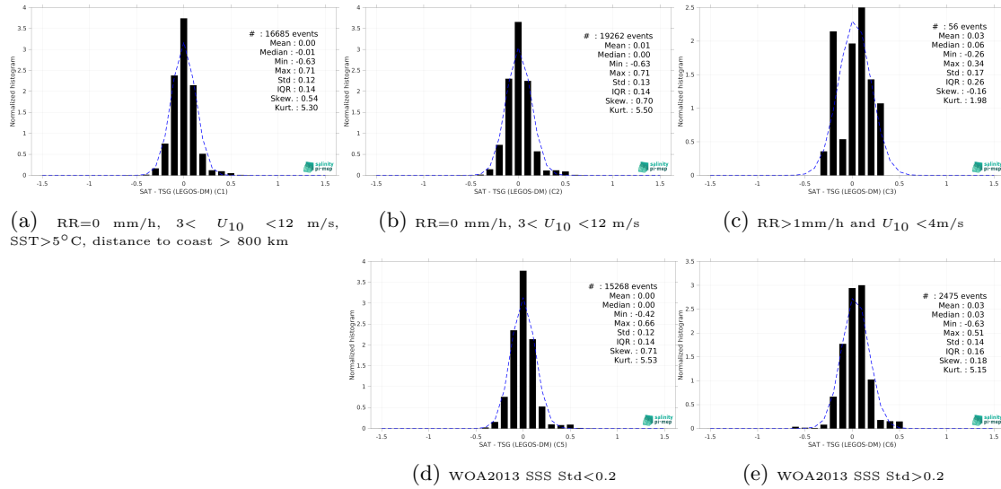
Figure 15: Normalized histogram of \Delta\text{SSS} (Aquarius SSS L4 OI v5 - Monthly (IPRC) - TSG (LEGOS-DM)) for 5 different subdatasets corresponding to: RR=0 mm/h, 3 < U_{10} < 12 m/s, SST>5°C, distance to coast > 800 km (a), RR=0 mm/h, 3 < U_{10} < 12 m/s (b), RR>1mm/h and U_{10} < 4 m/s (c), WOA2013 SSS Std<0.2 (d), WOA2013 SSS Std>0.2 (e).
