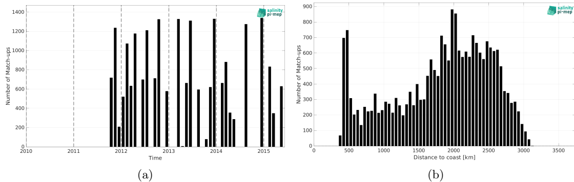
Figure 2: Number of match-ups between TSG (LEGOS-DM) and Aquarius SSS L4 OI v5 - Monthly (IPRC) SSS as a function of time (a) and as function of the distance to coast (b) over the OTT zone Pi-MEP region and for the full satellite product period.
