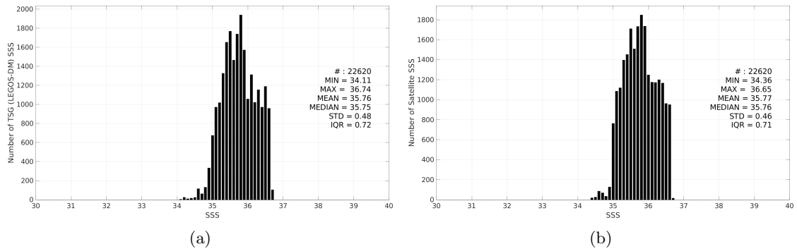
Figure 3: Histograms of SSS from TSG (LEGOS-DM) (a) and Aquarius SSS L4 OI v5 - Monthly (IPRC) (b) considering all match-up pairs per bins of 0.1 over the OTT zone Pi-MEP region and for the full satellite product period.
