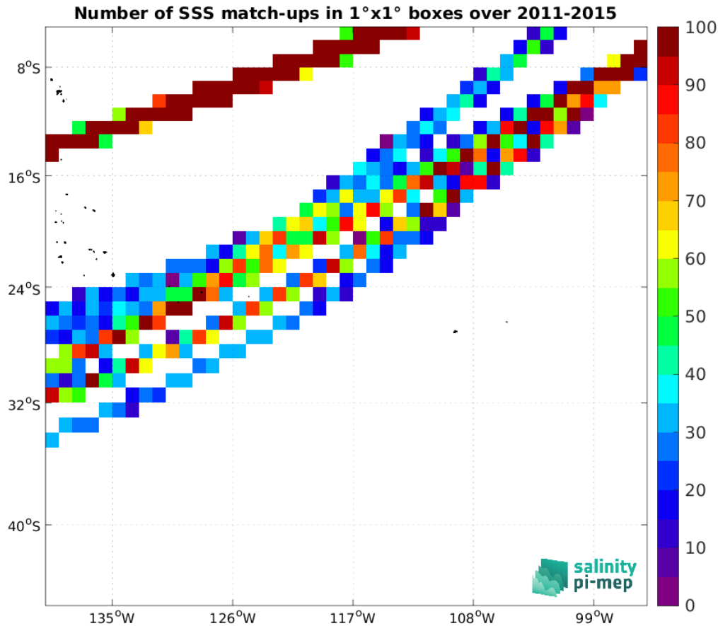
Figure 5: Number of SSS match-ups between TSG (LEGOS-DM) SSS and the Aquarius SSS L4 OI v5 - Monthly (IPRC) SSS product for the OTT zone Pi-MEP region over 1^\circ \times 1^\circ boxes and for the full satellite product period.
