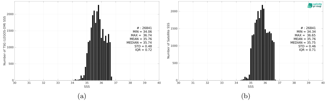
Figure 2: Histograms of SSS from TSG (LEGOS-DM) (a) and Aquarius SSS L4 OI v5 - Monthly (IPRC) (b) considering all match-up pairs per bins of 0.1 over the OTT zone Pi-MEP region and for the full satellite product period.
