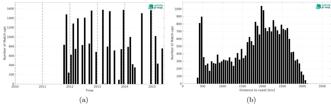
Figure 1: Number of match-ups between TSG (LEGOS-DM) and Aquarius SSS L4 OI v5 - Monthly (IPRC) SSS as a function of time (a) and as function of the distance to coast (b) over the OTT zone Pi-MEP region and for the full satellite product period.
