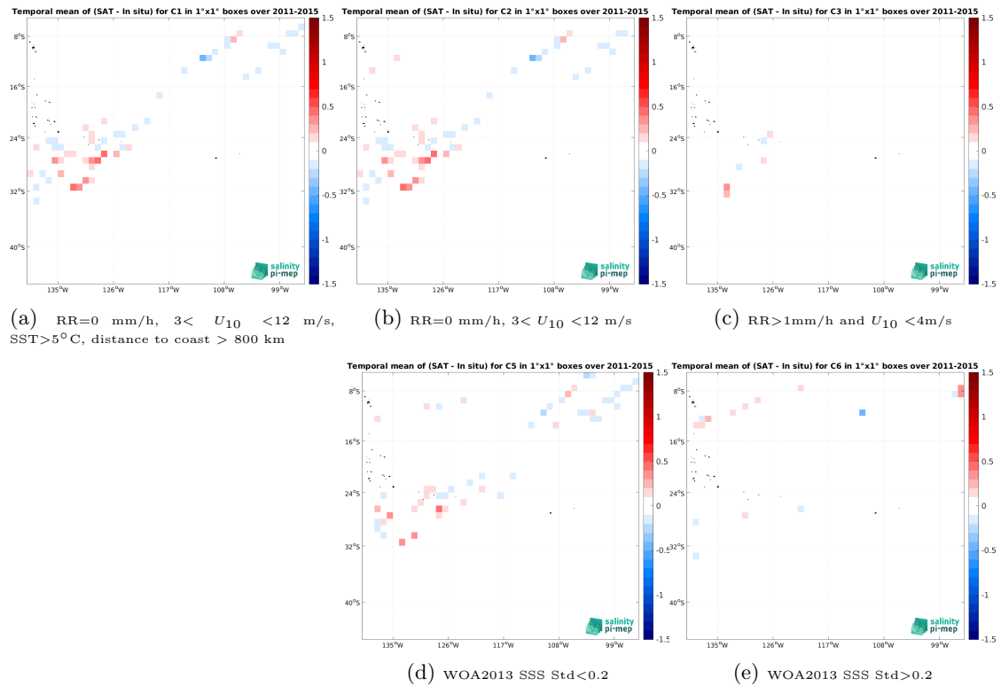
Figure 12: Temporal mean gridded over spatial boxes of size 1^\circ \times 1^\circ of \Delta SSS (Aquarius SSS L4 OI v5 - Monthly (IPRC) - TSG (LEGOS-DM)) for 5 different subdatasets corresponding to:RR=0 mm/h, 3 < U_{10} < 12 m/s, SST >5^\circ C, distance to coast > 800 km (a), RR=0 mm/h, 3 < U_{10} < 12 m/s (b), RR >1 mm/h and U_{10} < 4 m/s (c), WOA2013 SSS Std <0.2 (d), WOA2013 SSS Std >0.2 (e).
