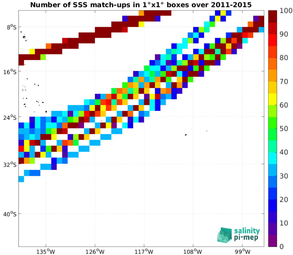
Figure 4: Number of SSS match-ups between TSG (LEGOS-DM) SSS and the Aquarius SSS L4 OI v5 - Monthly (IPRC) SSS product for the OTT zone Pi-MEP region over 1^\circ \times 1^\circ boxes and for the full satellite product period.
