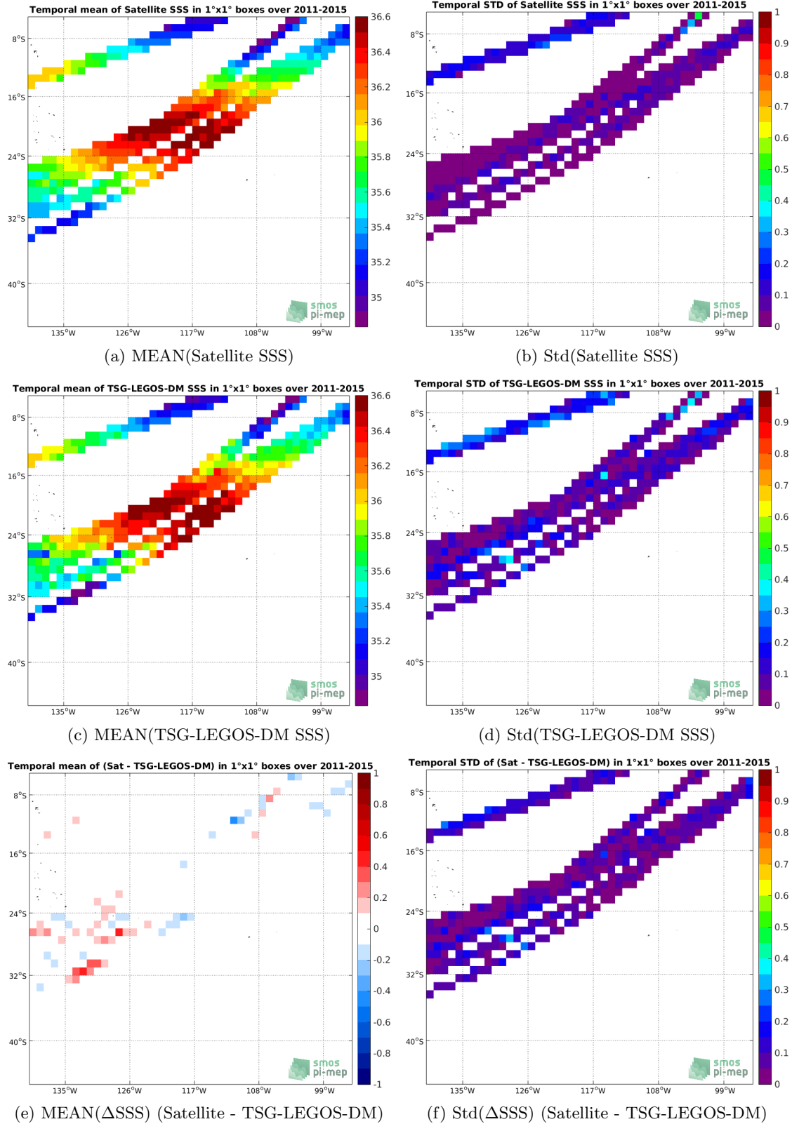
Figure 6: Temporal mean (left) and Std (right) of SSS from Aquarius-L4-IPRC-V5-MONTHLY (top), TSG-LEGOS-DM (middle), and of \Delta SSS 22 (Satellite - TSG-LEGOS-DM). Only match-up pairs are used to generate these maps.
