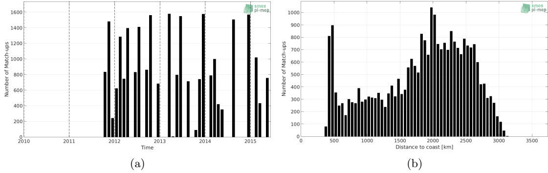
Figure 1: Number of match-ups between TSG-LEGOS-DM and Aquarius-L4-IPRC-V5-MONTHLY SSS as a function of time (a) and as function of the distance to coast (b) over the OTT zone Pi-MEP region and for the full satellite product period.
