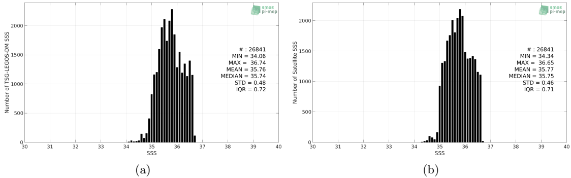
Figure 2: Histograms of SSS from TSG-LEGOS-DM (a) and Aquarius-L4-IPRC-V5-MONTHLY (b) considering all match-up pairs per bins of 0.1 over the OTT zone Pi-MEP region and for the full satellite product period.
