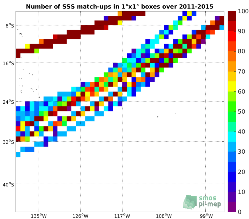
Figure 4: Number of SSS match-ups between TSG-LEGOS-DM SSS and the Aquarius-L4-IPRC-V5-MONTHLY SSS product for the OTT zone Pi-MEP region over 1°x1° boxes and for the full satellite product period.
