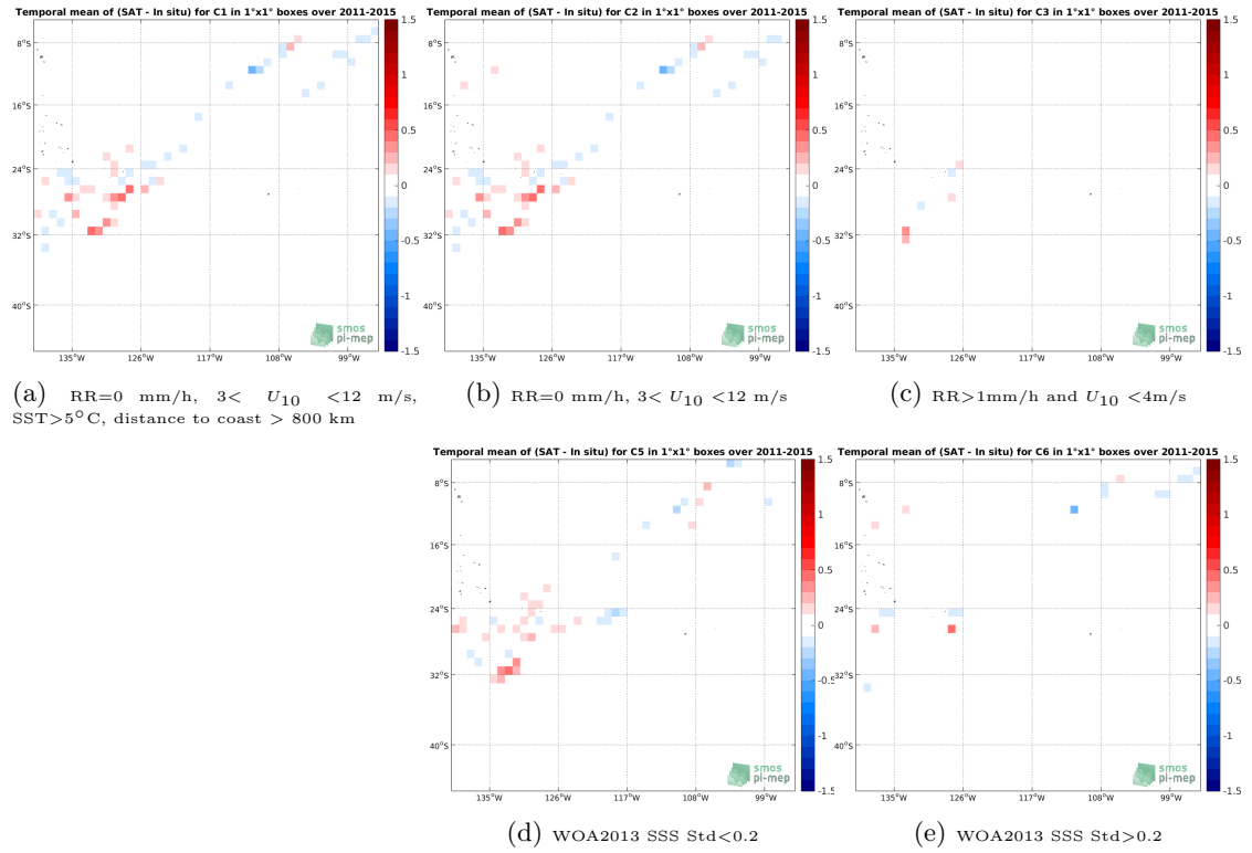
Figure 12: Temporal mean gridded over spatial boxes of size 1^\circ \times 1^\circ of \Delta SSS (Aquarius-L4-IPRC-V5-MONTHLY - TSG-LEGOS-DM) for 5 different subdatasets corresponding to:RR=0 mm/h, 3 < U_{10} < 12 m/s, SST >5^\circ\text{C} , distance to coast > 800 km (a), RR=0 mm/h, 3 < U_{10} < 12 m/s (b), RR >1 mm/h and U_{10} < 4 m/s (c), WOA2013 SSS Std <0.2 (d), WOA2013 SSS Std >0.2 (e).
