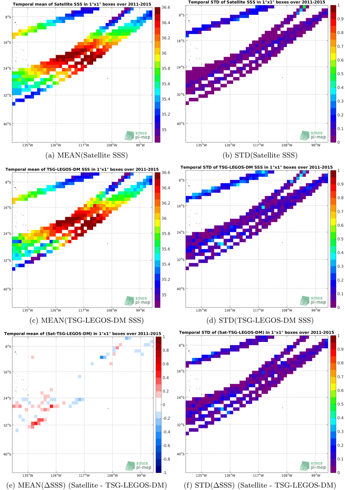
Figure 6: Temporal mean (left) and STD (right) of SSS from Aquarius-L4-IPRC-V5-MONTHLY (top), TSG-LEGOS-DM (middle), and of \Delta SSS (Satellite - TSG-LEGOS-DM). Only match-up pairs are used to generate these maps.
