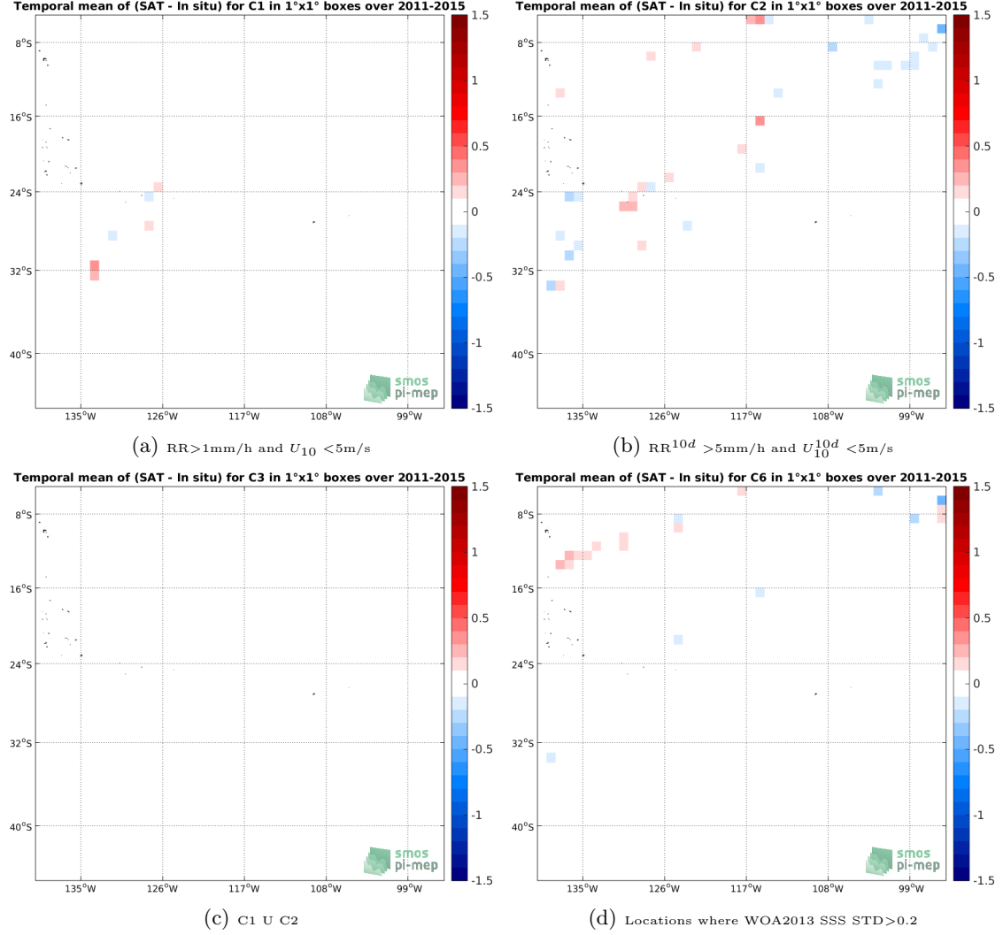
Figure 12: Temporal mean gridded over spatial boxes of size 1^\circ \times 1^\circ of \Delta SSS (Aquarius-L4-IPRC-V5-MONTHLY - TSG-LEGOS-DM) for 4 different subdatasets corresponding to: RR > 1\text{mm/h} and U_{10} < 5\text{m/s} (a), RR^{10d} > 5\text{mm/h} and U_{10}^{10d} < 5\text{m/s} (b), C1 U C2 (c), Locations where WOA2013 SSS STD > 0.2 (d).
