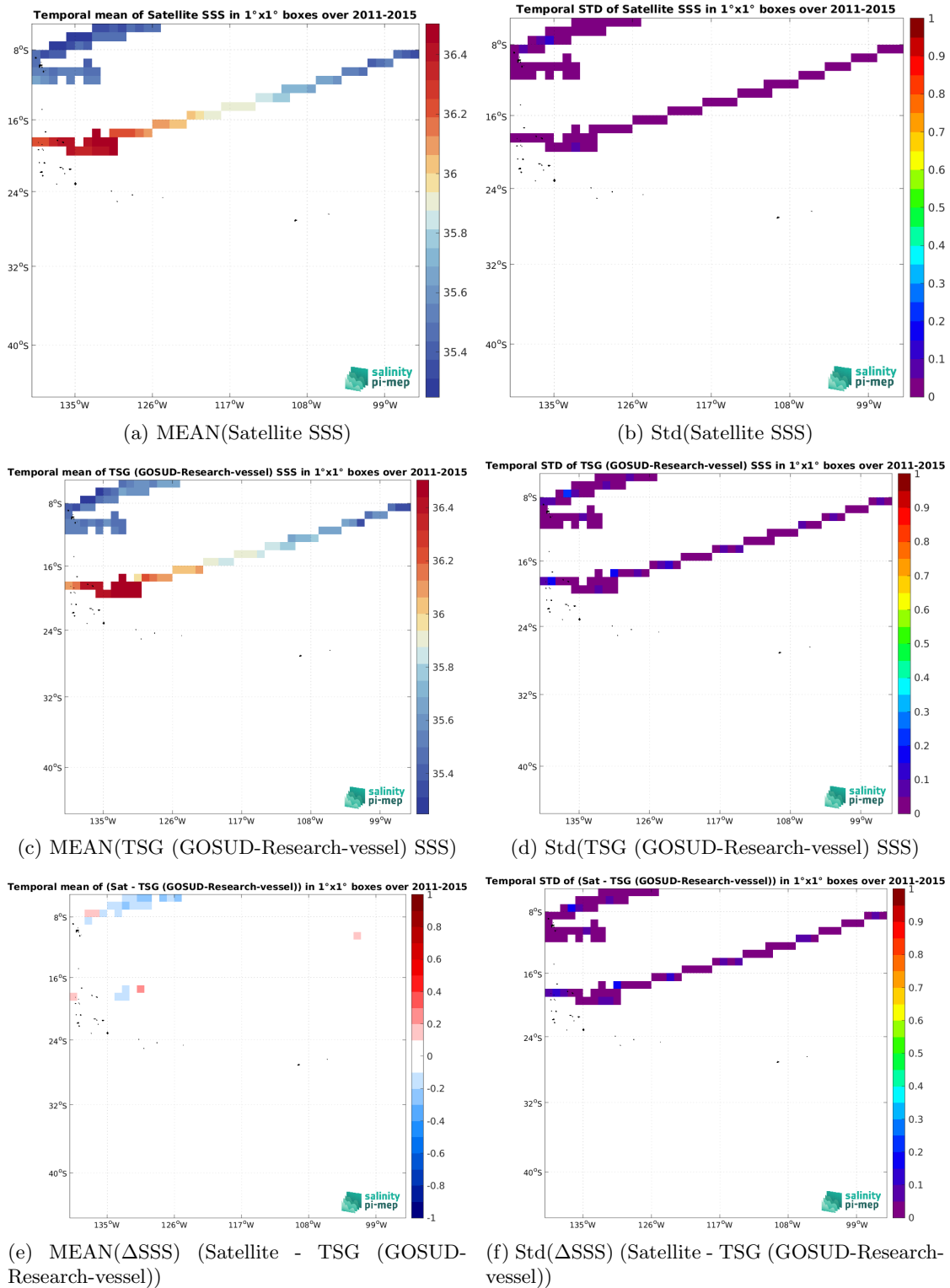
Figure 7: Temporal mean (left) and Std (right) of SSS from Aquarius SSS L4 OI v5 - Monthly (IPRC) (top), TSG (GOSUD-Research-vessel) (middle), and of \Delta SSS (Satellite - TSG (GOSUD-Research-vessel)). Only match-up pairs are used to generate these maps.
