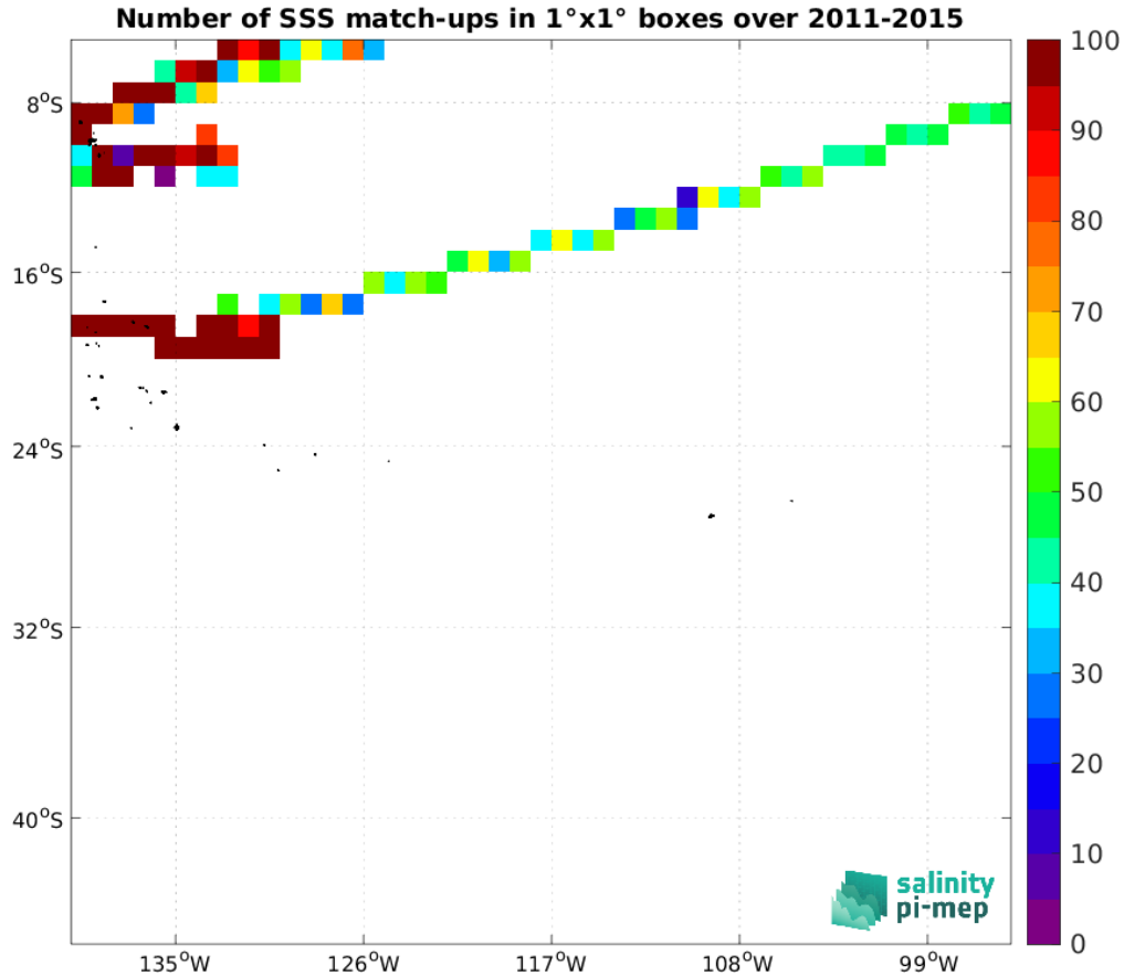
Figure 5: Number of SSS match-ups between TSG (GOSUD-Research-vessel) SSS and the Aquarius SSS L4 OI v5 - Monthly (IPRC) SSS product for the OTT zone Pi-MEP region over 1^\circ \times 1^\circ boxes and for the full satellite product period.
