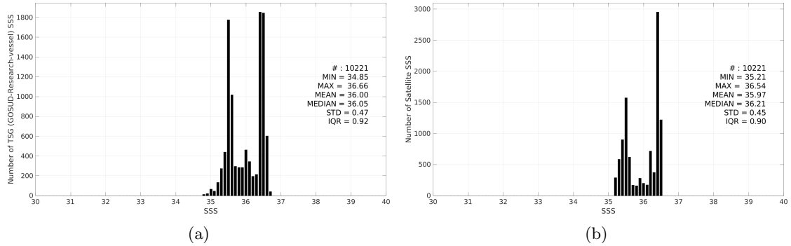
Figure 3: Histograms of SSS from TSG (GOSUD-Research-vessel) (a) and Aquarius SSS L4 OI v5 - Monthly (IPRC) (b) considering all match-up pairs per bins of 0.1 over the OTT zone Pi-MEP region and for the full satellite product period.
