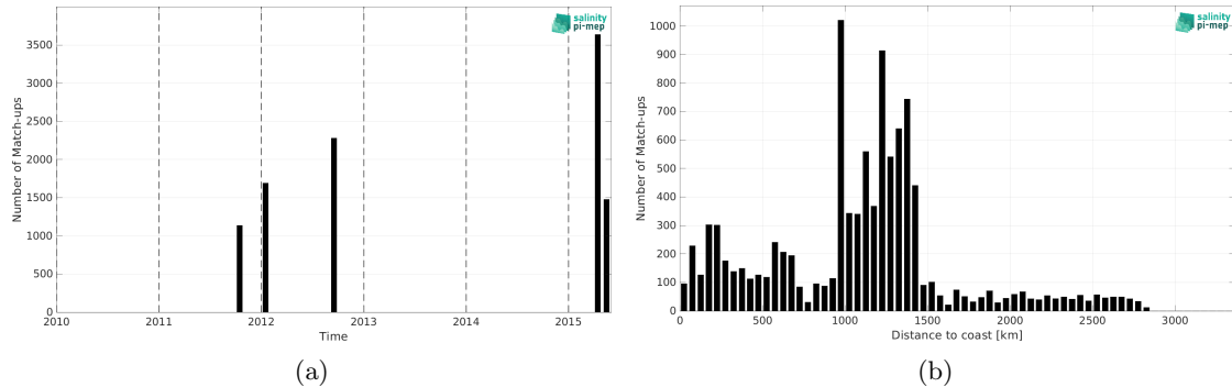
Figure 2: Number of match-ups between TSG (GOSUD-Research-vessel) and Aquarius SSS L4 OI v5 - Monthly (IPRC) SSS as a function of time (a) and as function of the distance to coast (b) over the OTT zone Pi-MEP region and for the full satellite product period.
