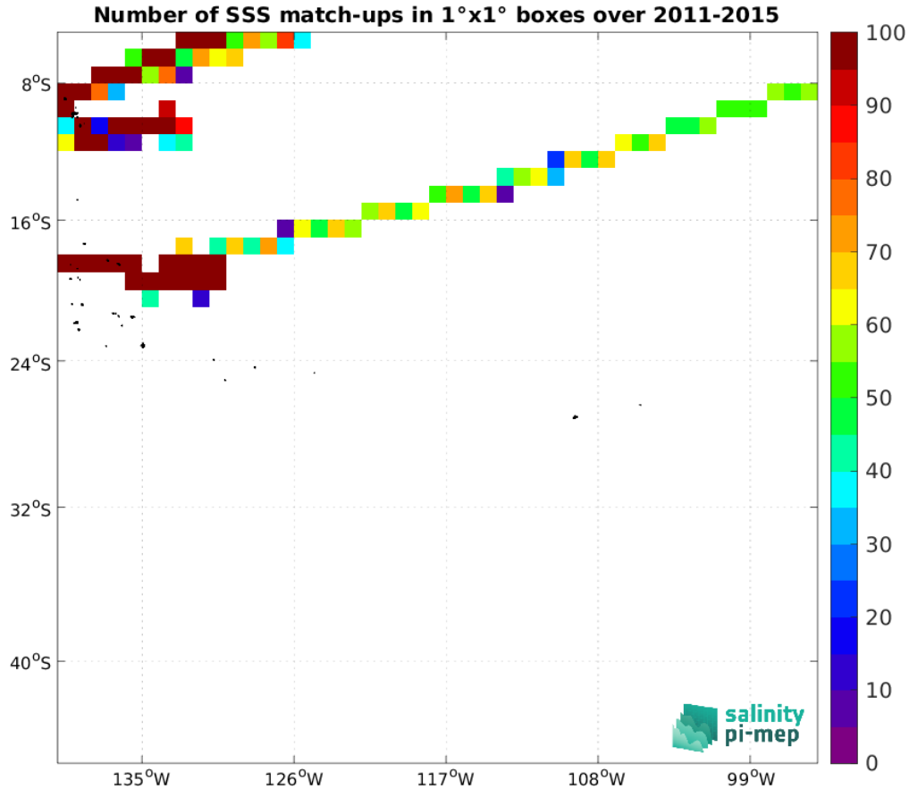
Figure 4: Number of SSS match-ups between TSG (GOSUD-Research-vessel) SSS and the Aquarius SSS L4 OI v5 - Monthly (IPRC) SSS product for the OTT zone Pi-MEP region over 1^\circ \times 1^\circ boxes and for the full satellite product period.
