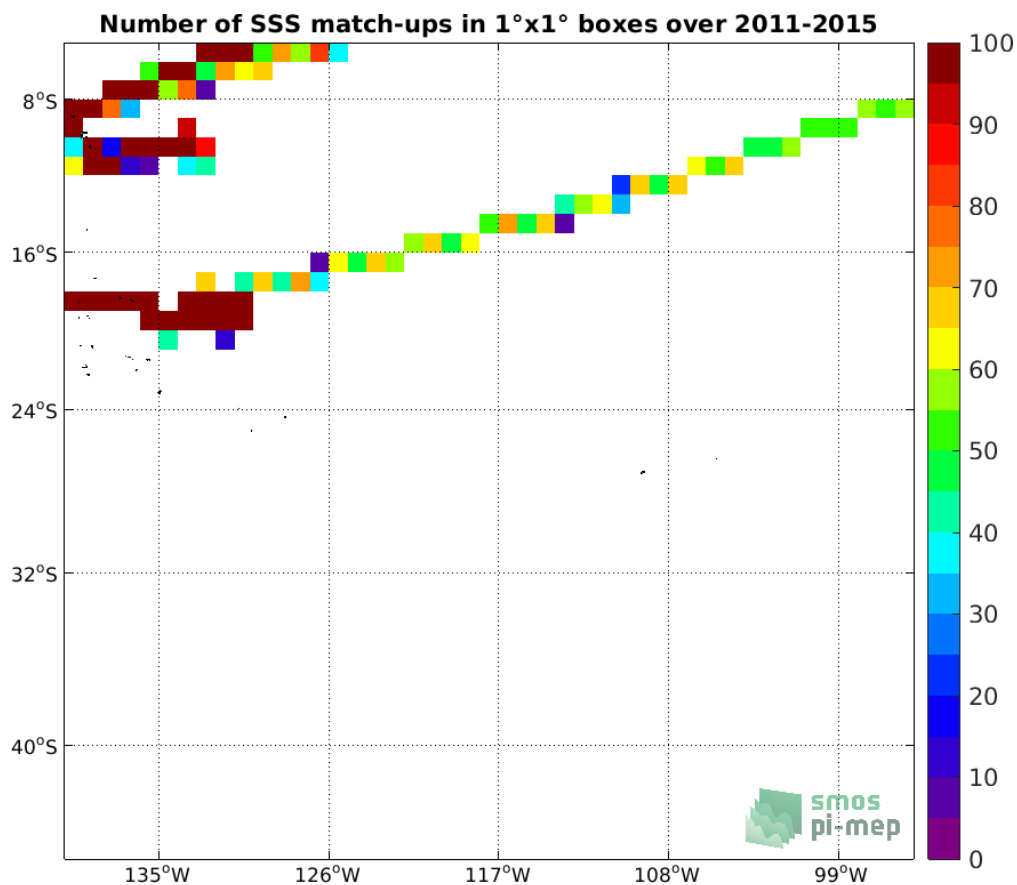
Figure 4: Number of SSS match-ups between TSG (GOSUD-Research-vessel) SSS and the Aquarius SSS L4 OI v5 - Monthly (IPRC) SSS product for the OTT zone Pi-MEP region over 1°x1° boxes and for the full satellite product period.
