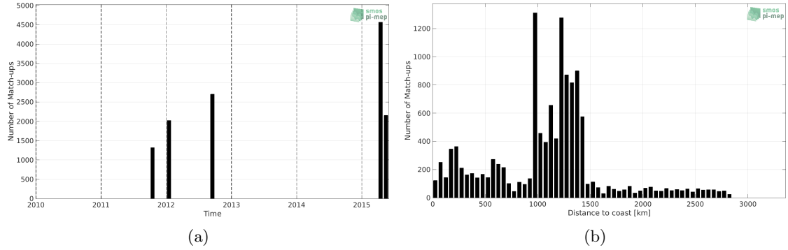
Figure 1: Number of match-ups between TSG (GOSUD-Research-vessel) and Aquarius SSS L4 OI v5 - Monthly (IPRC) SSS as a function of time (a) and as function of the distance to coast (b) over the OTT zone Pi-MEP region and for the full satellite product period.
