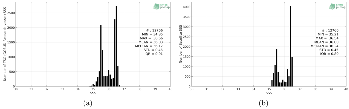
Figure 2: Histograms of SSS from TSG (GOSUD-Research-vessel) (a) and Aquarius SSS L4 OI v5 - Monthly (IPRC) (b) considering all match-up pairs per bins of 0.1 over the OTT zone Pi-MEP region and for the full satellite product period.
