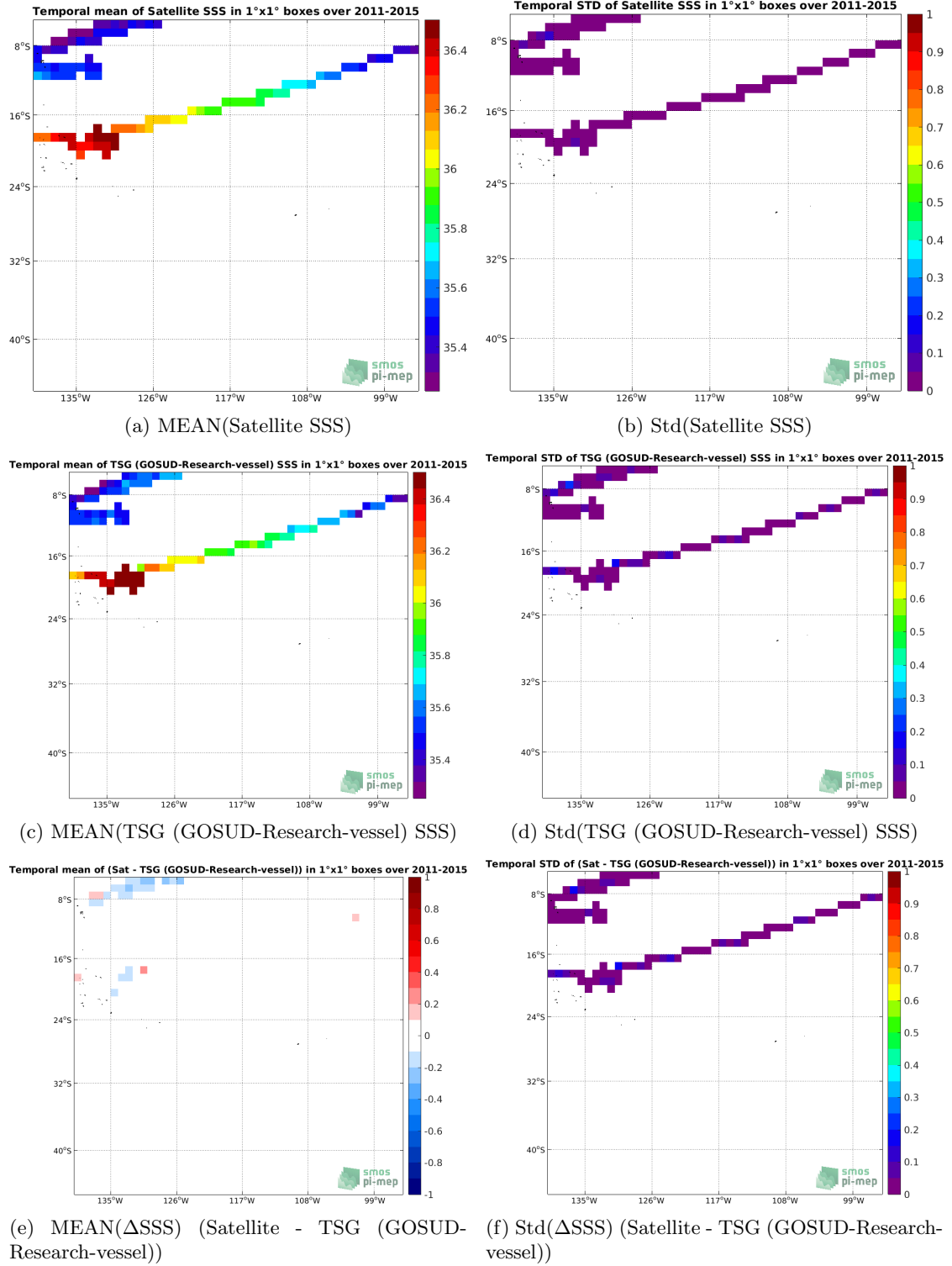
Figure 6: Temporal mean (left) and Std (right) of SSS from Aquarius SSS L4 OI v5 - Monthly (IPRC) (top), TSG (GOSUD-Research-vessel) (middle), and of \Delta SSS (Satellite - TSG (GOSUD-Research-vessel)). Only match-up pairs are used to generate these maps.
