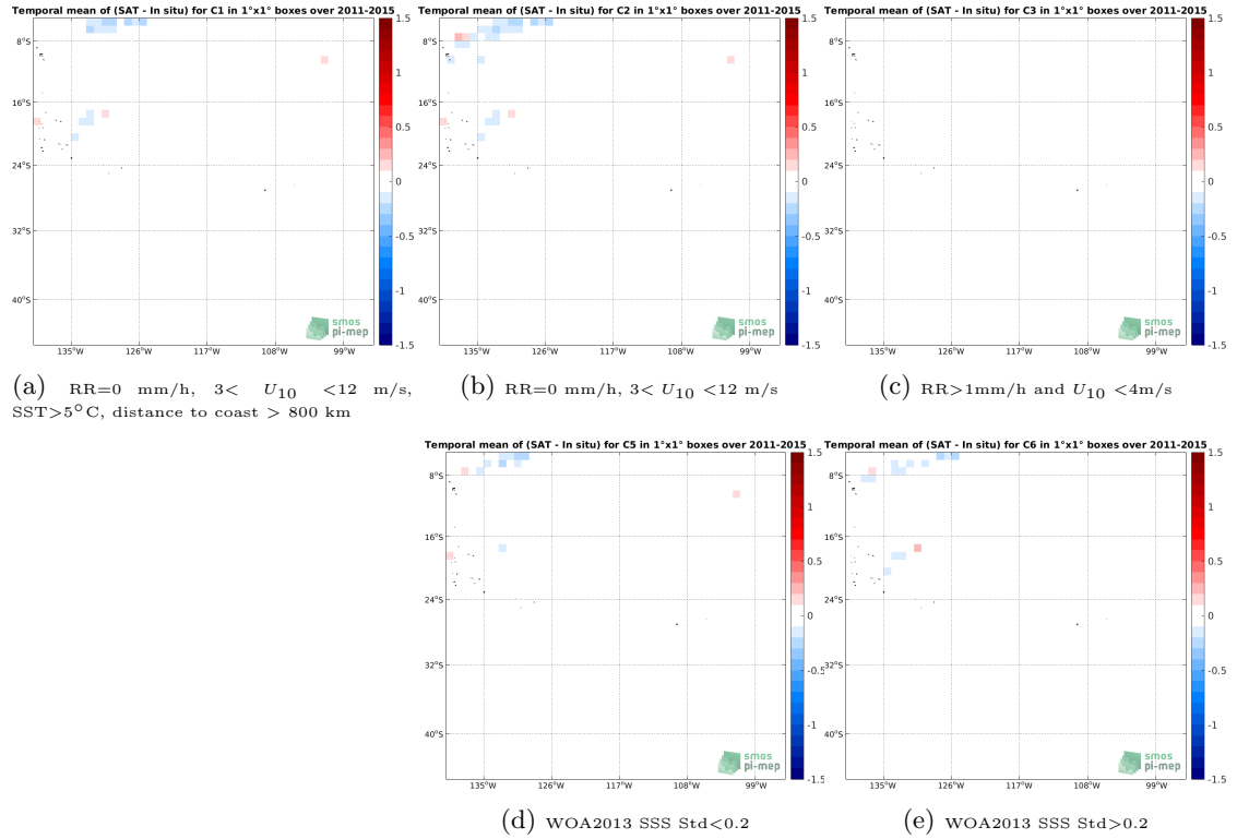
Figure 12: Temporal mean gridded over spatial boxes of size 1^\circ \times 1^\circ of \Delta SSS (Aquarius SSS L4 OI v5 - Monthly (IPRC) - TSG (GOSUD-Research-vessel)) for 5 different subdatasets corresponding to: RR=0 mm/h, 3 < U_{10} < 12 m/s, SST >5^\circ\text{C} , distance to coast > 800 km (a), RR=0 mm/h, 3 < U_{10} < 12 m/s (b), RR >1 mm/h and U_{10} < 4 m/s (c), WOA2013 SSS Std <0.2 (d), WOA2013 SSS Std >0.2 (e).
