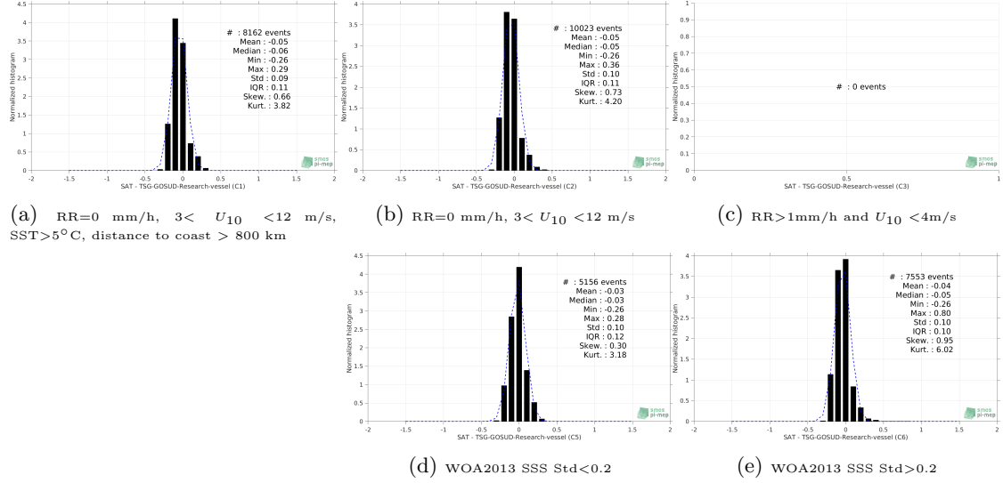
Figure 13: Normalized histogram of \Delta\text{SSS} (Aquarius-L4-IPRC-V5-MONTHLY - TSG-GOSUD-Research-vessel) for 5 different subdatasets corresponding to: RR=0 mm/h, 3 < U_{10} < 12 m/s, SST > 5^\circ\text{C} , distance to coast > 800 km (a), RR=0 mm/h, 3 < U_{10} < 12 m/s (b), RR > 1 mm/h and U_{10} < 4 m/s (c), WOA2013 SSS Std < 0.2 (d), WOA2013 SSS Std > 0.2 (e).
