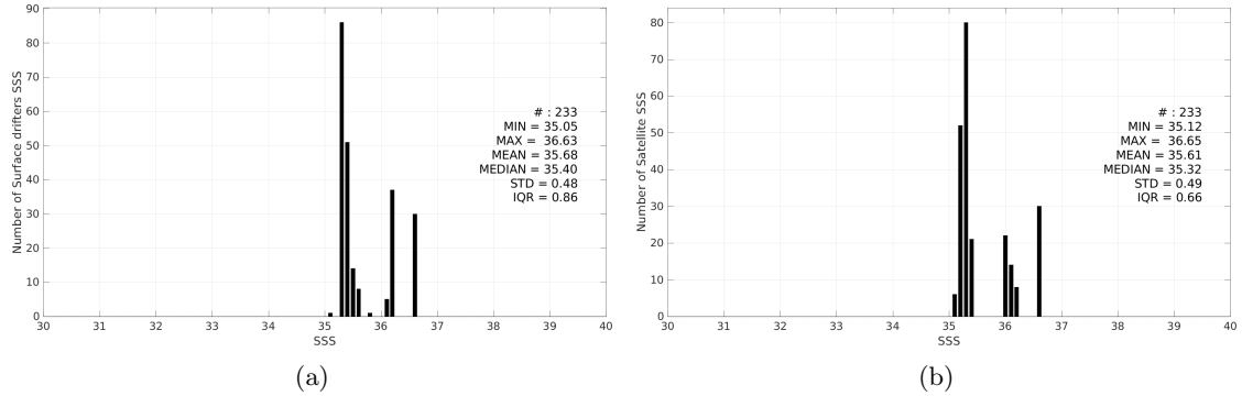
Figure 3: Histograms of SSS from Surface drifters (a) and Aquarius SSS L4 OI v5 - Monthly (IPRC) (b) considering all match-up pairs per bins of 0.1 over the OTT zone Pi-MEP region and for the full satellite product period.
