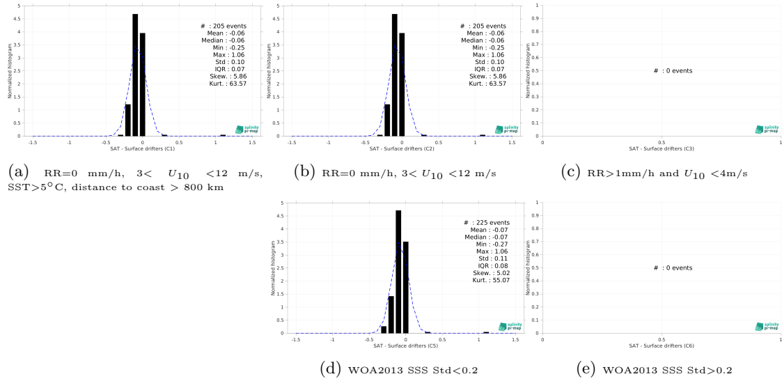
Figure 14: Normalized histogram of \Delta\text{SSS} (Aquarius SSS L4 OI v5 - Monthly (IPRC) - Surface drifters) for 5 different subdatasets corresponding to: RR=0 mm/h, 3 < U_{10} < 12 m/s, SST > 5^\circ\text{C} , distance to coast > 800 km (a), RR=0 mm/h, 3 < U_{10} < 12 m/s (b), RR > 1\text{mm/h} and U_{10} < 4\text{m/s} (c), WOA2013 SSS Std < 0.2 (d), WOA2013 SSS Std > 0.2 (e).
