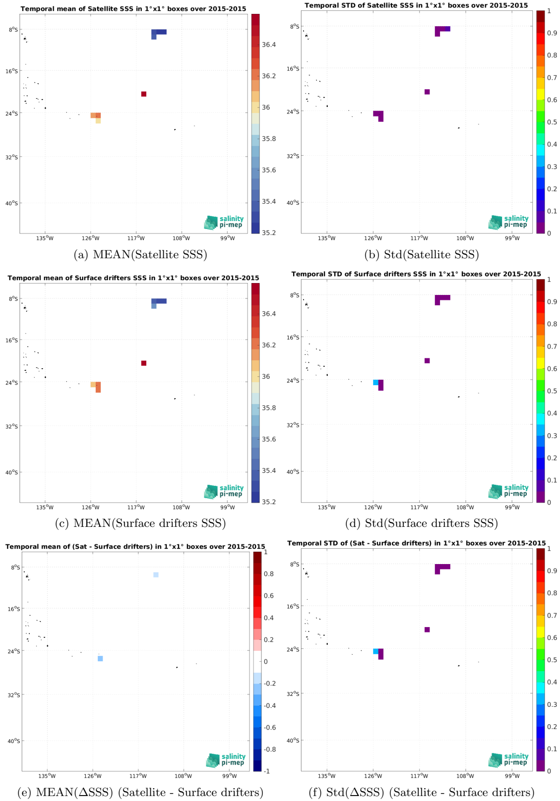
Figure 6: Temporal mean (left) and Std (right) of SSS from Aquarius SSS L4 OI v5 - Monthly (IPRC) (top), Surface drifters (middle), and of \Delta SSS (Satellite - Surface drifters). Only match-up pairs are used to generate these maps.
