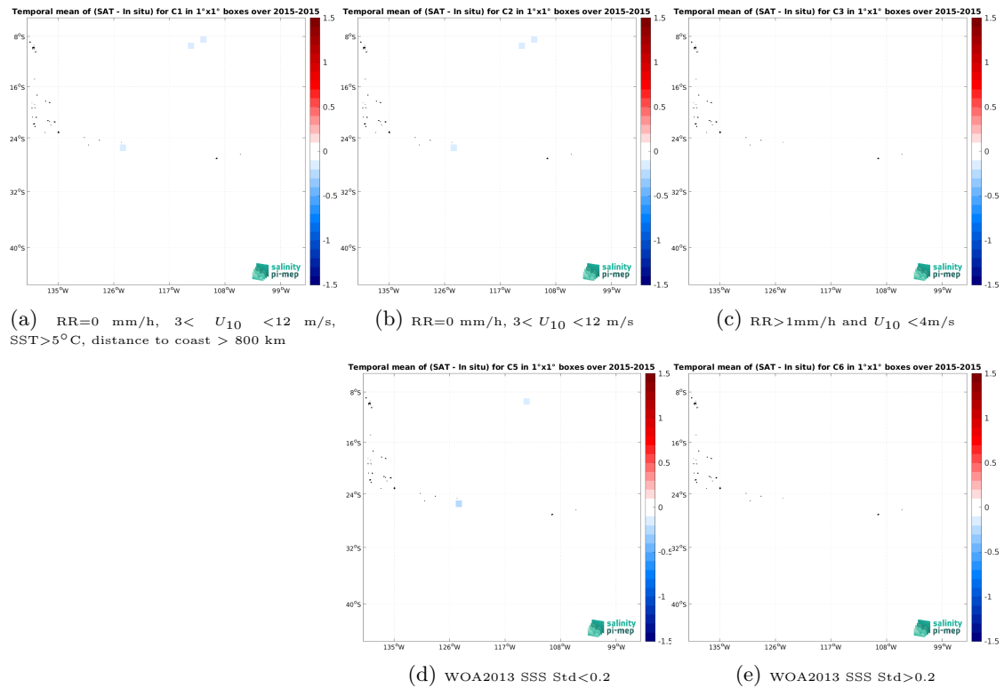
Figure 13: Temporal mean gridded over spatial boxes of size 1^\circ \times 1^\circ of \Delta SSS (Aquarius SSS L4 OI v5 - Monthly (IPRC) - Surface drifters) for 5 different subdatasets corresponding to:RR=0 mm/h, 3 < U_{10} < 12 m/s, SST >5^\circ C, distance to coast > 800 km (a), RR=0 mm/h, 3 < U_{10} < 12 m/s (b), RR >1 mm/h and U_{10} < 4 m/s (c), WOA2013 SSS Std <0.2 (d), WOA2013 SSS Std >0.2 (e).
