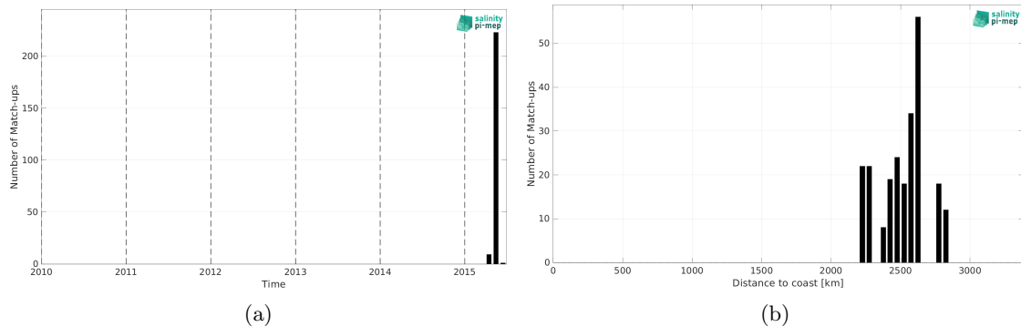
Figure 2: Number of match-ups between Surface drifters and Aquarius SSS L4 OI v5 - Monthly (IPRC) SSS as a function of time (a) and as function of the distance to coast (b) over the OTT zone Pi-MEP region and for the full satellite product period.
