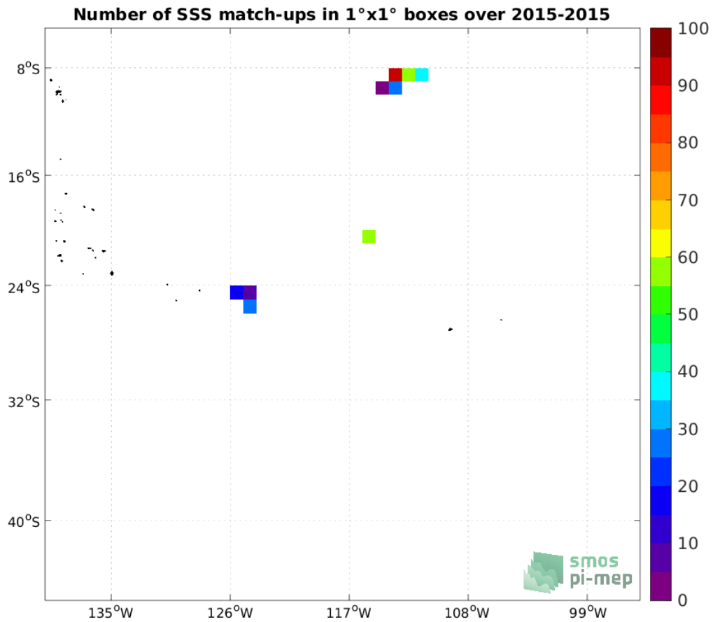
Figure 3: Number of SSS match-ups between Surface drifters SSS and the Aquarius SSS L4 OI v5 - Monthly (IPRC) SSS product for the OTT zone Pi-MEP region over 1°x1° boxes and for the full satellite product period.
