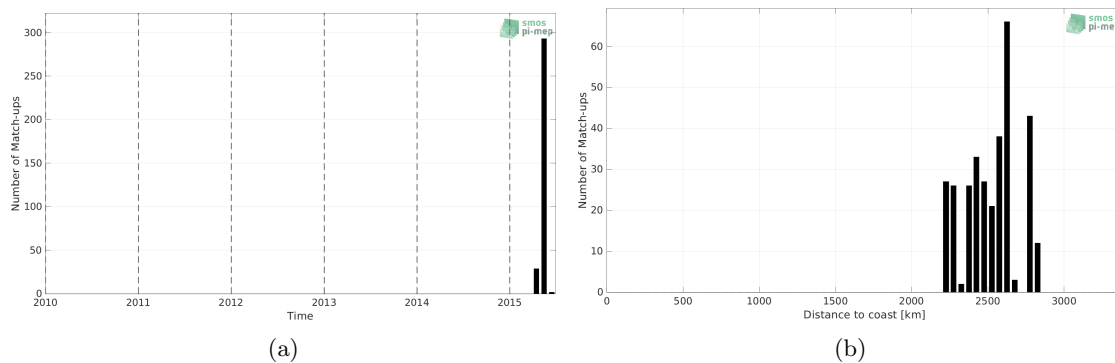
Figure 1: Number of match-ups between Surface drifters and Aquarius SSS L4 OI v5 - Monthly (IPRC) SSS as a function of time (a) and as function of the distance to coast (b) over the OTT zone Pi-MEP region and for the full satellite product period.
