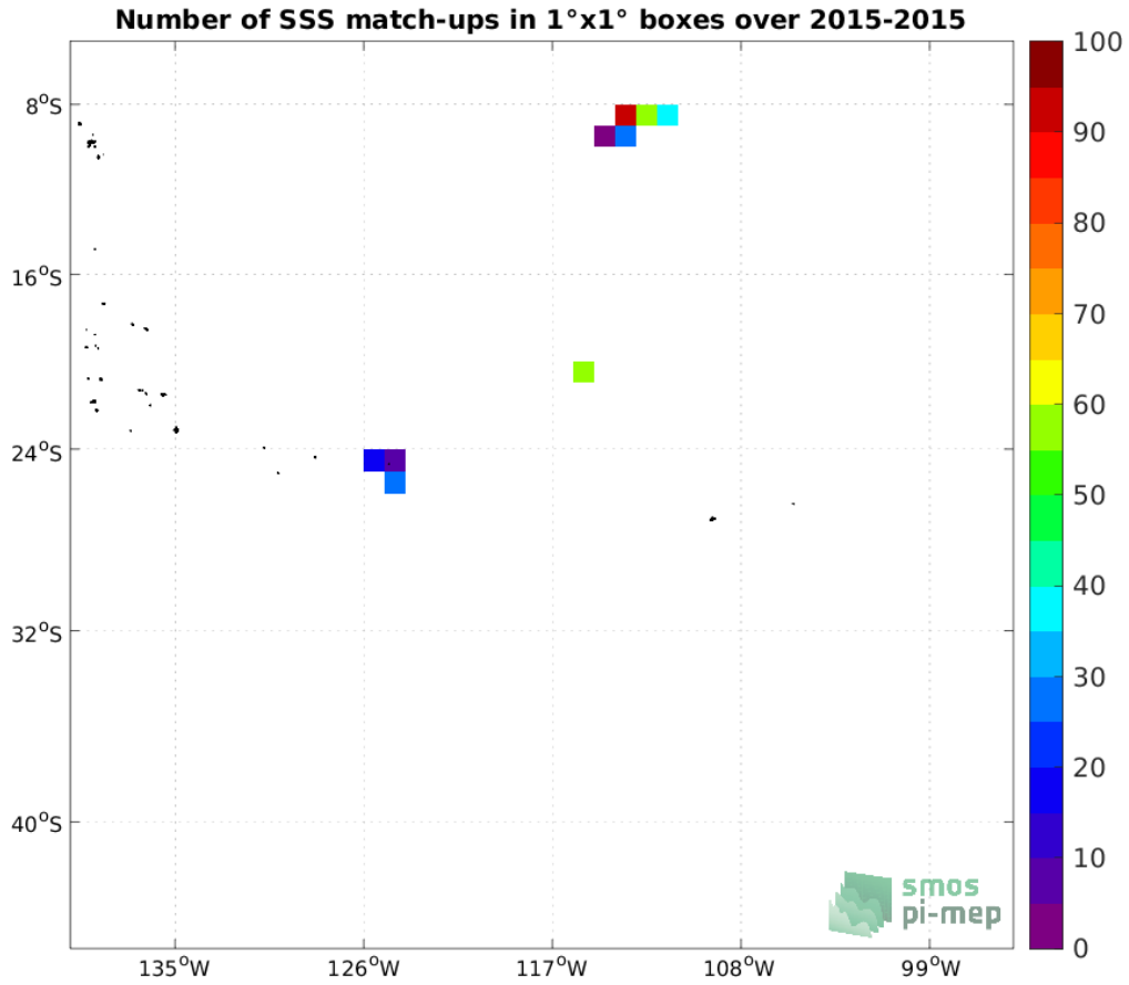
Figure 3: Number of SSS match-ups between Surface drifters SSS and the Aquarius SSS L4 OI v5 - Monthly (IPRC) SSS product for the OTT zone Pi-MEP region over 1^\circ \times 1^\circ boxes and for the full satellite product period.
