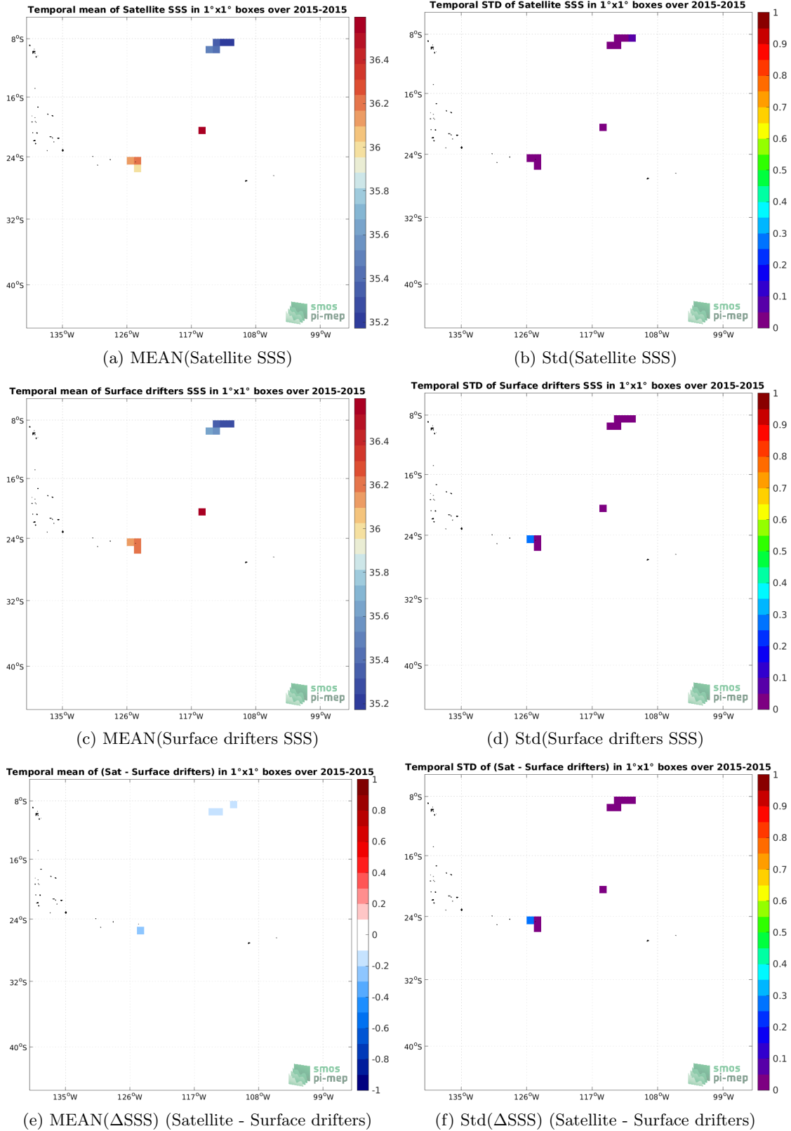
Figure 5: Temporal mean (left) and Std (right), of SSS from Aquarius SSS L4 OI v5 - Monthly (IPRC) (top), Surface drifters (middle), and of \Delta SSS (Satellite - Surface drifters). Only match-up pairs are used to generate these maps.
