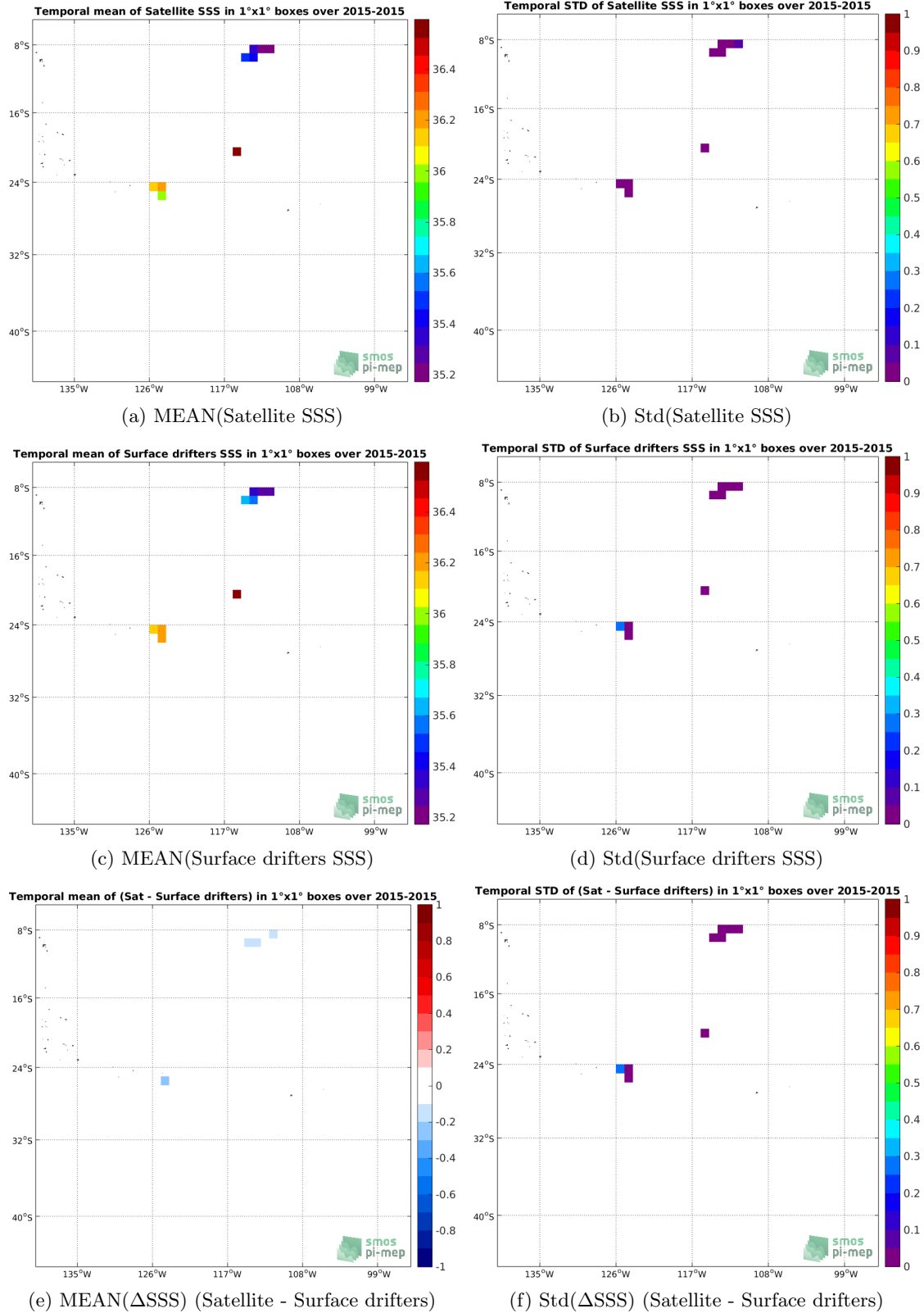
Figure 5: Temporal mean (left) and Std (right) of SSS from Aquarius-L4-IPRC-V5-MONTHLY (top), Surface drifters (middle), and of \Delta SSS (Satellite - Surface drifters). Only match-up pairs are used to generate these maps.
