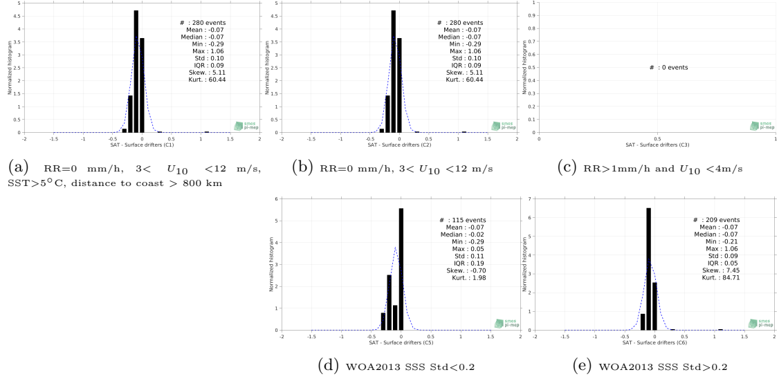
Figure 12: Normalized histogram of \Delta SSS (Aquarius-L4-IPRC-V5-MONTHLY - Surface drifters) for 5 different subdatasets corresponding to: RR=0 mm/h, 3 < U_{10} < 12 m/s, SST>5°C, distance to coast > 800 km (a), RR=0 mm/h, 3 < U_{10} < 12 m/s (b), RR>1mm/h and U_{10} < 4 m/s (c), WOA2013 SSS Std<0.2 (d), WOA2013 SSS Std>0.2 (e).
