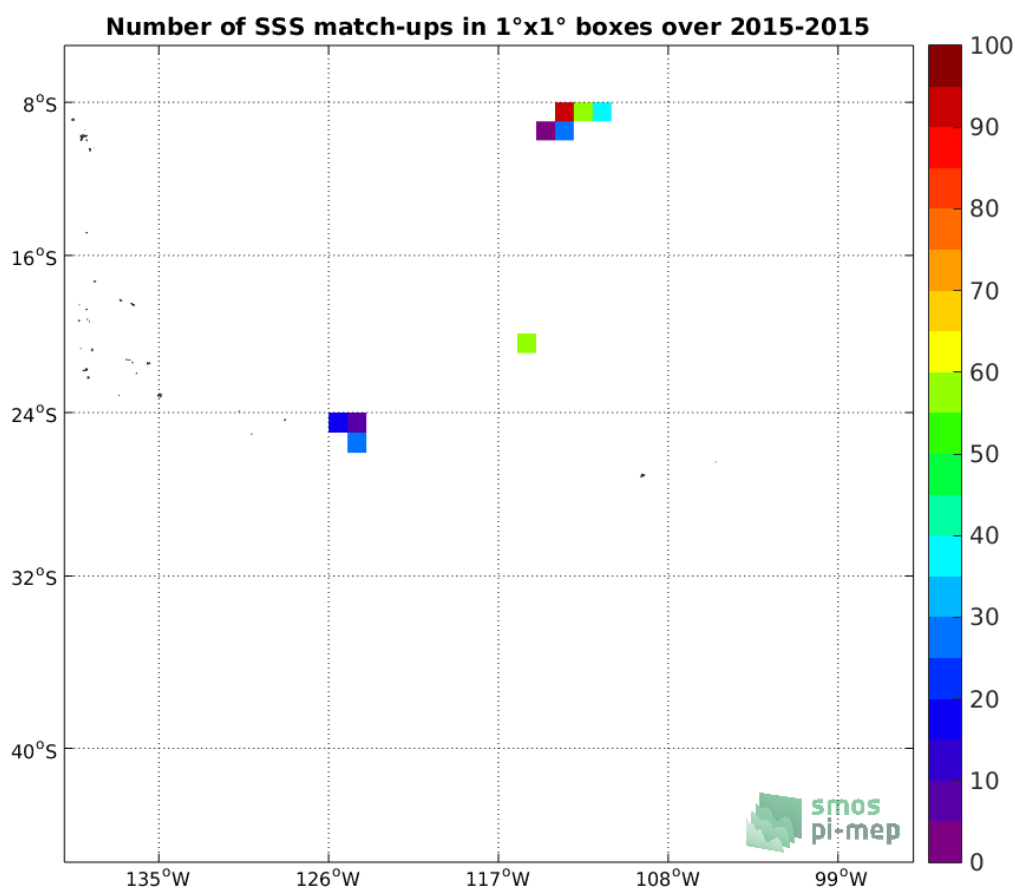
Figure 3: Number of SSS match-ups between Surface drifters SSS and the Aquarius-L4-IPRC-V5-MONTHLY SSS product for the OTT zone Pi-MEP region over 1°x1° boxes and for the full satellite product period.
