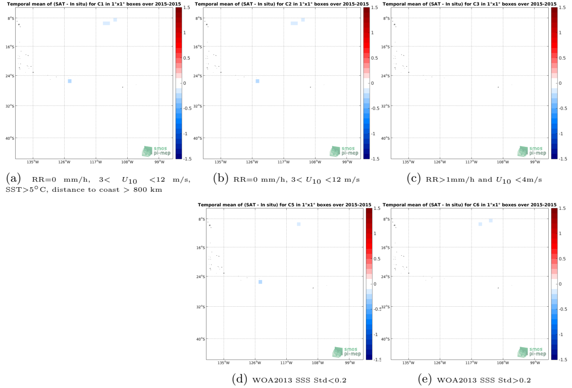
Figure 11: Temporal mean gridded over spatial boxes of size 1^\circ \times 1^\circ of \Delta SSS (Aquarius-L4-IPRC-V5-MONTHLY - Surface drifters) for 5 different subdatasets corresponding to: RR=0 mm/h, 3 < U_{10} < 12 m/s, SST > 5^\circ C , distance to coast > 800 km (a), RR=0 mm/h, 3 < U_{10} < 12 m/s (b), RR > 1 mm/h and U_{10} < 4 m/s (c), WOA2013 SSS Std < 0.2 (d), WOA2013 SSS Std > 0.2 (e).
