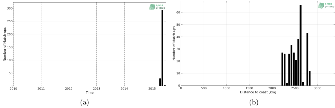
Figure 1: Number of match-ups between Surface drifters and Aquarius-L4-IPRC-V5-MONTHLY SSS as a function of time (a) and as function of the distance to coast (b) over the OTT zone Pi-MEP region and for the full satellite product period.
