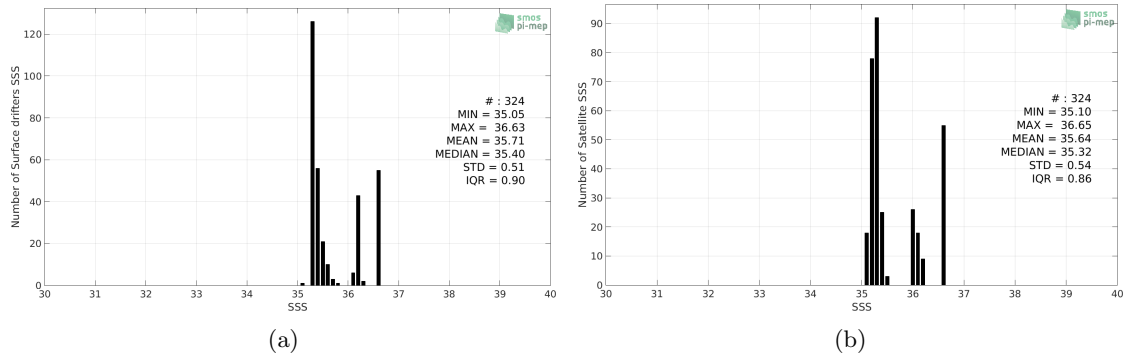
Figure 2: Histograms of SSS from Surface drifters (a) and Aquarius-L4-IPRC-V5-MONTHLY (b) considering all match-up pairs per bins of 0.1 over the OTT zone Pi-MEP region and for the full satellite product period.
