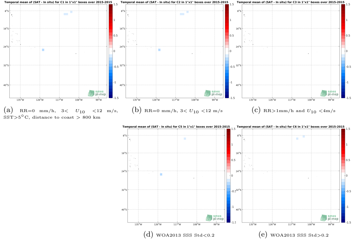
Figure 11: Temporal mean gridded over spatial boxes of size 1^\circ \times 1^\circ of \Delta SSS (Aquarius-L4-IPRC-V5-MONTHLY - Surface drifters) for 5 different subdatasets corresponding to:RR=0 mm/h, 3 < U_{10} < 12 m/s, SST>5°C, distance to coast > 800 km (a), RR=0 mm/h, 3 < U_{10} < 12 m/s (b), RR>1mm/h and U_{10} < 4 m/s (c), WOA2013 SSS Std<0.2 (d), WOA2013 SSS Std>0.2 (e).
