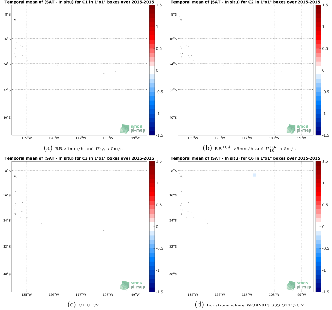
Figure 11: Temporal mean gridded over spatial boxes of size 1^\circ \times 1^\circ of \Delta SSS (Aquarius-L4-IPRC-V5-MONTHLY - Surface drifters) for 4 different subdatasets corresponding to: RR > 1\text{mm/h} and U_{10} < 5\text{m/s} (a), RR^{10d} > 5\text{mm/h} and U_{10}^{10d} < 5\text{m/s} (b), C1 U C2 (c), Locations where WOA2013 SSS STD > 0.2 (d).
