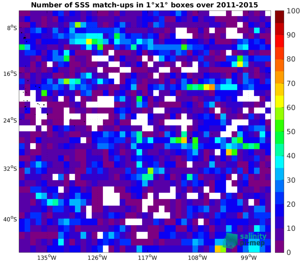
Figure 4: Number of SSS match-ups between Argo SSS and the Aquarius SSS L4 OI v5 - Monthly (IPRC) SSS product for the OTT zone Pi-MEP region over 1^\circ \times 1^\circ boxes and for the full satellite product period.
