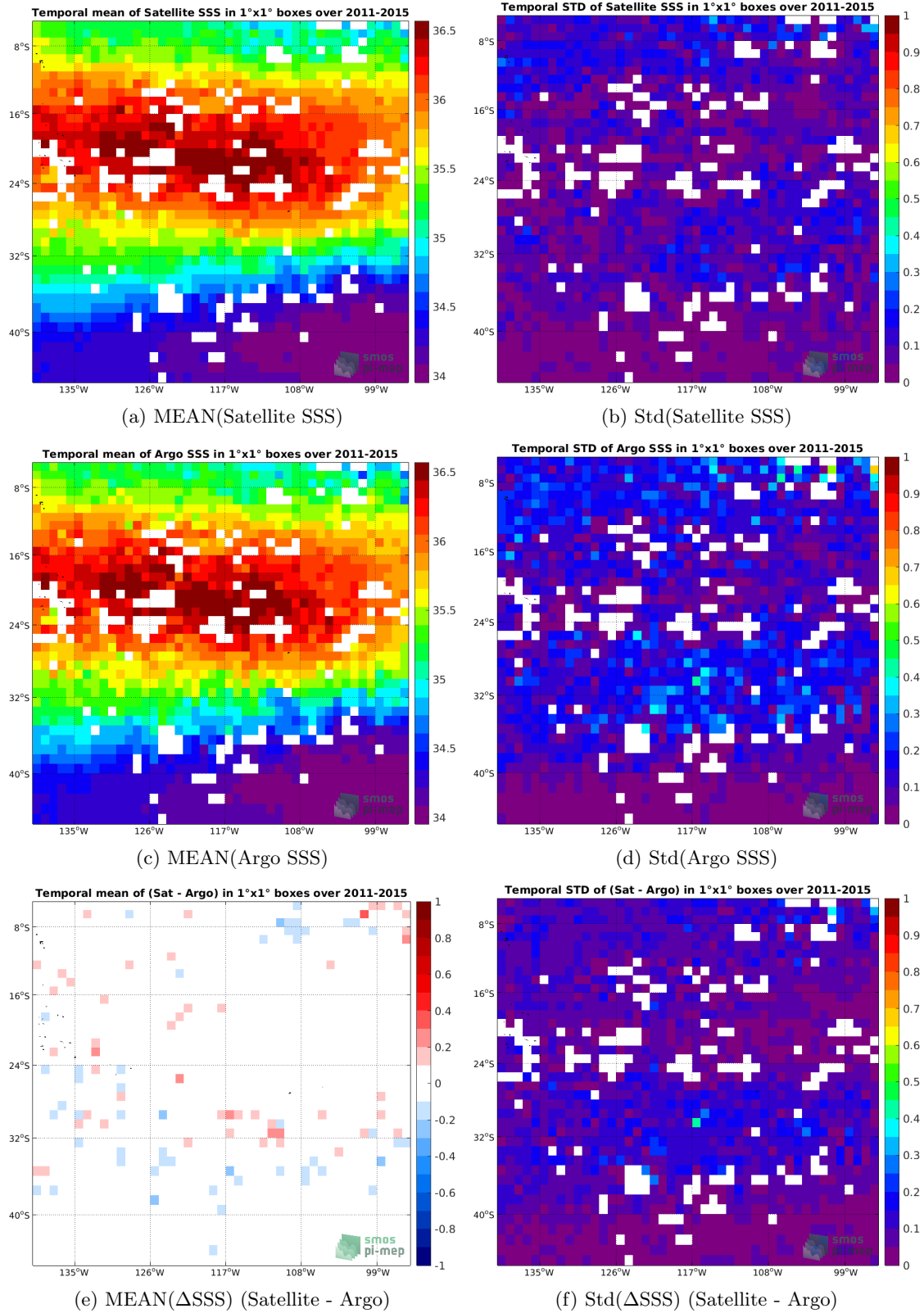
Figure 6: Temporal mean (left) and Std (right) of SSS from Aquarius SSS L4 OI v5 - Monthly (IPRC) (top), Argo (middle), and of \Delta SSS (Satellite - Argo). Only match-up pairs are used to generate these maps.
