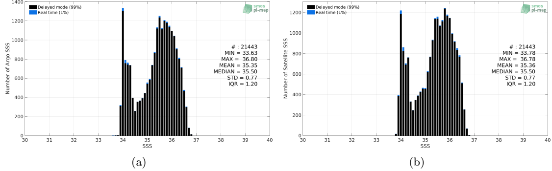
Figure 2: Histograms of SSS from Argo (a) and Aquarius SSS L4 OI v5 - Monthly (IPRC) (b) considering all match-up pairs per bins of 0.1 over the OTT zone Pi-MEP region and for the full satellite product period.
