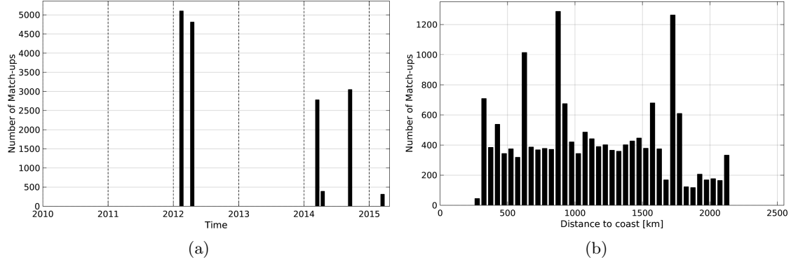
Figure 1: Number of match-ups between TSG-SAMOS and Aquarius-L4-IPRC-V4-MONTHLY SSS as a function of time (a) and as function of the distance to coast (b) over the OTT zone Pi-MEP region and for the full satellite product period.
