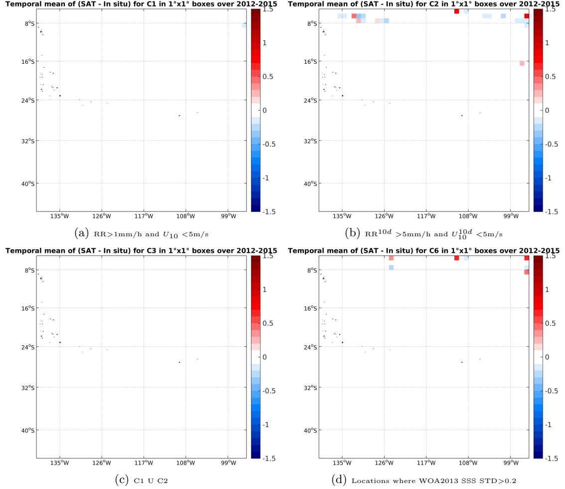
Figure 12: Temporal mean gridded over spatial boxes of size 1^\circ \times 1^\circ of \Delta SSS (Aquarius-L4-IPRC-V4-MONTHLY - TSG-SAMOS) for 4 different subdatasets corresponding to: RR > 1 mm/h and U_{10} < 5 m/s (a), RR^{10d} > 5 mm/h and U_{10}^{10d} < 5 m/s (b), C1 U C2 (c), Locations where WOA2013 SSS STD > 0.2 (d).
