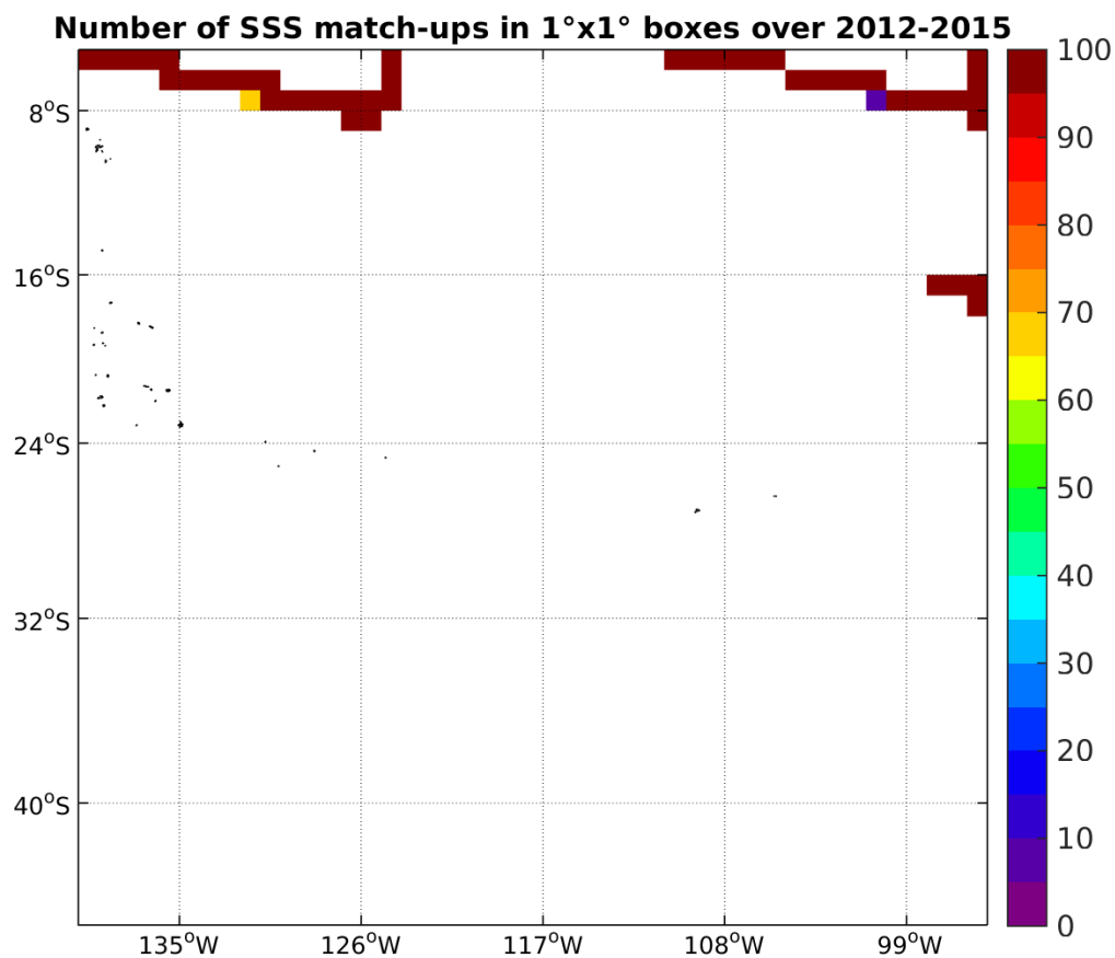
Figure 4: Number of SSS match-ups between TSG-SAMOS SSS and the Aquarius-L4-IPRC-V4-MONTHLY SSS product for the OTT zone Pi-MEP region over 1°x1° boxes and for the full satellite product period.
