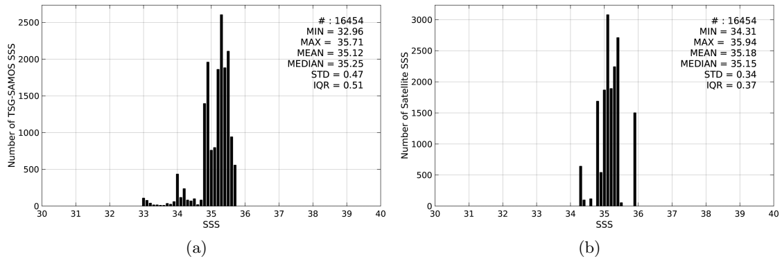
Figure 2: Histograms of SSS from TSG-SAMOS (a) and Aquarius-L4-IPRC-V4-MONTHLY (b) considering all match-up pairs per bins of 0.1 over the OTT zone Pi-MEP region and for the full satellite product period.
