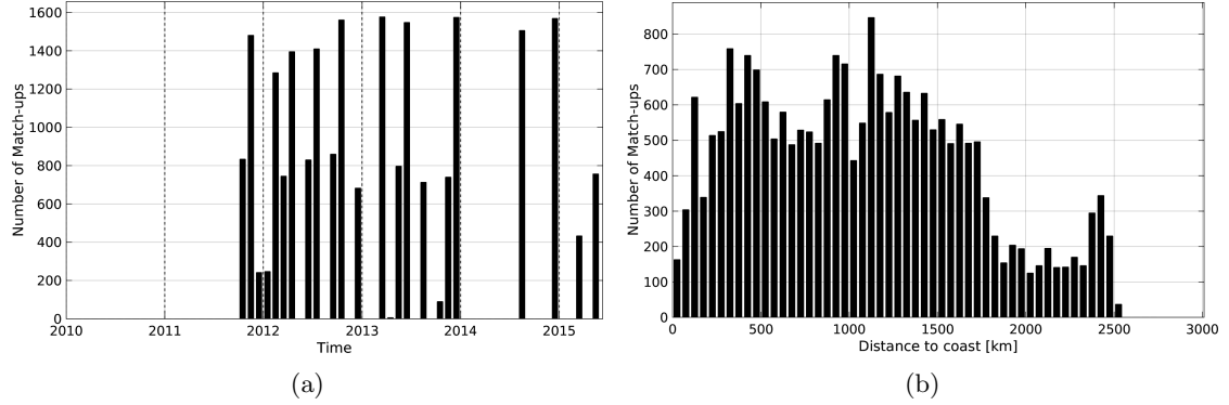
Figure 1: Number of match-ups between TSG-LEGOS-DM and Aquarius-L4-IPRC-V4-MONTHLY SSS as a function of time (a) and as function of the distance to coast (b) over the OTT zone Pi-MEP region and for the full satellite product period.
