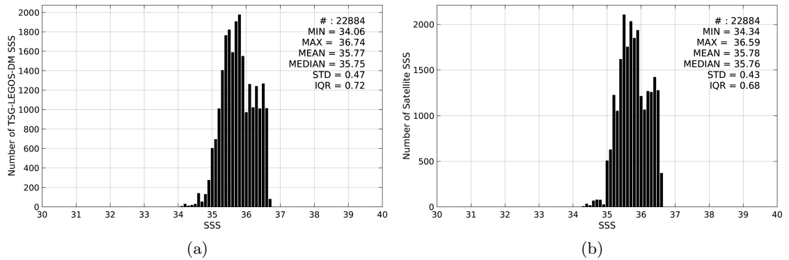
Figure 2: Histograms of SSS from TSG-LEGOS-DM (a) and Aquarius-L4-IPRC-V4-MONTHLY (b) considering all match-up pairs per bins of 0.1 over the OTT zone Pi-MEP region and for the full satellite product period.
