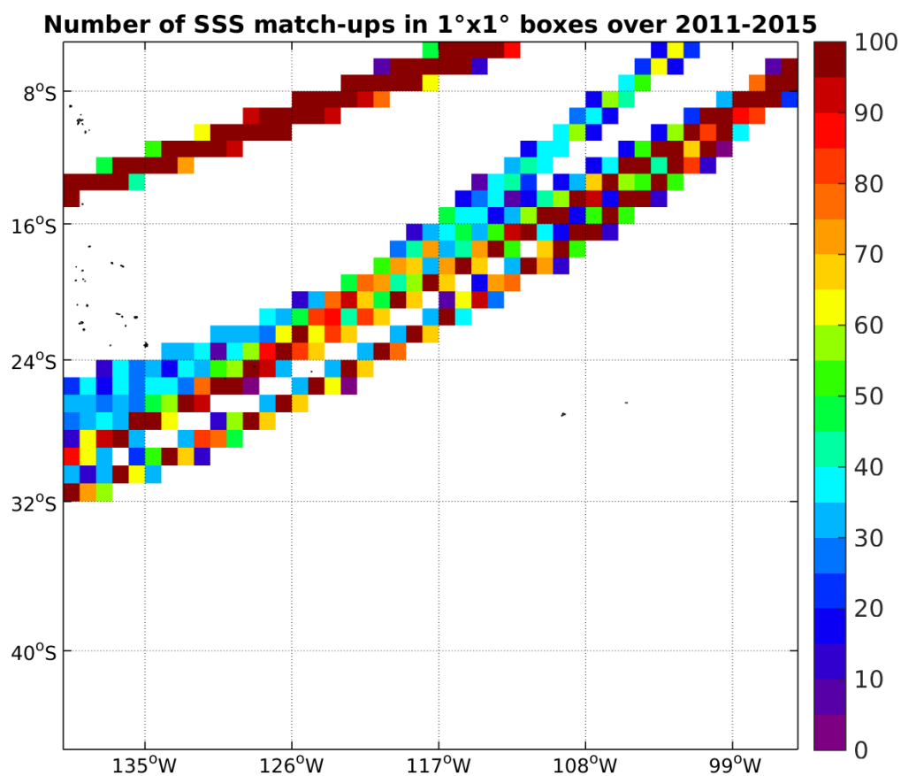
Figure 4: Number of SSS match-ups between TSG-LEGOS-DM SSS and the Aquarius-L4-IPRC-V4-MONTHLY SSS product for the OTT zone Pi-MEP region over 1°x1° boxes and for the full satellite product period.
