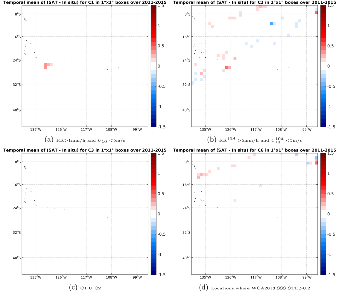
Figure 12: Temporal mean gridded over spatial boxes of size 1^\circ \times 1^\circ of \Delta SSS (Aquarius-L4-IPRC-V4-MONTHLY - TSG-LEGOS-DM) for 4 different subdatasets corresponding to: RR > 1\text{mm/h} and U_{10} < 5\text{m/s} (a), RR^{10d} > 5\text{mm/h} and U_{10}^{10d} < 5\text{m/s} (b), C1 U C2 (c), Locations where WOA2013 SSS STD > 0.2 (d).
