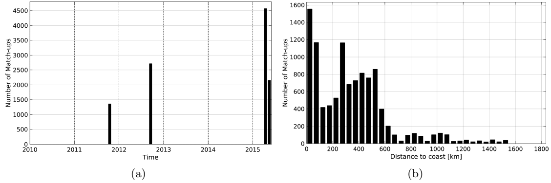
Figure 1: Number of match-ups between TSG-GOSUD-Research-vessel and Aquarius-L4-IPRC-V4-MONTHLY SSS as a function of time (a) and as function of the distance to coast (b) over the OTT zone Pi-MEP region and for the full satellite product period.
