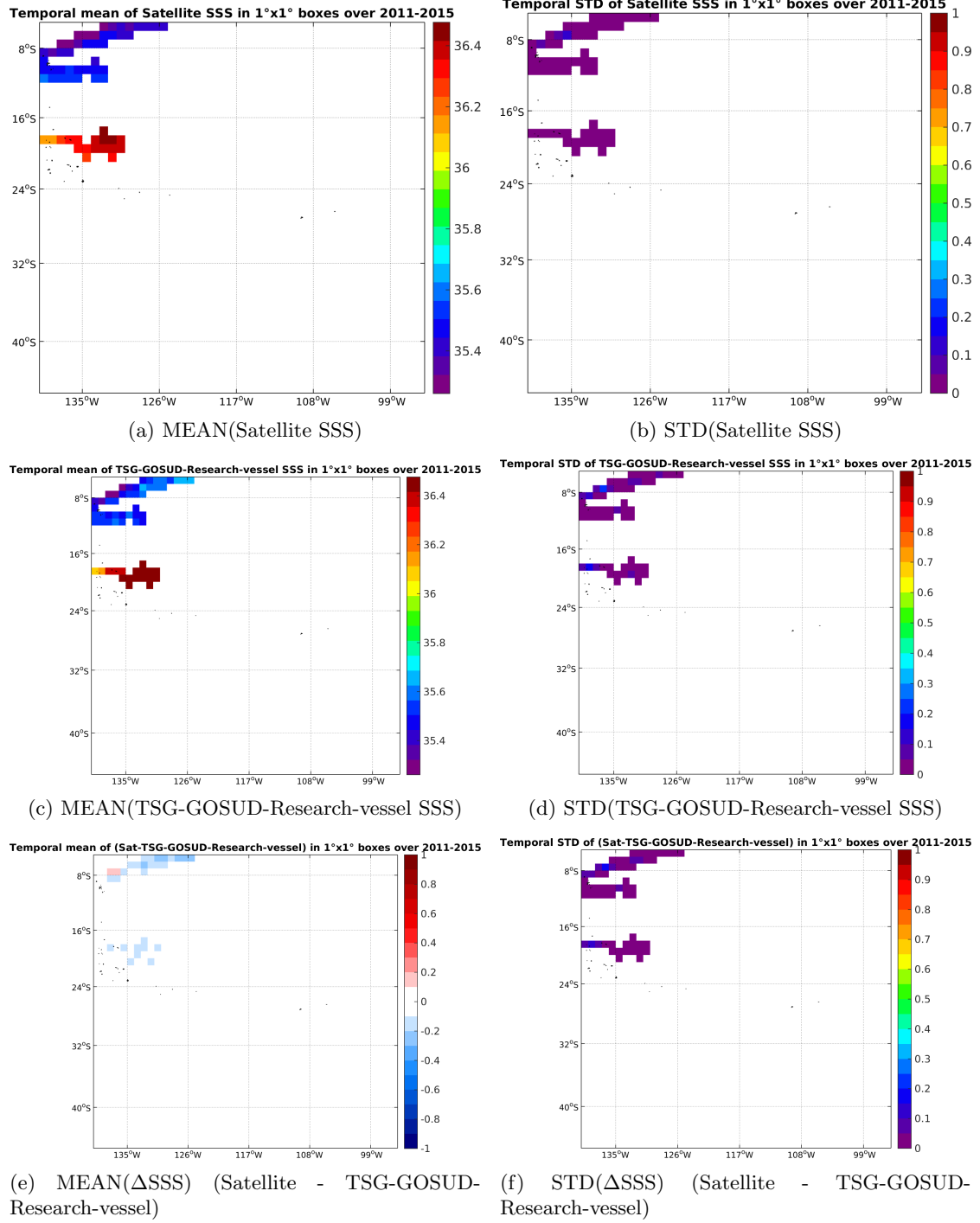
Figure 6: Temporal mean (left) and STD (right) of SSS from Aquarius-L4-IPRC-V4-MONTHLY (top), TSG-GOSUD-Research-vessel (middle), and of \Delta SSS (Satellite - TSG-GOSUD-Research-vessel). Only match-up pairs are used to generate these maps.
