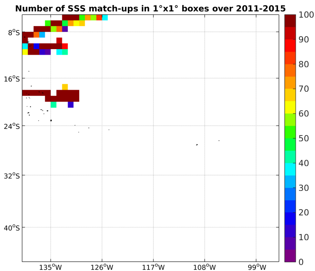
Figure 4: Number of SSS match-ups between TSG-GOSUD-Research-vessel SSS and the Aquarius-L4-IPRC-V4-MONTHLY SSS product for the OTT zone Pi-MEP region over 1°x1° boxes and for the full satellite product period.
