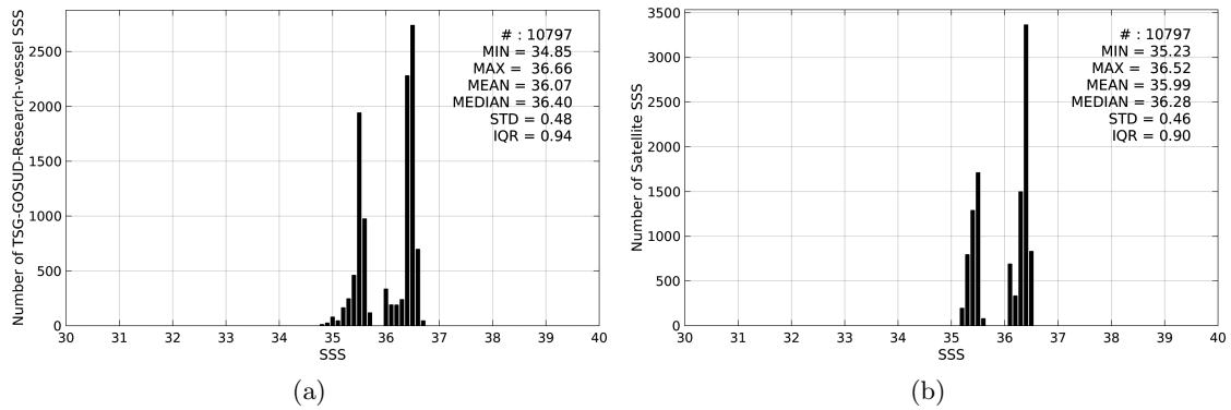
Figure 2: Histograms of SSS from TSG-GOSUD-Research-vessel (a) and Aquarius-L4-IPRC-V4-MONTHLY (b) considering all match-up pairs per bins of 0.1 over the OTT zone Pi-MEP region and for the full satellite product period.
