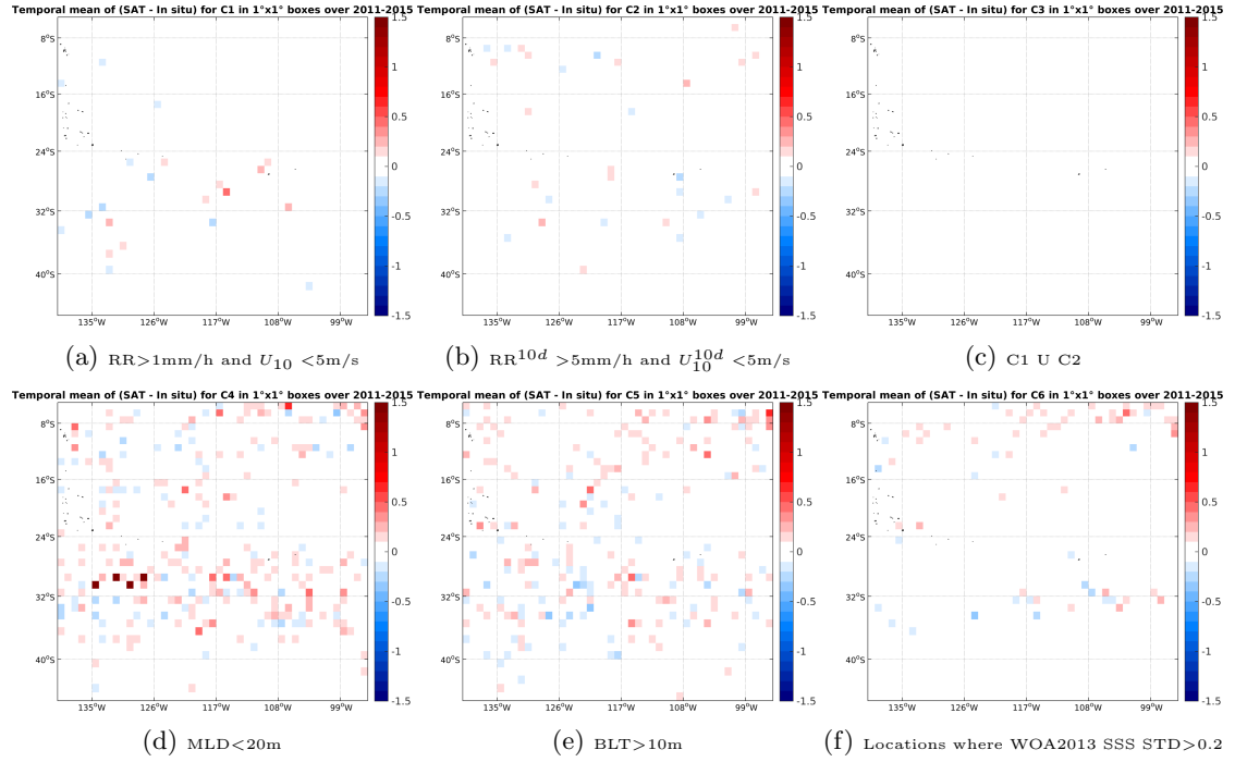
Figure 12: Temporal mean gridded over spatial boxes of size 1^\circ \times 1^\circ of \Delta SSS (Aquarius-L4-IPRC-V4-MONTHLY - Argo) for 6 different subdatasets corresponding to: RR > 1mm/h and U_{10} < 5\text{m/s} (a), RR^{10d} > 5\text{mm/h} and U_{10}^{10d} < 5\text{m/s} (b), C1 U C2 (c), MLD < 20m (d), BLT > 10m (e), Locations where WOA2013 SSS STD > 0.2 (f).
