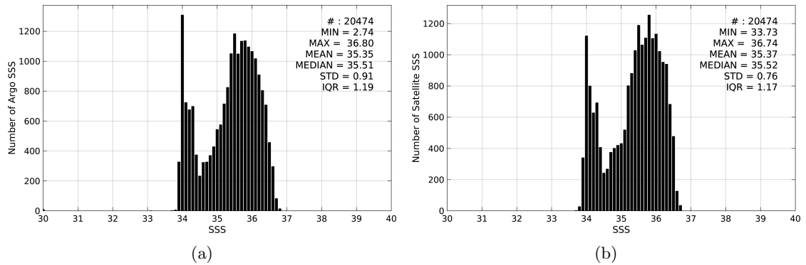
Figure 2: Histograms of SSS from Argo (a) and Aquarius-L4-IPRC-V4-MONTHLY (b) considering all match-up pairs per bins of 0.1 over the OTT zone Pi-MEP region and for the full satellite product period.
