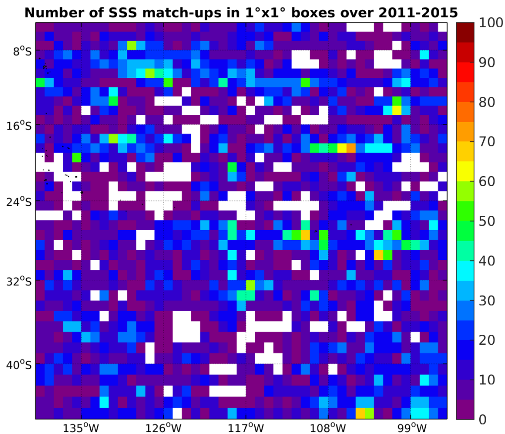
Figure 4: Number of SSS match-ups between Argo SSS and the Aquarius-L4-IPRC-V4-MONTHLY SSS product for the OTT zone Pi-MEP region over 1°x1° boxes and for the full satellite product period.
