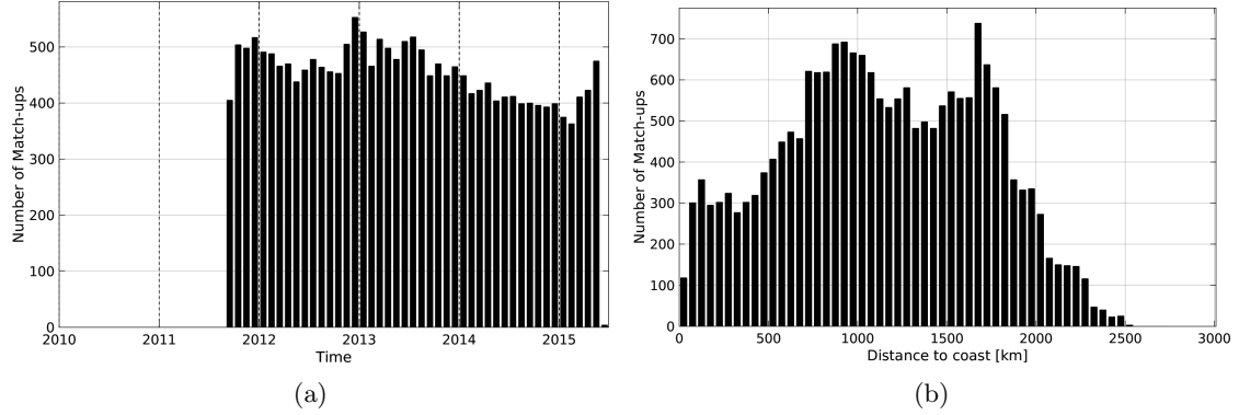
Figure 1: Number of match-ups between Argo and Aquarius-L4-IPRC-V4-MONTHLY SSS as a function of time (a) and as function of the distance to coast (b) over the OTT zone Pi-MEP region and for the full satellite product period.
