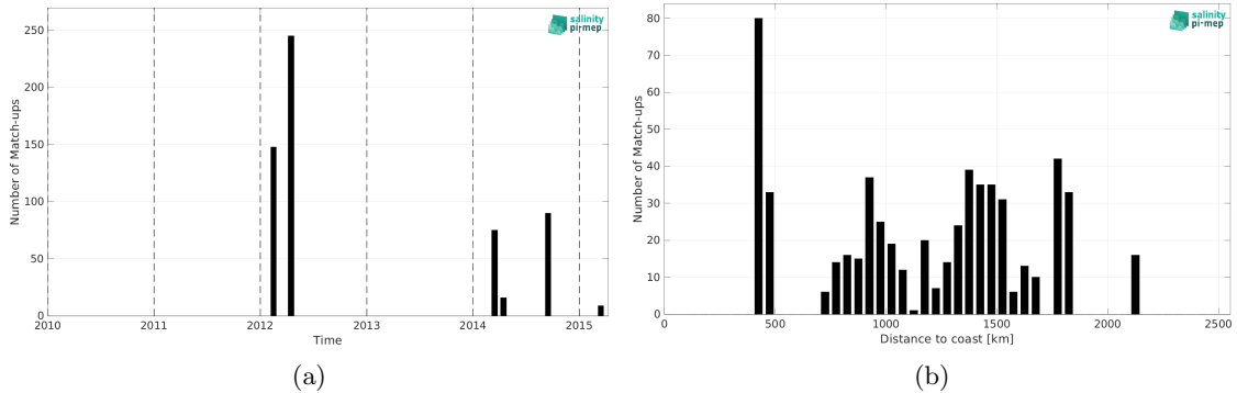
Figure 2: Number of match-ups between TSG (SAMOS) and Aquarius SSS L3 OR v5 - 7-Day running (NASA-GSFC) SSS as a function of time (a) and as function of the distance to coast (b) over the OTT zone Pi-MEP region and for the full satellite product period.
