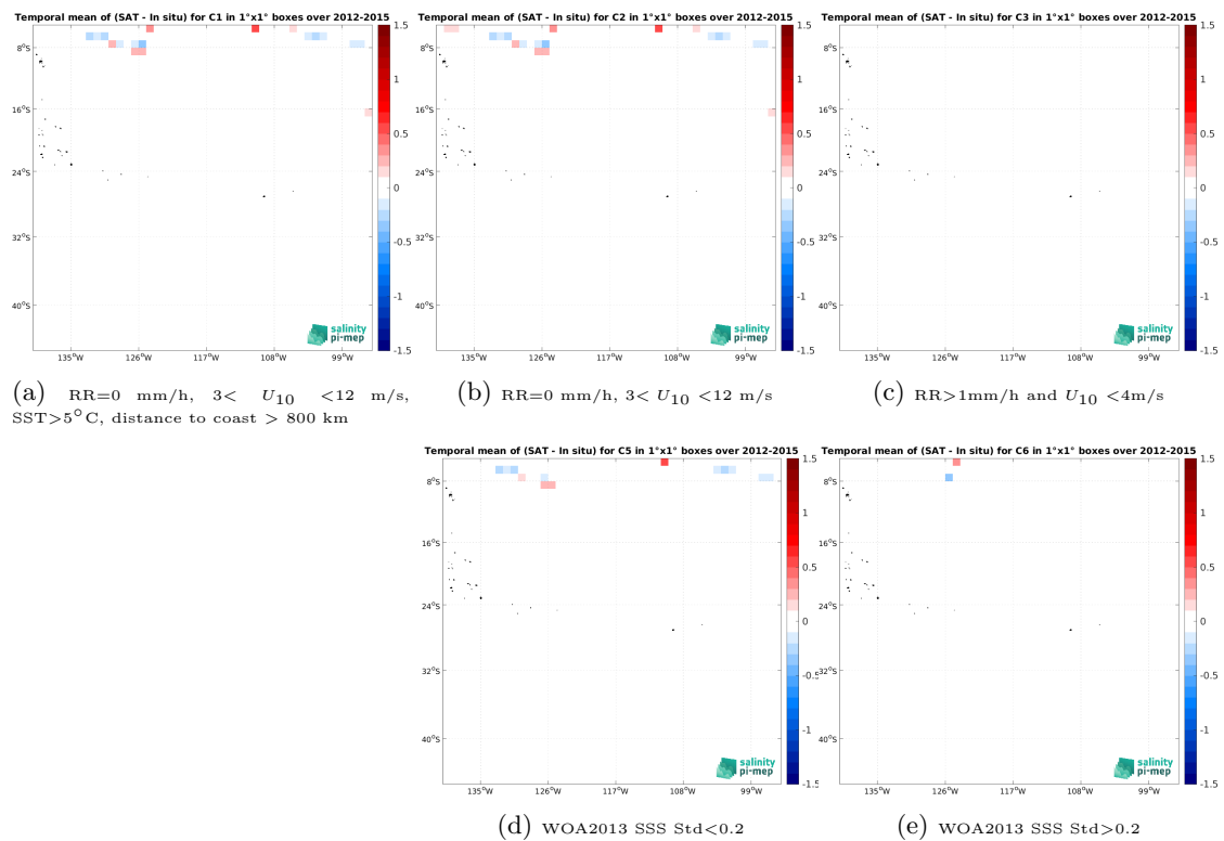
Figure 14: Temporal mean gridded over spatial boxes of size 1^\circ \times 1^\circ of \Delta SSS (Aquarius SSS L3 OR v5 - 7-Day running (NASA-GSFC) - TSG (SAMOS)) for 5 different subdatasets corresponding to: RR=0 mm/h, 3 < U_{10} < 12 m/s, SST > 5^\circ C , distance to coast > 800 km (a), RR=0 mm/h, 3 < U_{10} < 12 m/s (b), RR > 1 mm/h and U_{10} < 4 m/s (c), WOA2013 SSS Std < 0.2 (d), WOA2013 SSS Std > 0.2 (e).
