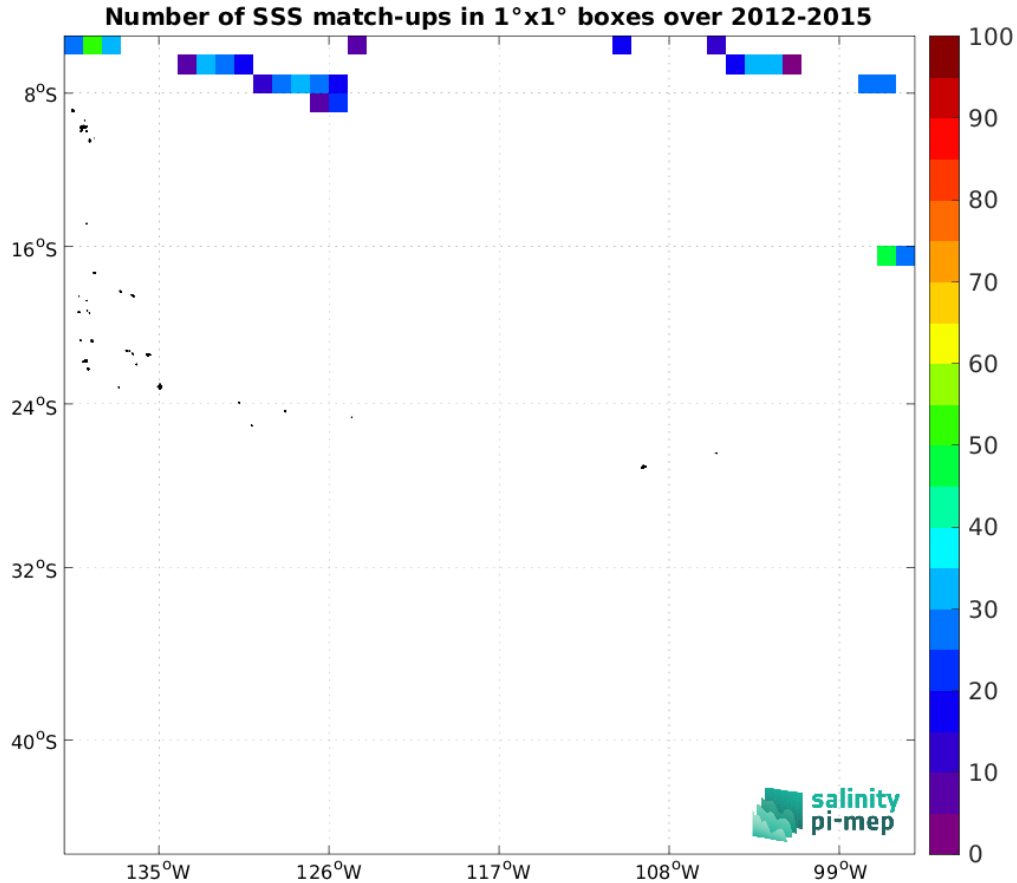
Figure 5: Number of SSS match-ups between TSG (SAMOS) SSS and the Aquarius SSS L3 OR v5 - 7-Day running (NASA-GSFC) SSS product for the OTT zone Pi-MEP region over 1^\circ \times 1^\circ boxes and for the full satellite product period.
