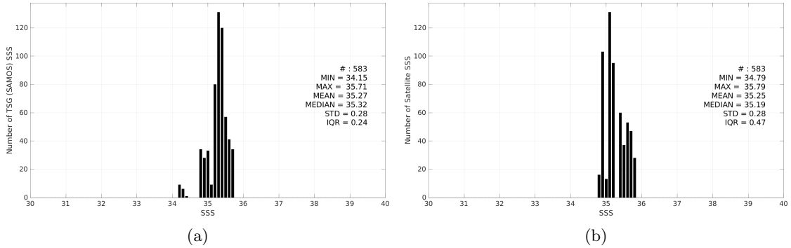
Figure 3: Histograms of SSS from TSG (SAMOS) (a) and Aquarius SSS L3 OR v5 - 7-Day running (NASA-GSFC) (b) considering all match-up pairs per bins of 0.1 over the OTT zone Pi-MEP region and for the full satellite product period.
