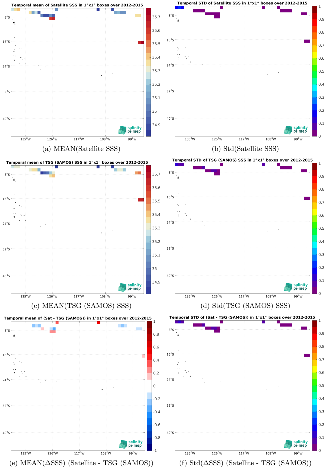
Figure 7: Temporal mean (left) and Std (right) of SSS from Aquarius SSS L3 OR v5 - 7-Day running (NASA-GSFC) (top), TSG (SAMOS) (middle), and of \Delta SSS (Satellite - TSG (SAMOS)). Only match-up pairs are used to generate these maps.
