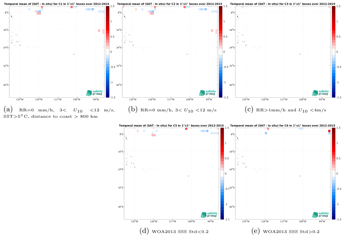
Figure 12: Temporal mean gridded over spatial boxes of size 1^\circ \times 1^\circ of \Delta SSS (Aquarius SSS L3 OR v5 - 7-Day running (NASA-GSFC) - TSG (SAMOS)) for 5 different subdatasets corresponding to: RR=0 mm/h, 3 < U_{10} < 12 m/s, SST > 5^\circ C , distance to coast > 800 km (a), RR=0 mm/h, 3 < U_{10} < 12 m/s (b), RR > 1 mm/h and U_{10} < 4 m/s (c), WOA2013 SSS Std < 0.2 (d), WOA2013 SSS Std > 0.2 (e).
