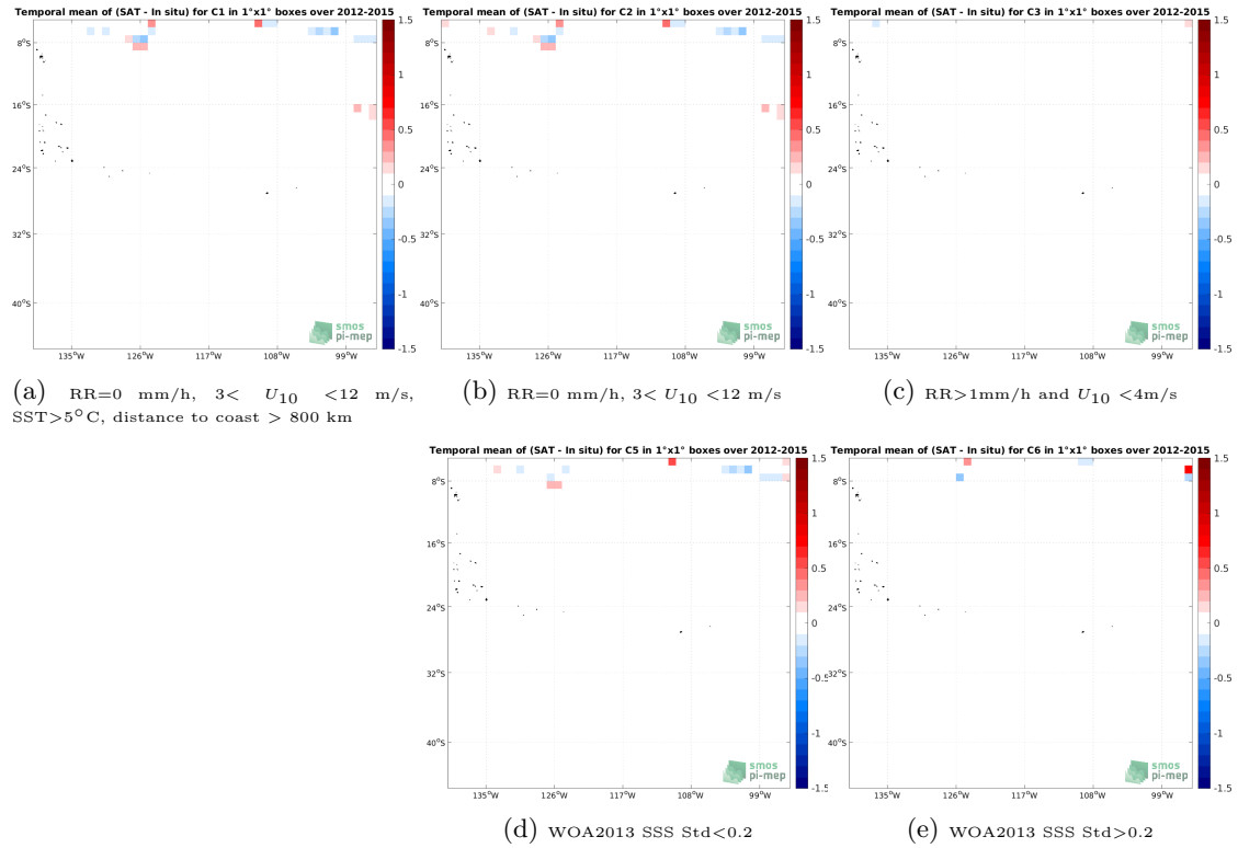
Figure 12: Temporal mean gridded over spatial boxes of size 1^\circ \times 1^\circ of \Delta SSS (Aquarius SSS L3 OR v5 - 7-Day running (NASA-GSFC) - TSG (SAMOS)) for 5 different subdatasets corresponding to: RR=0 mm/h, 3 < U_{10} < 12 m/s, SST > 5^\circ C , distance to coast > 800 km (a), RR=0 mm/h, 3 < U_{10} < 12 m/s (b), RR > 1 mm/h and U_{10} < 4 m/s (c), WOA2013 SSS Std < 0.2 (d), WOA2013 SSS Std > 0.2 (e).
