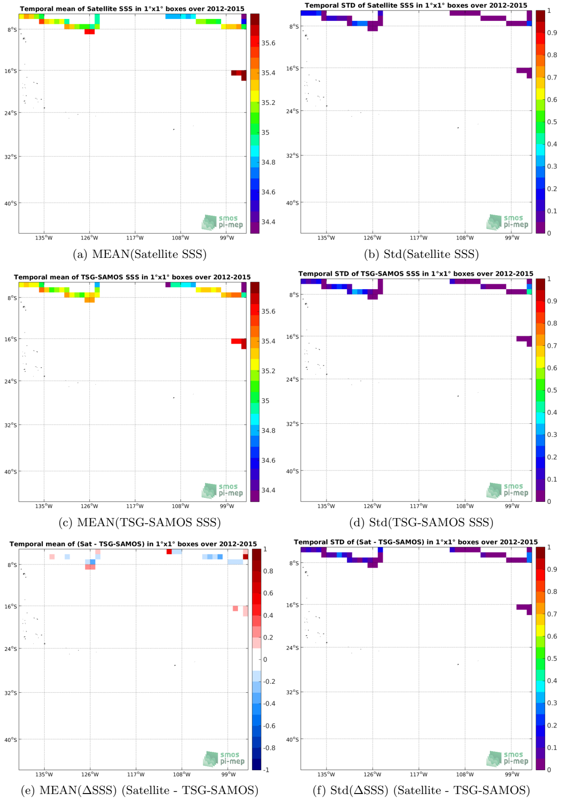
Figure 6: Temporal mean (left) and Std (right) of SSS from Aquarius-L3-OR-V5-7DAY-RUNNING-1DEG (top), TSG-SAMOS (middle), and of \Delta SSS (Satellite - TSG-SAMOS). Only match-up pairs are used to generate these maps.
