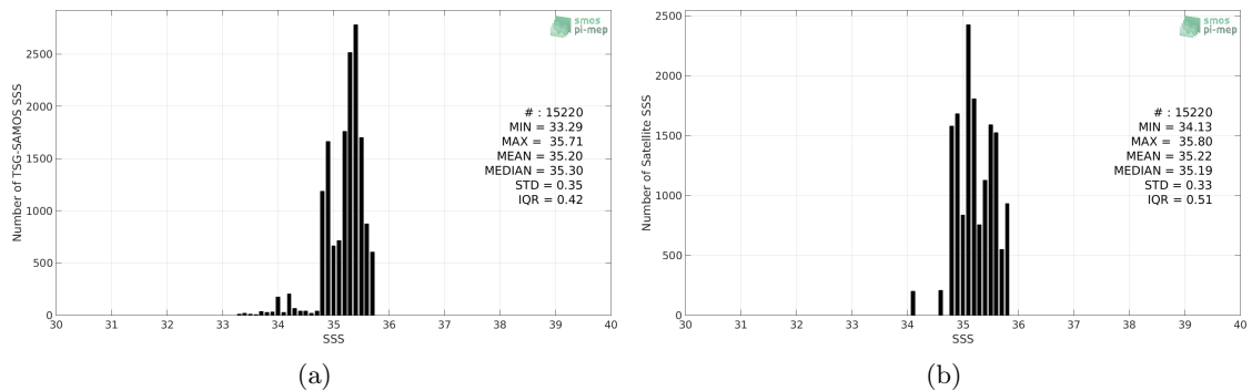
Figure 2: Histograms of SSS from TSG-SAMOS (a) and Aquarius-L3-OR-V5-7DAY-RUNNING-1DEG (b) considering all match-up pairs per bins of 0.1 over the OTT zone Pi-MEP region and for the full satellite product period.
