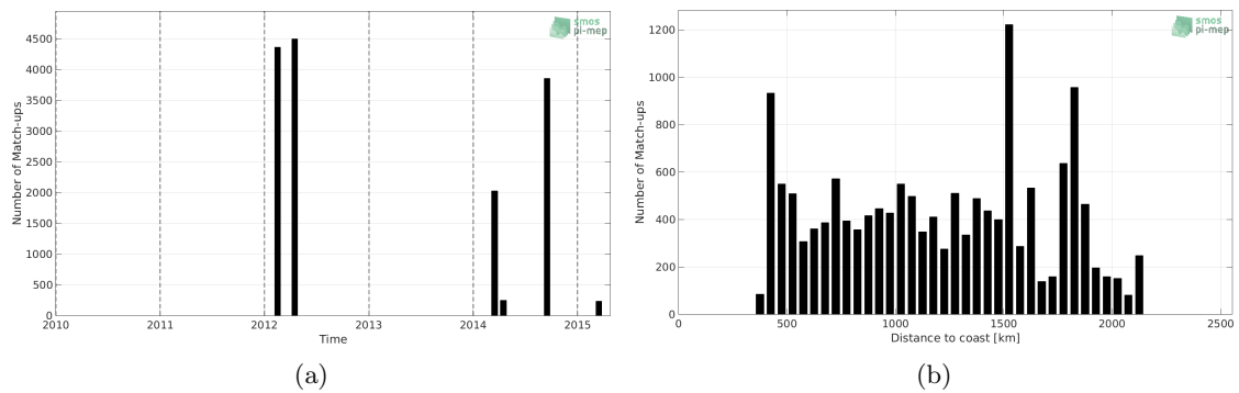
Figure 1: Number of match-ups between TSG-SAMOS and Aquarius-L3-OR-V5-7DAY-RUNNING-1DEG SSS as a function of time (a) and as function of the distance to coast (b) over the OTT zone Pi-MEP region and for the full satellite product period.
