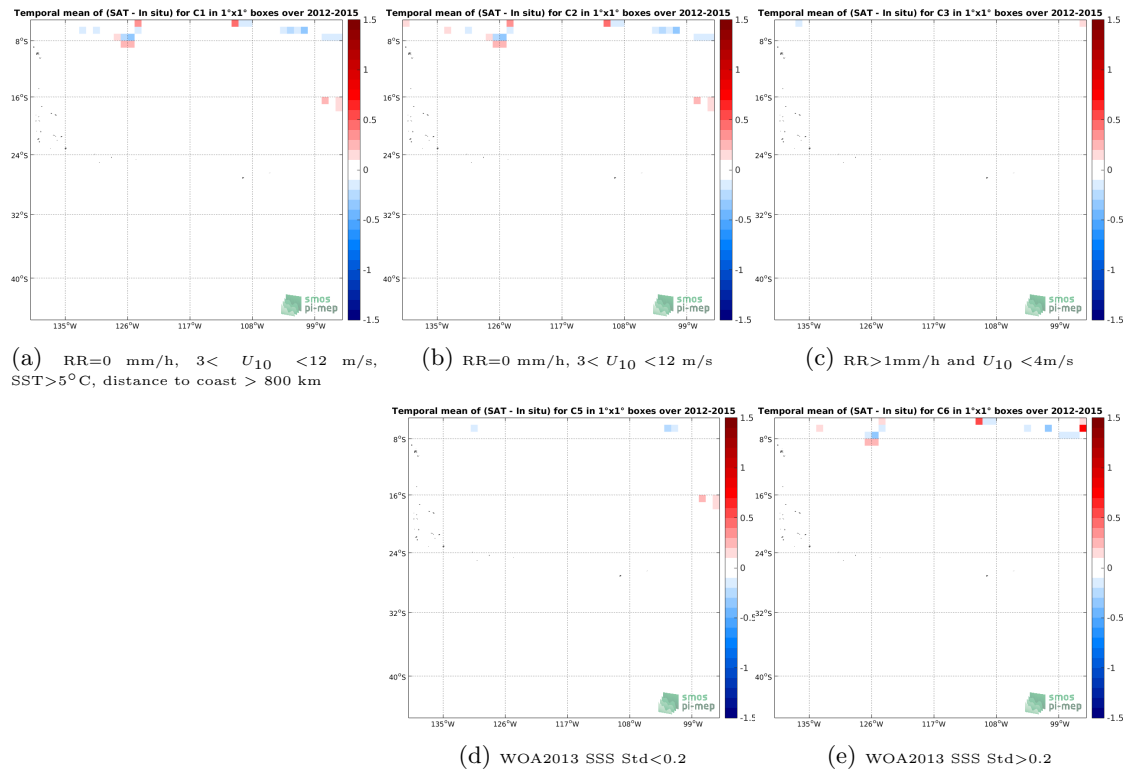
Figure 12: Temporal mean gridded over spatial boxes of size 1^\circ \times 1^\circ of \Delta SSS (Aquarius-L3-OR-V5-7DAY-RUNNING-1DEG - TSG-SAMOS) for 5 different subdatasets corresponding to:RR=0 mm/h, 3 < U_{10} < 12 m/s, SST >5^\circ\text{C} , distance to coast > 800 km (a), RR=0 mm/h, 3 < U_{10} < 12 m/s (b), RR >1 mm/h and U_{10} < 4 m/s (c), WOA2013 SSS Std <0.2 (d), WOA2013 SSS Std >0.2 (e).
