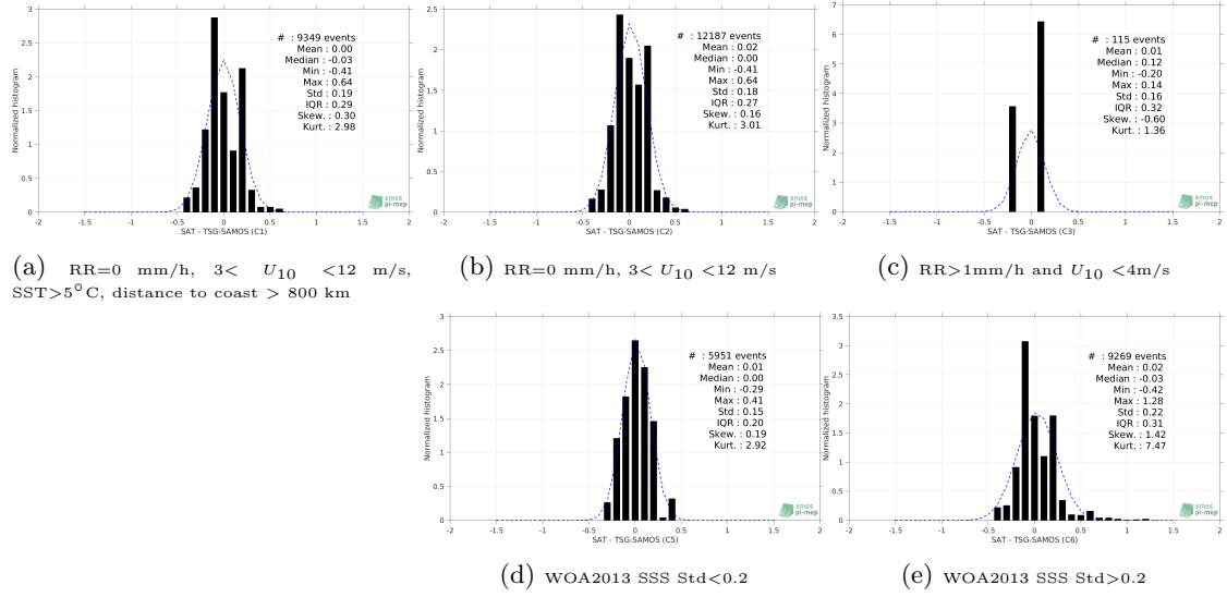
Figure 13: Normalized histogram of \Delta\text{SSS} (Aquarius-L3-OR-V5-7DAY-RUNNING-1DEG - TSG-SAMOS) for 5 different subdatasets corresponding to: RR=0 mm/h, 3 < U_{10} < 12 m/s, SST > 5^{\circ}\text{C} , distance to coast > 800 km (a), RR=0 mm/h, 3 < U_{10} < 12 m/s (b), RR > 1\text{mm/h} and U_{10} < 4\text{m/s} (c), WOA2013 SSS Std < 0.2 (d), WOA2013 SSS Std > 0.2 (e).
