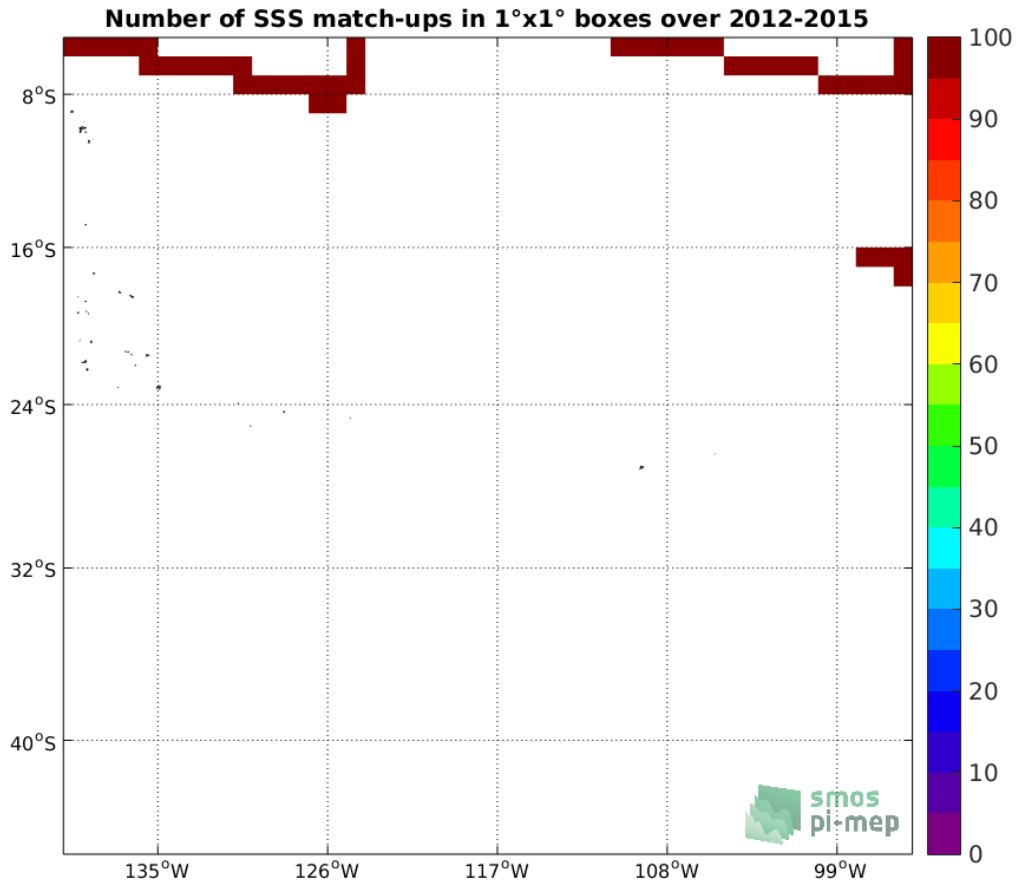
Figure 4: Number of SSS match-ups between TSG-SAMOS SSS and the Aquarius-L3-OR-V5-7DAY-RUNNING-1DEG SSS product for the OTT zone Pi-MEP region over 1°x1° boxes and for the full satellite product period.
