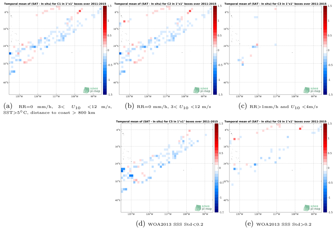
Figure 12: Temporal mean gridded over spatial boxes of size 1^\circ \times 1^\circ of \Delta SSS (Aquarius-L3-OR-V5-7DAY-RUNNING-1DEG - TSG-LEGOS-DM) for 5 different subdatasets corresponding to:RR=0 mm/h, 3 < U_{10} < 12 m/s, SST >5^\circ C, distance to coast > 800 km (a), RR=0 mm/h, 3 < U_{10} < 12 m/s (b), RR >1 mm/h and U_{10} < 4 m/s (c), WOA2013 SSS Std <0.2 (d), WOA2013 SSS Std >0.2 (e).
