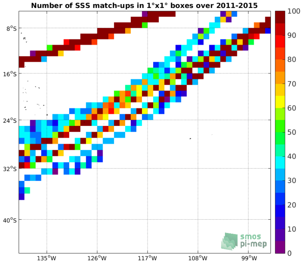
Figure 4: Number of SSS match-ups between TSG-LEGOS-DM SSS and the Aquarius-L3-OR-V5-7DAY-RUNNING-1DEG SSS product for the OTT zone Pi-MEP region over 1°x1° boxes and for the full satellite product period.
