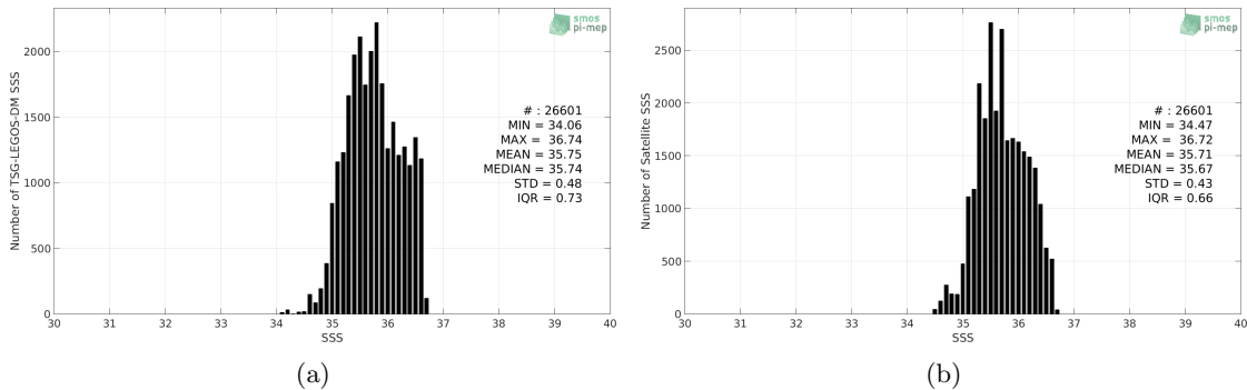
Figure 2: Histograms of SSS from TSG-LEGOS-DM (a) and Aquarius-L3-OR-V5-7DAY-RUNNING-1DEG (b) considering all match-up pairs per bins of 0.1 over the OTT zone Pi-MEP region and for the full satellite product period.
