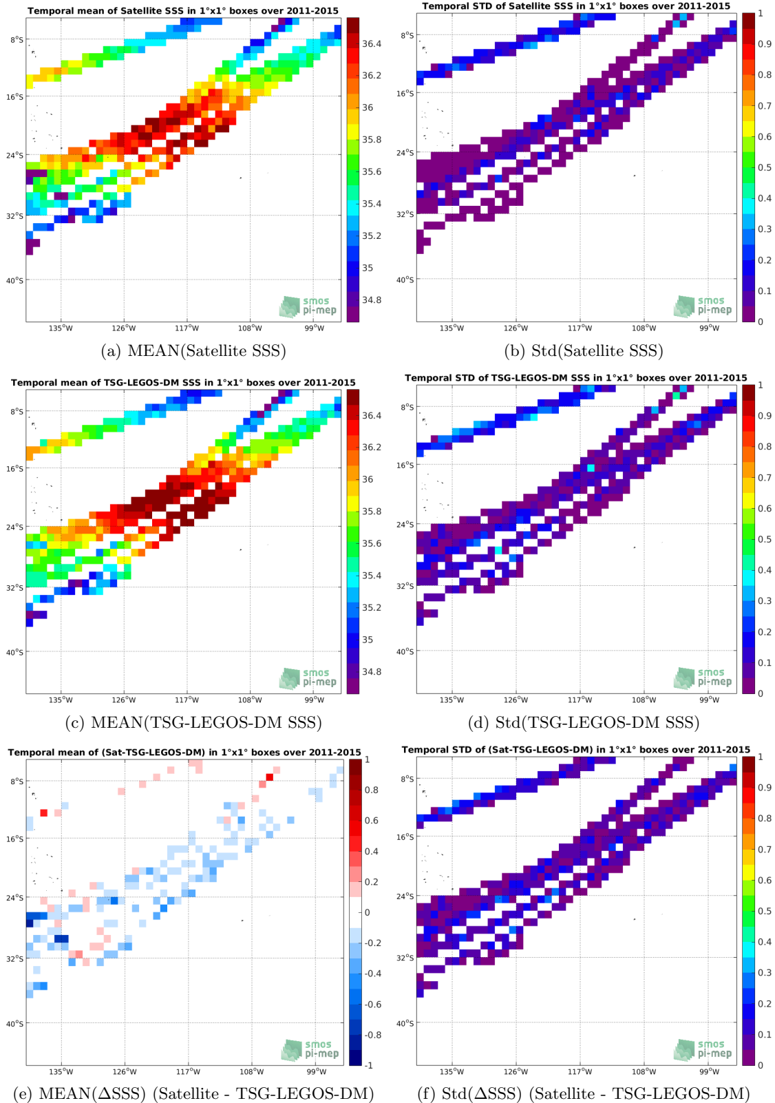
Figure 6: Temporal mean (left) and Std (right) of SSS from Aquarius-L3-OR-V5-7DAY-RUNNING-1DEG (top), TSG-LEGOS-DM (middle), and of \Delta SSS (Satellite - TSG-LEGOS-DM). Only match-up pairs are used to generate these maps.
