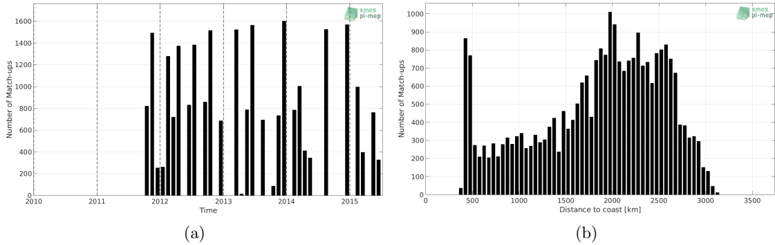
Figure 1: Number of match-ups between TSG-LEGOS-DM and Aquarius-L3-OR-V5-7DAY-RUNNING-1DEG SSS as a function of time (a) and as function of the distance to coast (b) over the OTT zone Pi-MEP region and for the full satellite product period.
