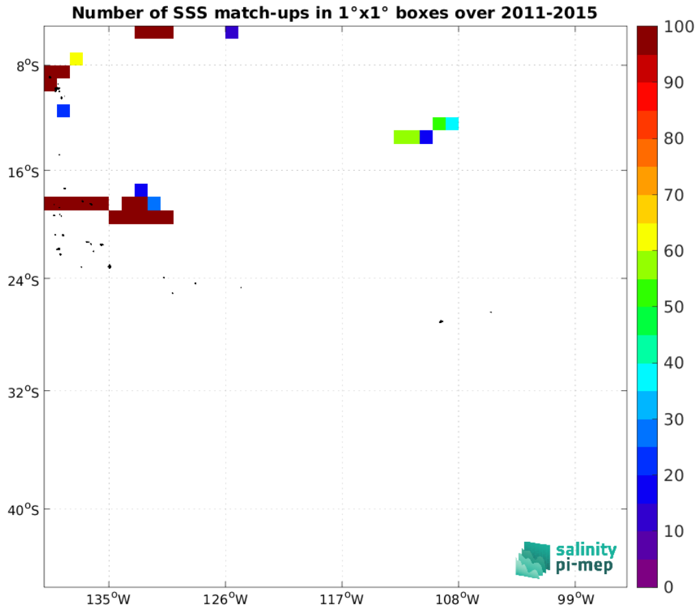
Figure 5: Number of SSS match-ups between TSG (GOSUD-Research-vessel) SSS and the Aquarius SSS L3 OR v5 - 7-Day running (NASA-GSFC) SSS product for the OTT zone Pi-MEP region over 1^\circ \times 1^\circ boxes and for the full satellite product period.
