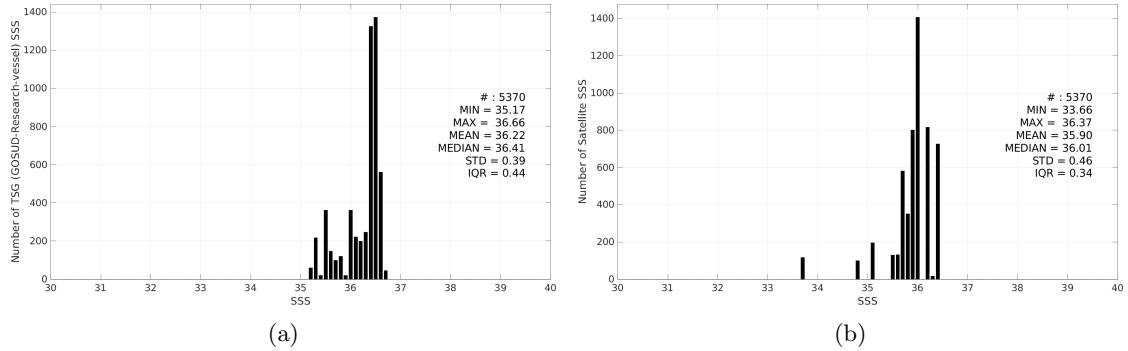
Figure 3: Histograms of SSS from TSG (GOSUD-Research-vessel) (a) and Aquarius SSS L3 OR v5 - 7-Day running (NASA-GSFC) (b) considering all match-up pairs per bins of 0.1 over the OTT zone Pi-MEP region and for the full satellite product period.
