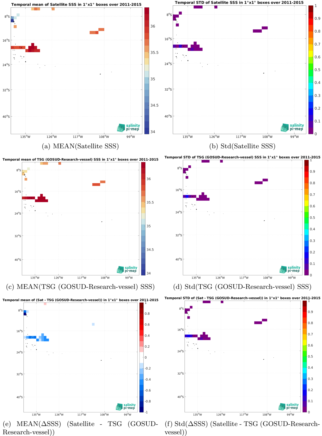
Figure 7: Temporal mean (left) and Std (right) of SSS from Aquarius SSS L3 OR v5 - 7-Day running (NASA-GSFC) (top), TSG (GOSUD-Research-vessel) (middle), and of \Delta SSS (Satellite - TSG (GOSUD-Research-vessel)). Only match-up pairs are used to generate these maps.
