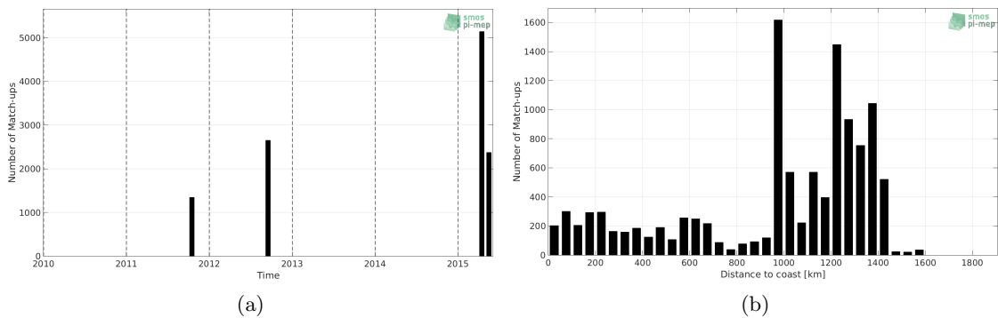
Figure 1: Number of match-ups between TSG-GOSUD-Research-vessel and Aquarius-L3-OR-V5-7DAY-RUNNING-1DEG SSS as a function of time (a) and as function of the distance to coast (b) over the OTT zone Pi-MEP region and for the full satellite product period.
