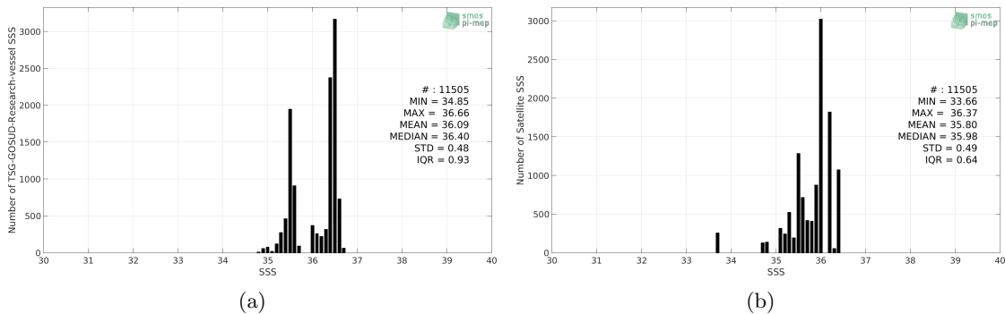
Figure 2: Histograms of SSS from TSG-GOSUD-Research-vessel (a) and Aquarius-L3-OR-V5-7DAY-RUNNING-1DEG (b) considering all match-up pairs per bins of 0.1 over the OTT zone Pi-MEP region and for the full satellite product period.
