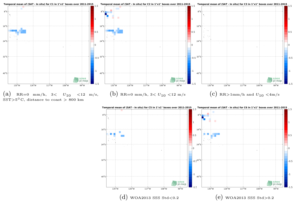
Figure 12: Temporal mean gridded over spatial boxes of size 1^\circ \times 1^\circ of \Delta SSS (Aquarius-L3-OR-V5-7DAY-RUNNING-1DEG - TSG-GOSUD-Research-vessel) for 5 different subdatasets corresponding to:RR=0 mm/h, 3 < U_{10} < 12 m/s, SST >5^\circ\text{C} , distance to coast > 800 km (a), RR=0 mm/h, 3 < U_{10} < 12 m/s (b), RR >1 mm/h and U_{10} < 4 m/s (c), WOA2013 SSS Std <0.2 (d), WOA2013 SSS Std >0.2 (e).
