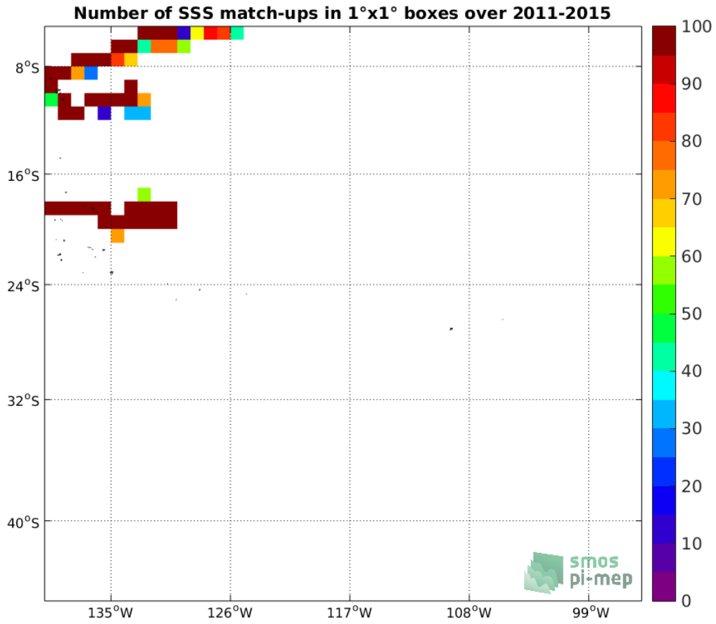
Figure 4: Number of SSS match-ups between TSG-GOSUD-Research-vessel SSS and the Aquarius-L3-OR-V5-7DAY-RUNNING-1DEG SSS product for the OTT zone Pi-MEP region over 1°x1° boxes and for the full satellite product period.
