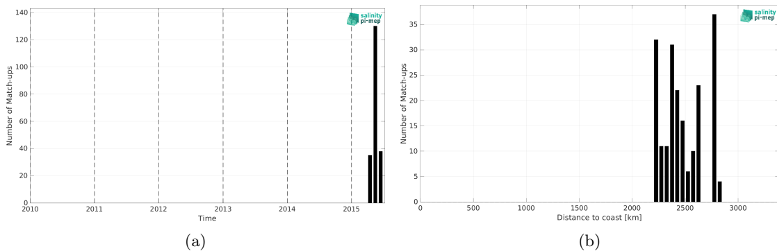
Figure 2: Number of match-ups between Surface drifters and Aquarius SSS L3 OR v5 - 7-Day running (NASA-GSFC) SSS as a function of time (a) and as function of the distance to coast (b) over the OTT zone Pi-MEP region and for the full satellite product period.
