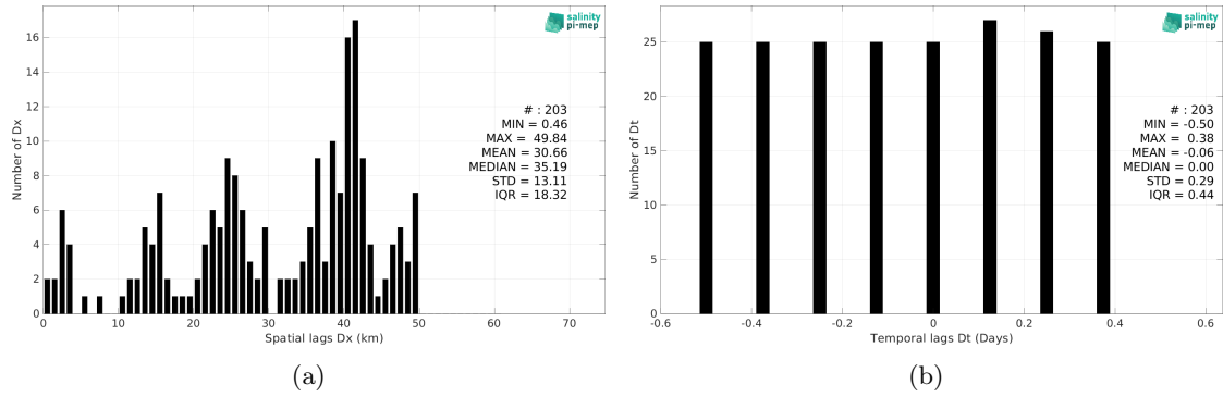
Figure 5: Histograms of the spatial (a) and temporal (b) lags between the location/time of the Surface drifters measurement and the date of the corresponding Aquarius SSS L3 OR v5 - 7-Day running (NASA-GSFC) SSS pixel.
