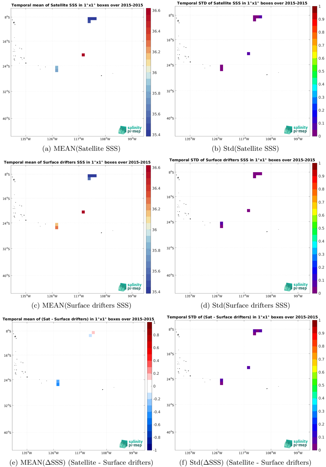
Figure 6: Temporal mean (left) and Std (right), of SSS from Aquarius SSS L3 OR v5 - 7-Day running (NASA-GSFC) (top), Surface drifters (middle), and of \Delta SSS (Satellite - Surface drifters). Only match-up pairs are used to generate these maps.
