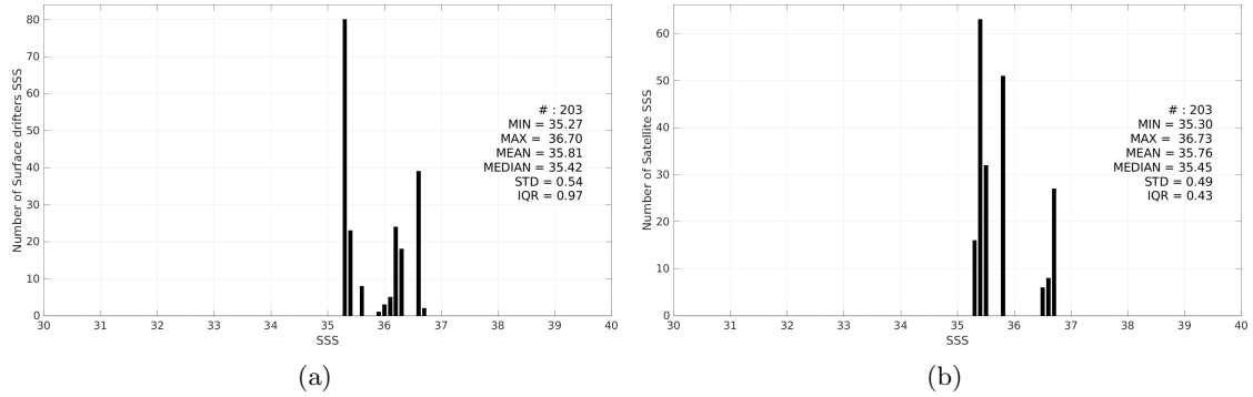
Figure 3: Histograms of SSS from Surface drifters (a) and Aquarius SSS L3 OR v5 - 7-Day running (NASA-GSFC) (b) considering all match-up pairs per bins of 0.1 over the OTT zone Pi-MEP region and for the full satellite product period.
