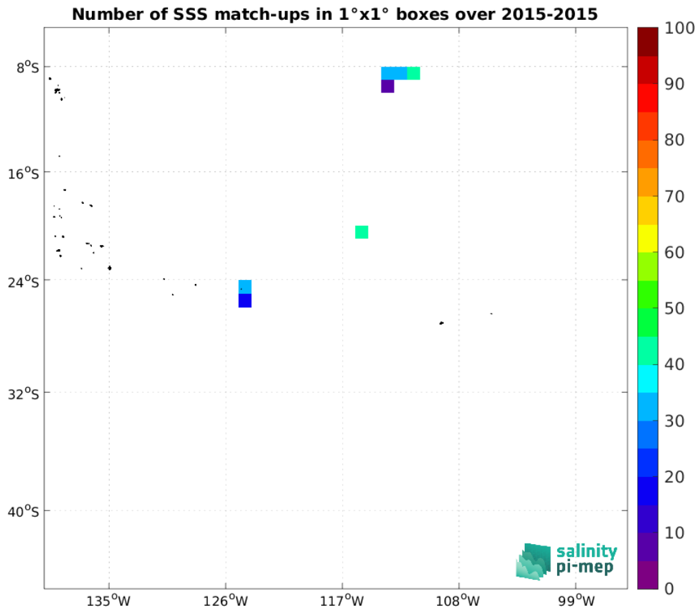
Figure 4: Number of SSS match-ups between Surface drifters SSS and the Aquarius SSS L3 OR v5 - 7-Day running (NASA-GSFC) SSS product for the OTT zone Pi-MEP region over 1°x1° boxes and for the full satellite product period.
