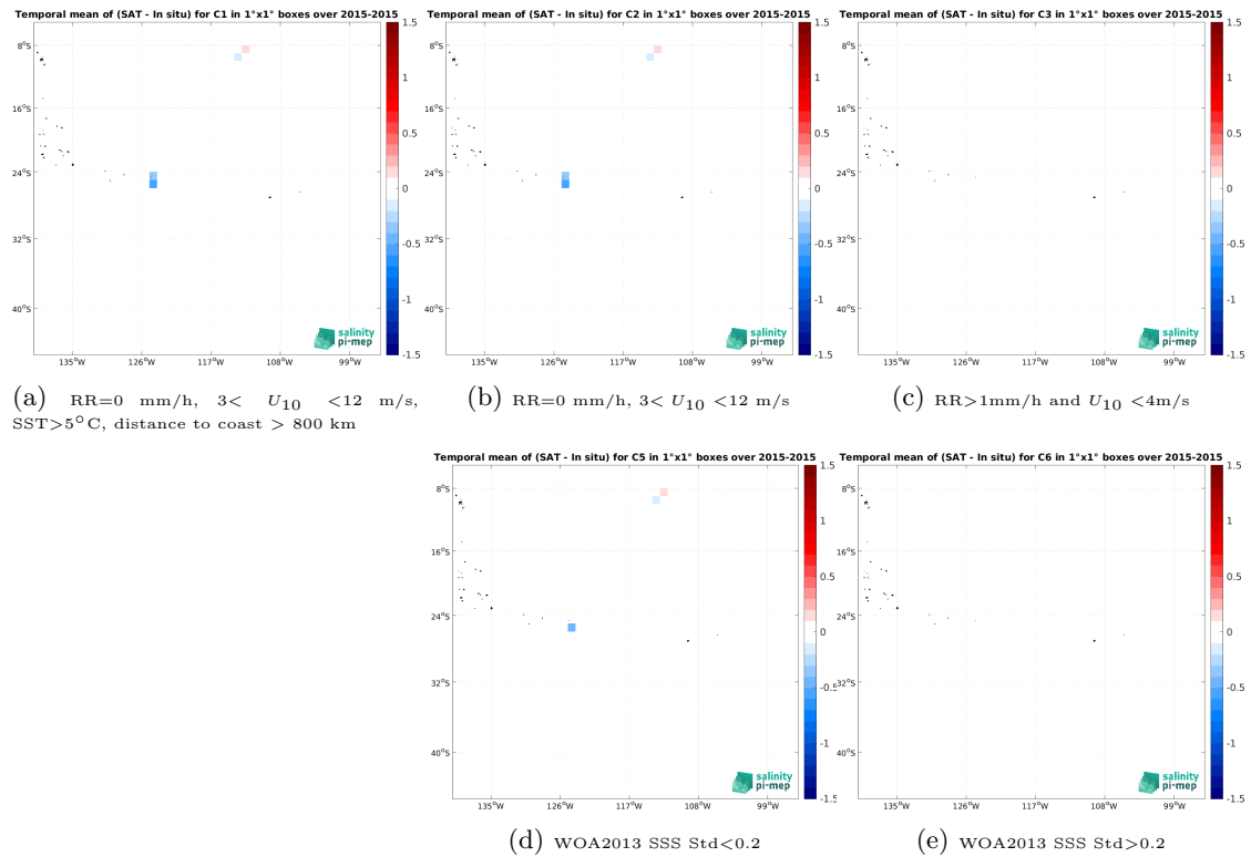
Figure 13: Temporal mean gridded over spatial boxes of size 1^\circ \times 1^\circ of \Delta SSS (Aquarius SSS L3 OR v5 - 7-Day running (NASA-GSFC) - Surface drifters) for 5 different subdatasets corresponding to: RR=0 mm/h, 3 < U_{10} < 12 m/s, SST > 5^\circ C , distance to coast > 800 km (a), RR=0 mm/h, 3 < U_{10} < 12 m/s (b), RR > 1 mm/h and U_{10} < 4 m/s (c), WOA2013 SSS Std < 0.2 (d), WOA2013 SSS Std > 0.2 (e).
