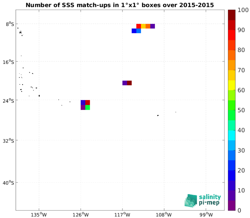
Figure 3: Number of SSS match-ups between Surface drifters SSS and the Aquarius SSS L3 OR v5 - 7-Day running (NASA-GSFC) SSS product for the OTT zone Pi-MEP region over 1°x1° boxes and for the full satellite product period.
