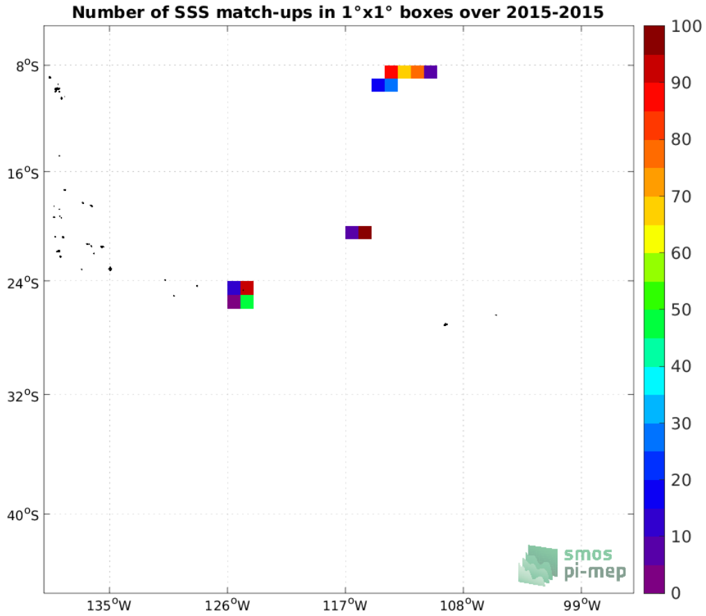
Figure 3: Number of SSS match-ups between Surface drifters SSS and the Aquarius SSS L3 OR v5 - 7-Day running (NASA-GSFC) SSS product for the OTT zone Pi-MEP region over 1^\circ \times 1^\circ boxes and for the full satellite product period.
