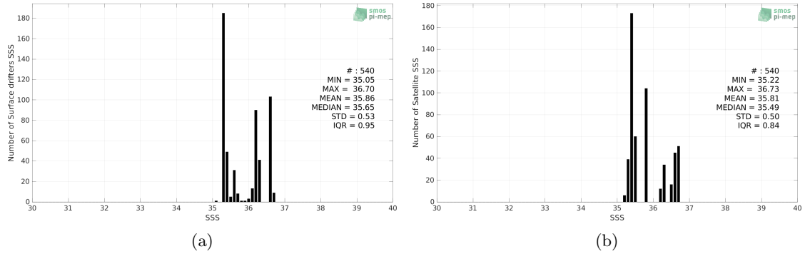
Figure 2: Histograms of SSS from Surface drifters (a) and Aquarius SSS L3 OR v5 - 7-Day running (NASA-GSFC) (b) considering all match-up pairs per bins of 0.1 over the OTT zone Pi-MEP region and for the full satellite product period.
