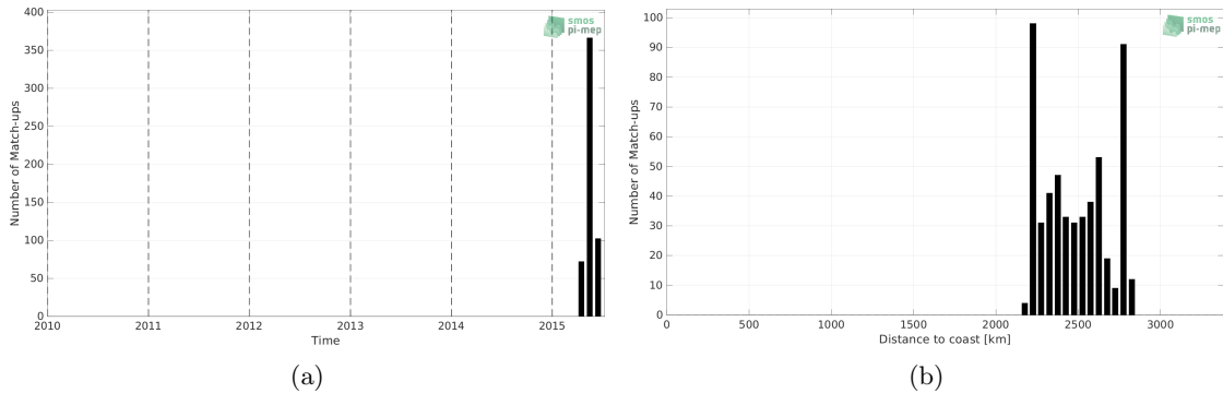
Figure 1: Number of match-ups between Surface drifters and Aquarius SSS L3 OR v5 - 7-Day running (NASA-GSFC) SSS as a function of time (a) and as function of the distance to coast (b) over the OTT zone Pi-MEP region and for the full satellite product period.
