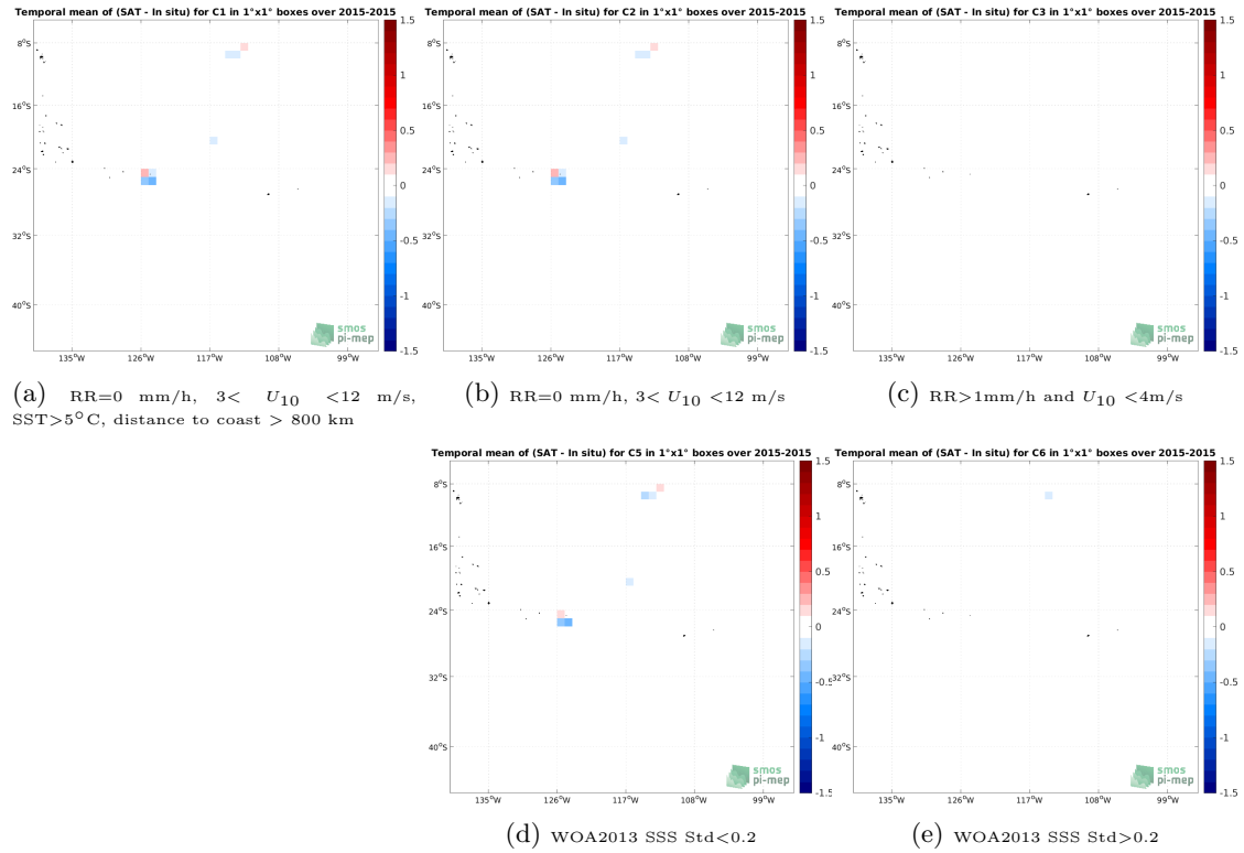
Figure 11: Temporal mean gridded over spatial boxes of size 1^\circ \times 1^\circ of \Delta SSS (Aquarius SSS L3 OR v5 - 7-Day running (NASA-GSFC) - Surface drifters) for 5 different subdatasets corresponding to: RR=0 mm/h, 3 < U_{10} < 12 m/s, SST > 5^\circ\text{C} , distance to coast > 800 km (a), RR=0 mm/h, 3 < U_{10} < 12 m/s (b), RR > 1 mm/h and U_{10} < 4 m/s (c), WOA2013 SSS Std < 0.2 (d), WOA2013 SSS Std > 0.2 (e).
