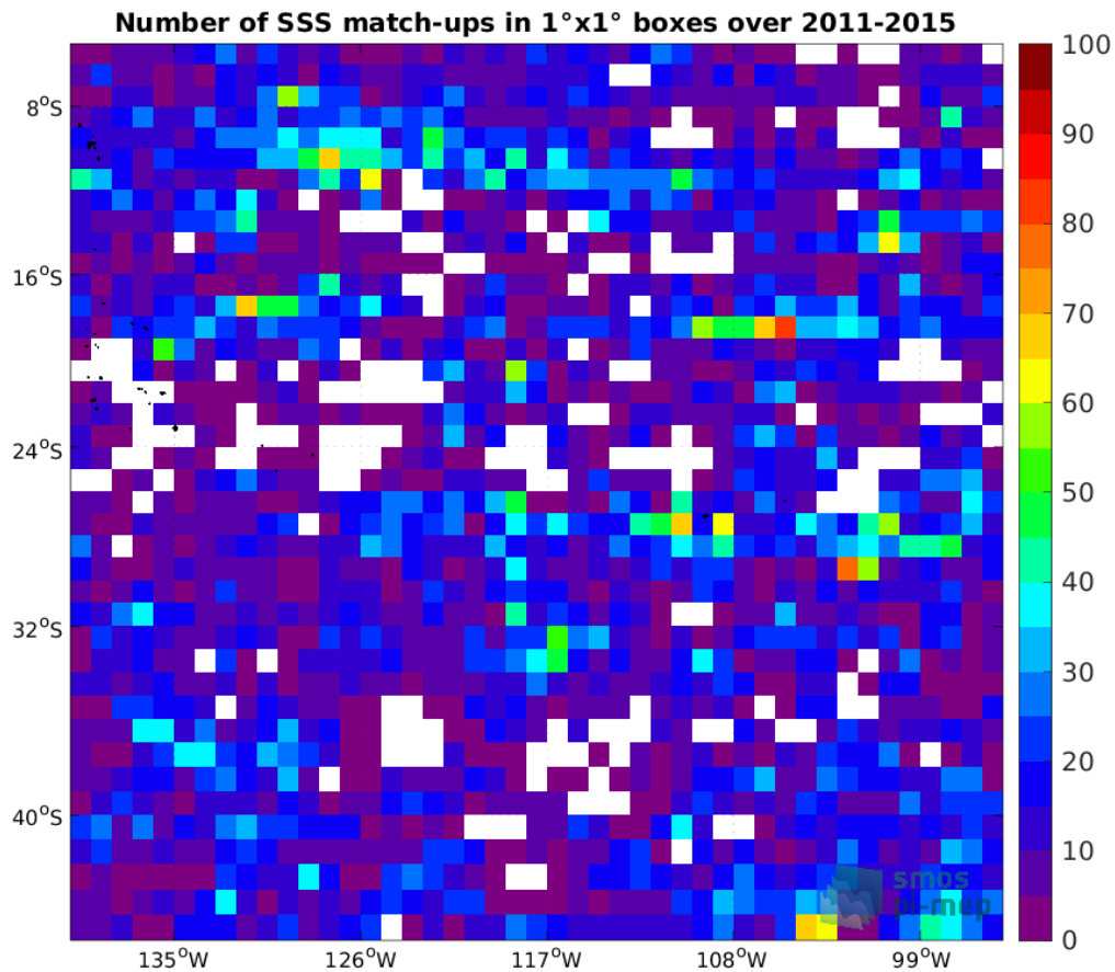
Figure 4: Number of SSS match-ups between Argo SSS and the Aquarius SSS L3 OR v5 - 7-Day running (NASA-GSFC) SSS product for the OTT zone Pi-MEP region over 1°×1° boxes and for the full satellite product period.
