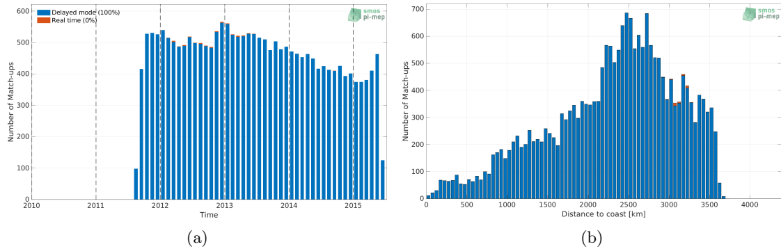
Figure 1: Number of match-ups between Argo and Aquarius SSS L3 OR v5 - 7-Day running (NASA-GSFC) SSS as a function of time (a) and as function of the distance to coast (b) over the OTT zone Pi-MEP region and for the full satellite product period.
