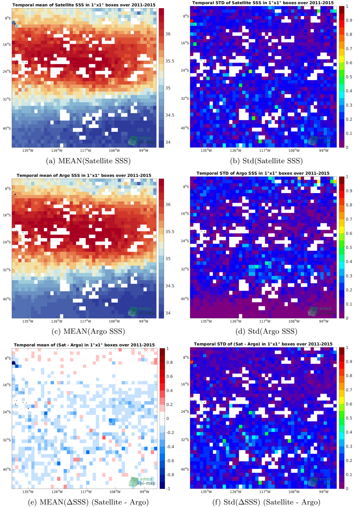
Figure 6: Temporal mean (left) and Std (right) of SSS from Aquarius SSS L3 OR v5 - 7-Day running (NASA-GSFC) (top), Argo (middle), and of \Delta SSS (Satellite - Argo). Only match-up pairs are used to generate these maps.
