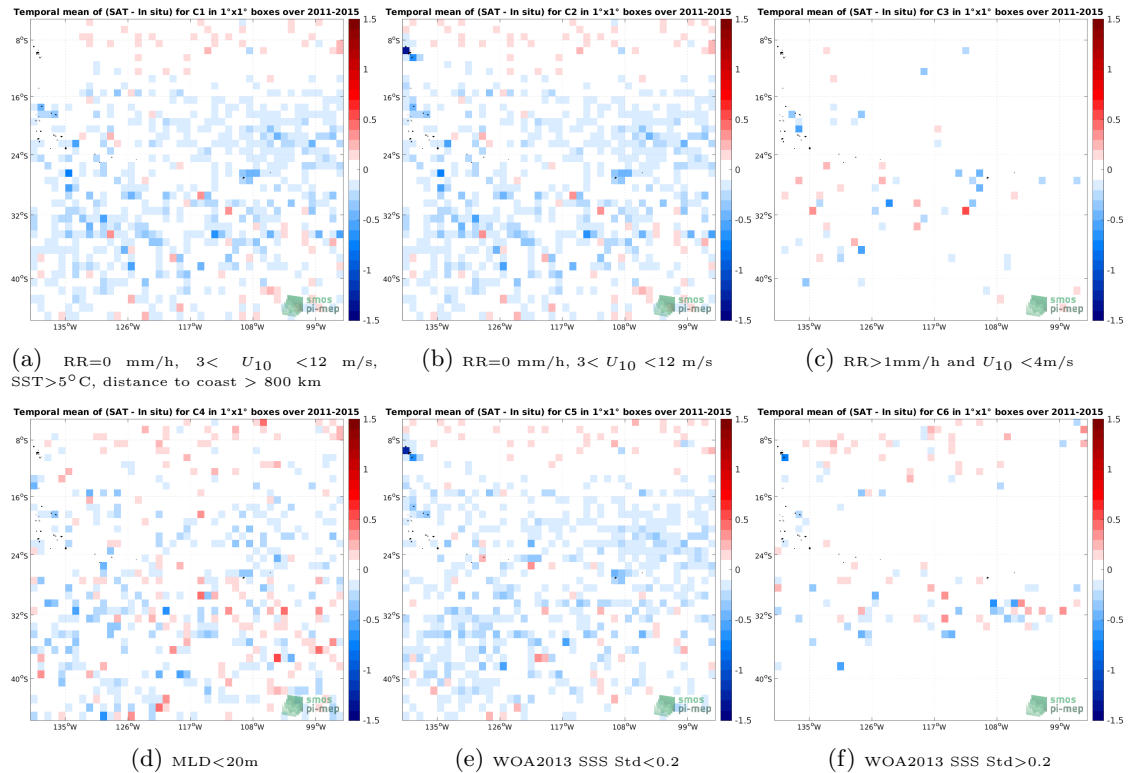
Figure 12: Temporal mean gridded over spatial boxes of size 1^\circ \times 1^\circ of \Delta SSS (Aquarius SSS L3 OR v5 - 7-Day running (NASA-GSFC) - Argo) for 6 different subdatasets corresponding to:RR=0 mm/h, 3 < U_{10} < 12 m/s, SST >5^\circ\text{C} , distance to coast > 800 km (a), RR=0 mm/h, 3 < U_{10} < 12 m/s (b), RR >1 mm/h and U_{10} < 4 m/s (c),MLD <20 m (d),WOA2013 SSS Std <0.2 (e),WOA2013 SSS Std >0.2 (f).
