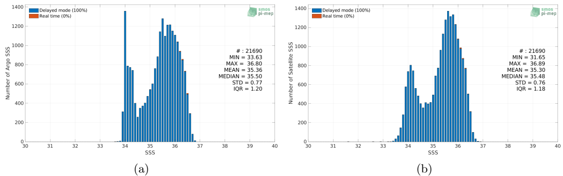
Figure 2: Histograms of SSS from Argo (a) and Aquarius SSS L3 OR v5 - 7-Day running (NASA-GSFC) (b) considering all match-up pairs per bins of 0.1 over the OTT zone Pi-MEP region and for the full satellite product period.
