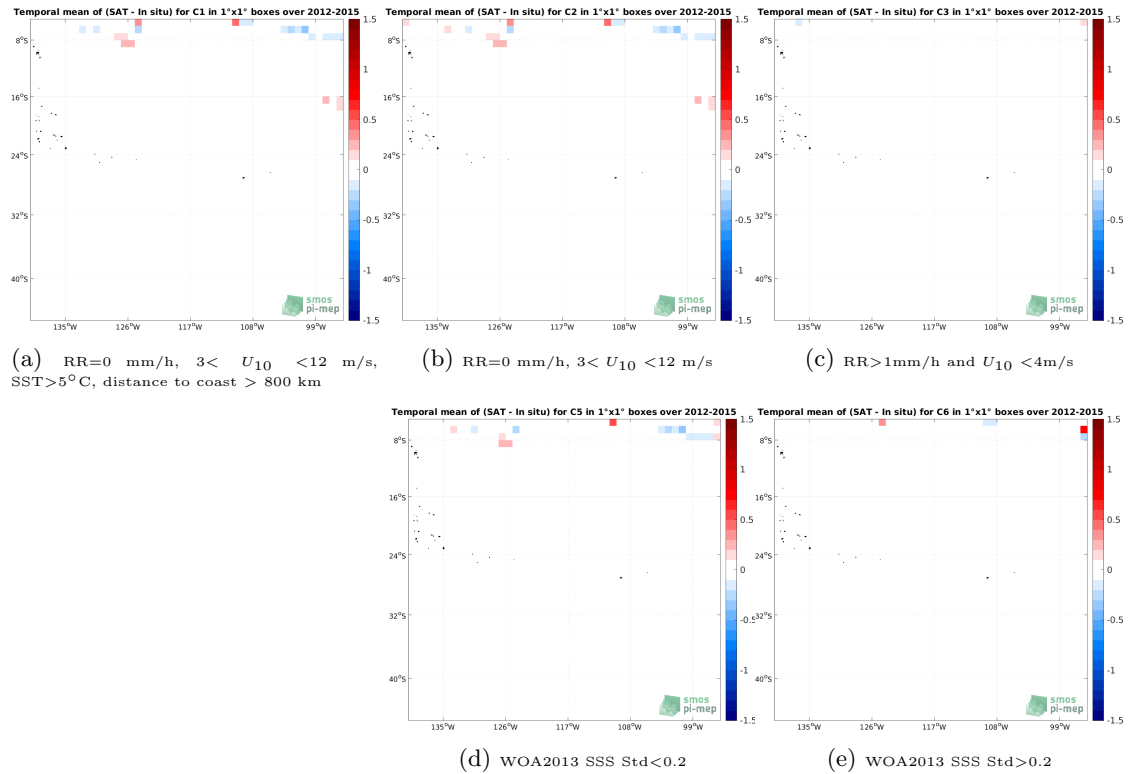
Figure 12: Temporal mean gridded over spatial boxes of size 1^{\circ}\times 1^{\circ} of \Delta\text{SSS} (Aquarius SSS L3 OR v5 - 7-Day running - Rain mask (NASA-GSFC) - TSG (SAMOS)) for 5 different subdatasets corresponding to:RR=0 mm/h, 3 < U_{10} < 12 m/s, SST >5^{\circ}\text{C} , distance to coast > 800 km (a), RR=0 mm/h, 3 < U_{10} < 12 m/s (b), RR >1 mm/h and U_{10} < 4 m/s (c), WOA2013 SSS Std <0.2 (d), WOA2013 SSS Std >0.2 (e).
