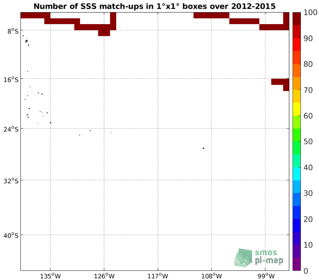
Figure 4: Number of SSS match-ups between TSG (SAMOS) SSS and the Aquarius SSS L3 OR v5 - 7-Day running - Rain mask (NASA-GSFC) SSS product for the OTT zone Pi-MEP region over 1°x1° boxes and for the full satellite product period.
