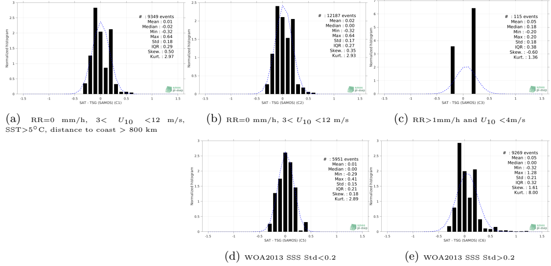
Figure 13: Normalized histogram of \Delta\text{SSS} (Aquarius SSS L3 OR v5 - 7-Day running - Rain mask (NASA-GSFC) - TSG (SAMOS)) for 5 different subdatasets corresponding to: RR=0 mm/h, 3 < U_{10} < 12 m/s, SST>5°C, distance to coast > 800 km (a), RR=0 mm/h, 3 < U_{10} < 12 m/s (b), RR>1mm/h and U_{10} < 4 m/s (c), WOA2013 SSS Std<0.2 (d), WOA2013 SSS Std>0.2 (e).
