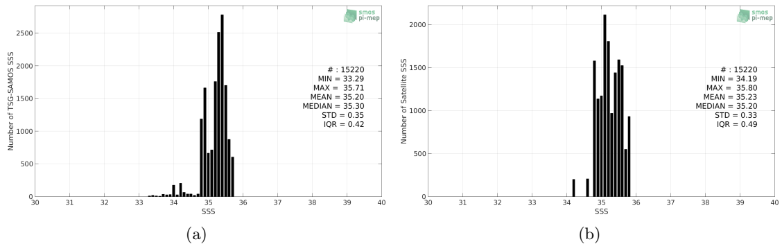
Figure 2: Histograms of SSS from TSG-SAMOS (a) and Aquarius-L3-OR-V5-7DAY-RUNNING-RAIN-MASK-1DEG (b) considering all match-up pairs per bins of 0.1 over the OTT zone Pi-MEP region and for the full satellite product period.
