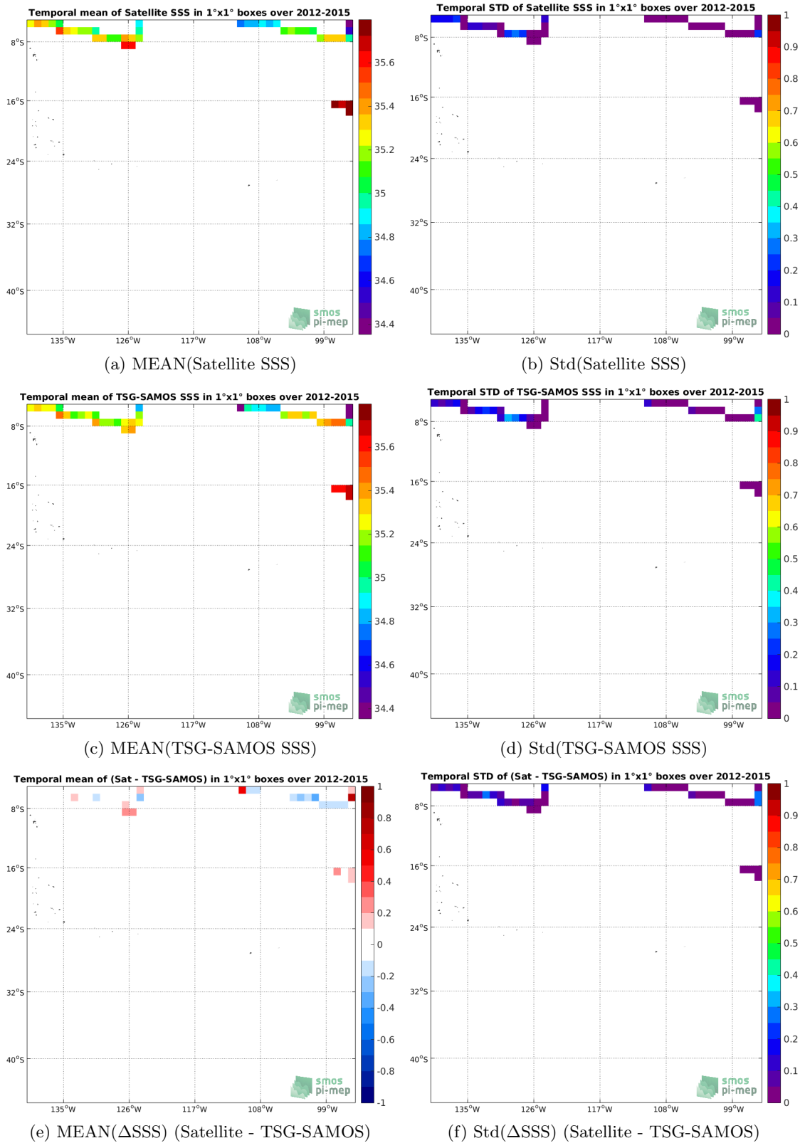
Figure 6: Temporal mean (left) and Std (right) of SSS from Aquarius-L3-OR-V5-7DAY-RUNNING-RAIN-MASK-1DEG (top), TSG-SAMOS (middle), and of \Delta SSS (Satellite - TSG-SAMOS). Only match-up pairs are used to generate these maps.
