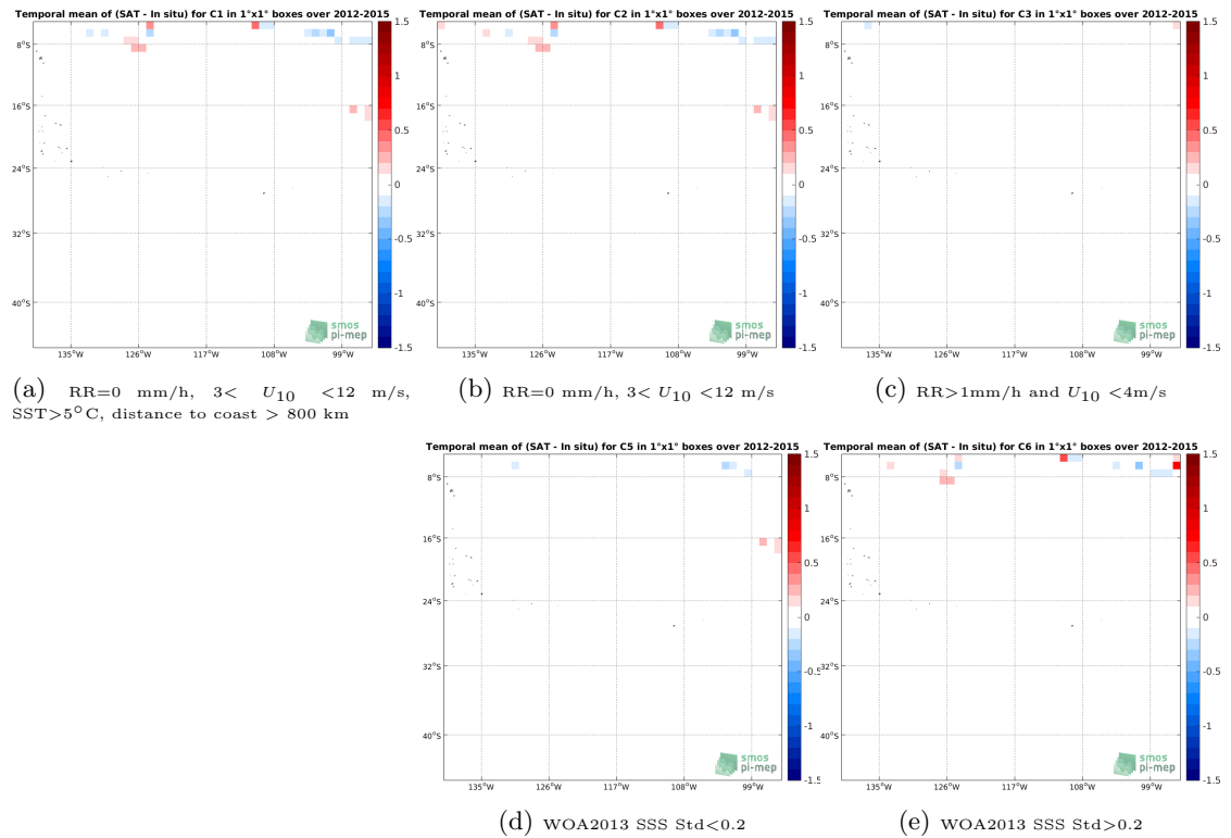
Figure 12: Temporal mean gridded over spatial boxes of size 1^\circ \times 1^\circ of \Delta SSS (Aquarius-L3-OR-V5-7DAY-RUNNING-RAIN-MASK-1DEG - TSG-SAMOS) for 5 different subdatasets corresponding to:RR=0 mm/h, 3 < U_{10} < 12 m/s, SST >5^\circ C, distance to coast > 800 km (a), RR=0 mm/h, 3 < U_{10} < 12 m/s (b), RR >1 mm/h and U_{10} < 4 m/s (c), WOA2013 SSS Std <0.2 (d), WOA2013 SSS Std >0.2 (e).
