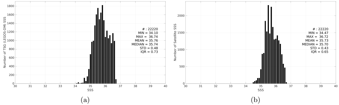
Figure 3: Histograms of SSS from TSG (LEGOS-DM) (a) and Aquarius SSS L3 OR v5 - 7-Day running - Rain mask (NASA-GSFC) (b) considering all match-up pairs per bins of 0.1 over the OTT zone Pi-MEP region and for the full satellite product period.
