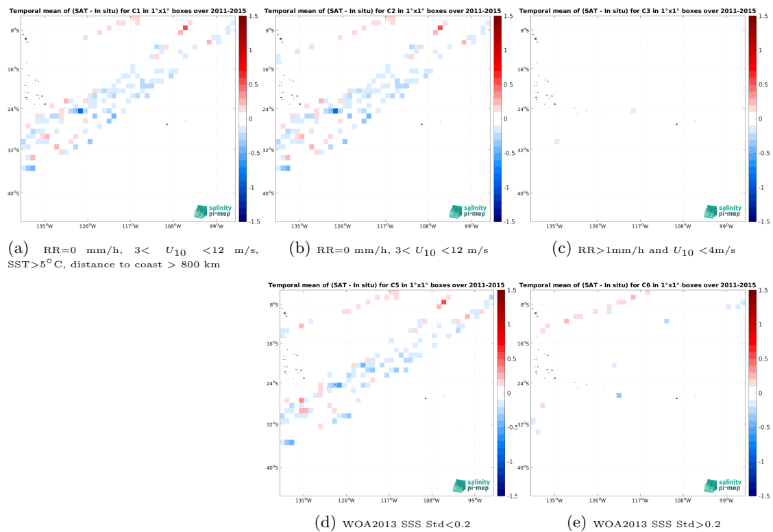
Figure 14: Temporal mean gridded over spatial boxes of size 1^\circ \times 1^\circ of \Delta SSS (Aquarius SSS L3 OR v5 - 7-Day running - Rain mask (NASA-GSFC) - TSG (LEGOS-DM)) for 5 different subdatasets corresponding to:RR=0 mm/h, 3 < U_{10} < 12 m/s, SST >5^\circ\text{C} , distance to coast > 800 km (a), RR=0 mm/h, 3 < U_{10} < 12 m/s (b), RR >1 mm/h and U_{10} < 4 m/s (c), WOA2013 SSS Std <0.2 (d), WOA2013 SSS Std >0.2 (e).
