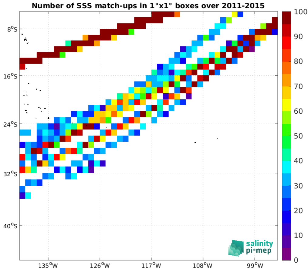
Figure 5: Number of SSS match-ups between TSG (LEGOS-DM) SSS and the Aquarius SSS L3 OR v5 - 7-Day running - Rain mask (NASA-GSFC) SSS product for the OTT zone Pi-MEP region over 1^\circ \times 1^\circ boxes and for the full satellite product period.
