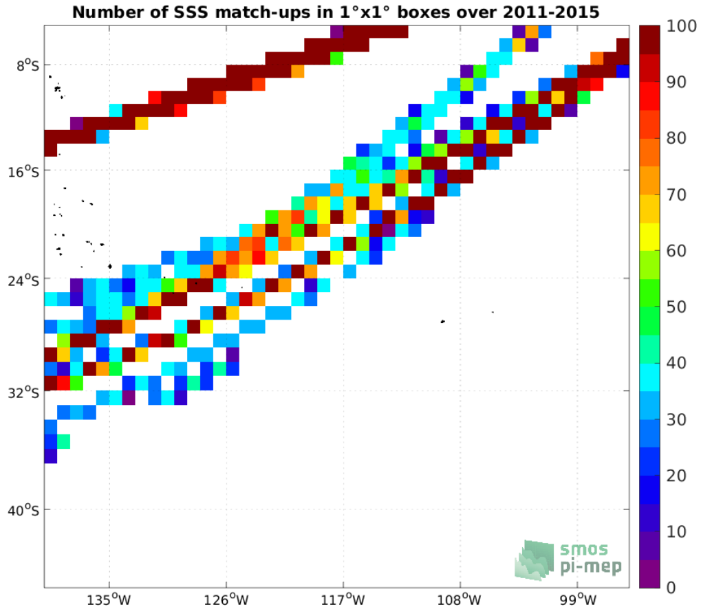
Figure 4: Number of SSS match-ups between TSG (LEGOS-DM) SSS and the Aquarius SSS L3 OR v5 - 7-Day running - Rain mask (NASA-GSFC) SSS product for the OTT zone Pi-MEP region over 1°x1° boxes and for the full satellite product period.
