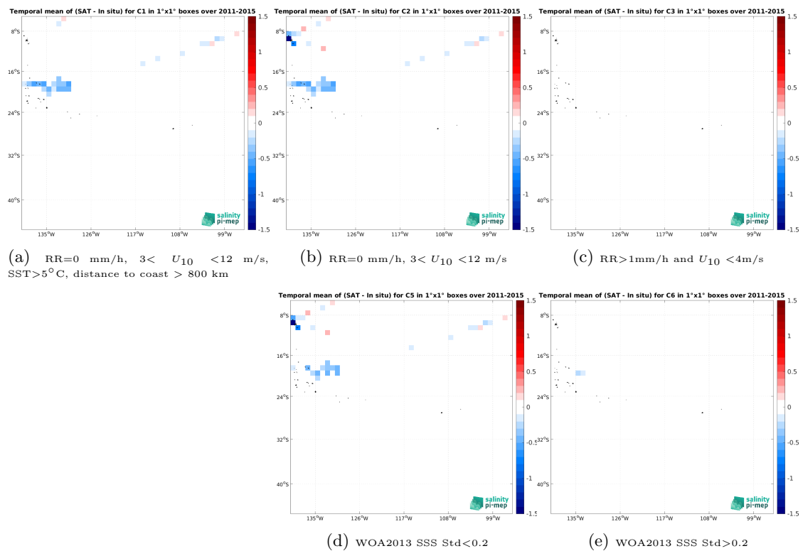
Figure 14: Temporal mean gridded over spatial boxes of size 1^\circ \times 1^\circ of \Delta SSS (Aquarius SSS L3 OR v5 - 7-Day running - Rain mask (NASA-GSFC) - TSG (GOSUD-Research-vessel)) for 5 different subdatasets corresponding to:RR=0 mm/h, 3 < U_{10} < 12 m/s, SST >5^\circ\text{C} , distance to coast > 800 km (a), RR=0 mm/h, 3 < U_{10} < 12 m/s (b), RR >1 mm/h and U_{10} < 4 m/s (c), WOA2013 SSS Std <0.2 (d), WOA2013 SSS Std >0.2 (e).
