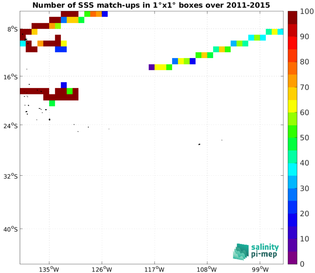
Figure 5: Number of SSS match-ups between TSG (GOSUD-Research-vessel) SSS and the Aquarius SSS L3 OR v5 - 7-Day running - Rain mask (NASA-GSFC) SSS product for the OTT zone Pi-MEP region over 1^\circ \times 1^\circ boxes and for the full satellite product period.
