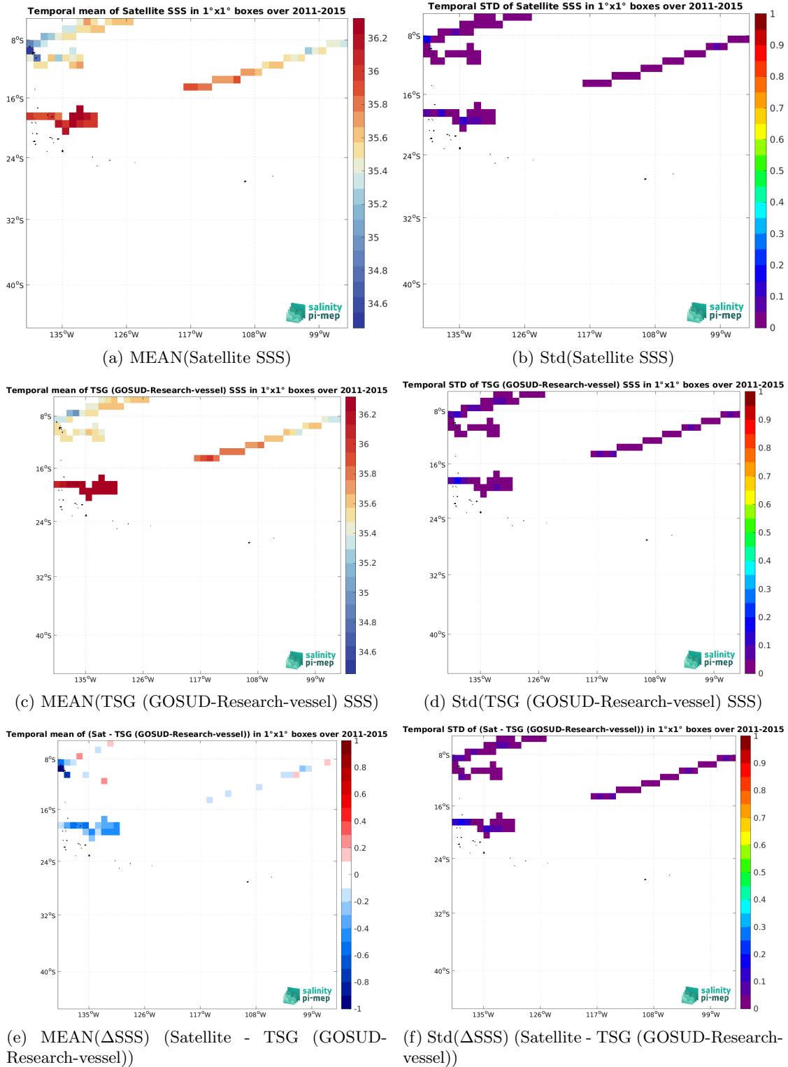
Figure 7: Temporal mean (left) and Std (right) of SSS from Aquarius SSS L3 OR v5 - 7-Day running - Rain mask (NASA-GSFC) (top), TSG (GOSUD-Research-vessel) (middle), and of \Delta SSS (Satellite - TSG (GOSUD-Research-vessel)). Only match-up pairs are used to generate these maps.
