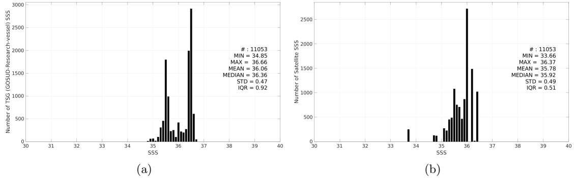
Figure 3: Histograms of SSS from TSG (GOSUD-Research-vessel) (a) and Aquarius SSS L3 OR v5 - 7-Day running - Rain mask (NASA-GSFC) (b) considering all match-up pairs per bins of 0.1 over the OTT zone Pi-MEP region and for the full satellite product period.
